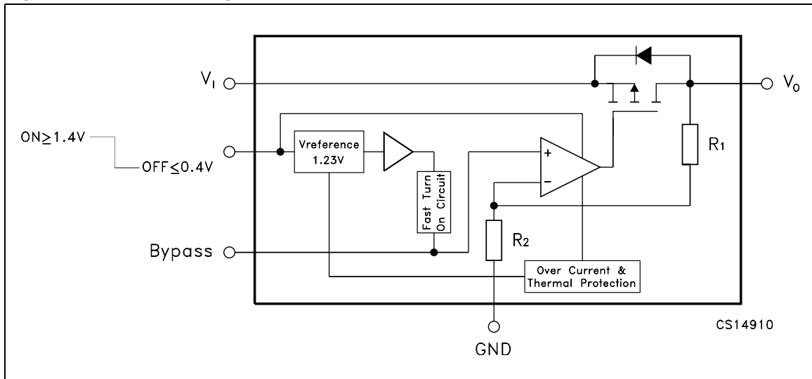
Figure 1. Schematic diagram
