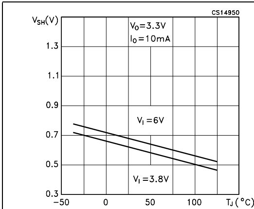
Figure 8. Shutdown voltage vs. temperature
