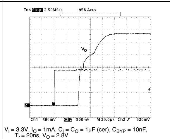
Figure 21. Start-Up
