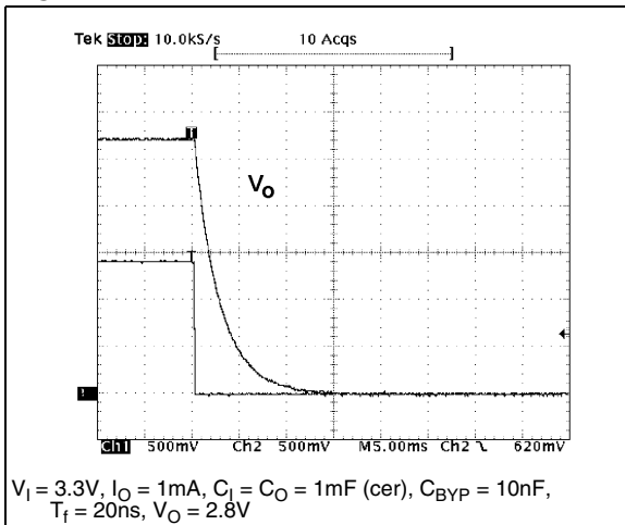
Figure 22. Turn-Off
