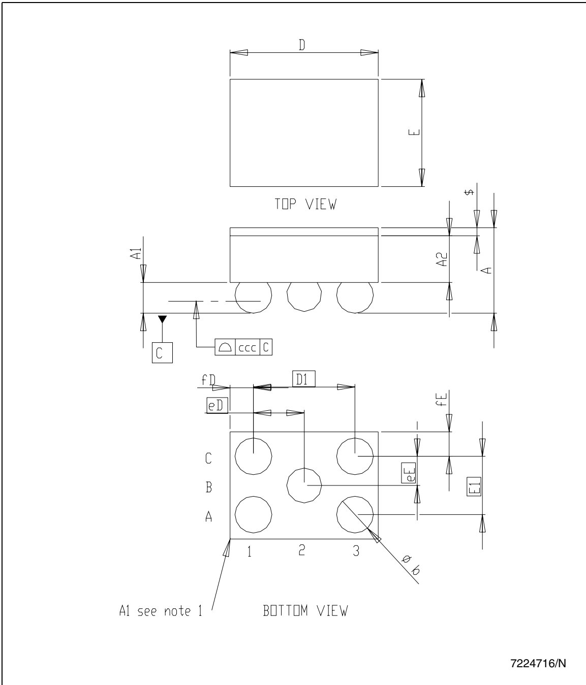
Figure 23. Drawing dimension Flip-chip 5
