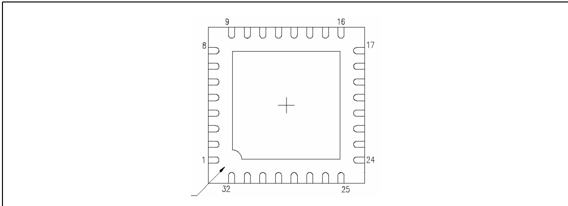
Figure 2. Pin connections (bottom view)
