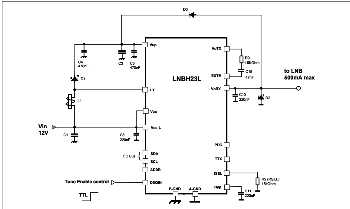
Figure 3. DiSEqC 1.x using internal 22 kHz tone generator
