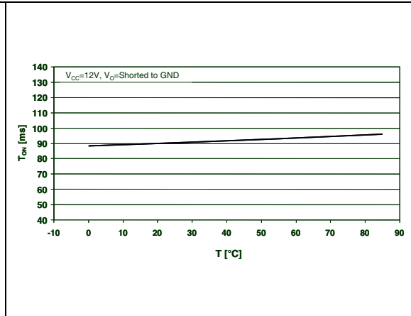
Figure 15. Dynamic overload protection ON time vs. temperature
