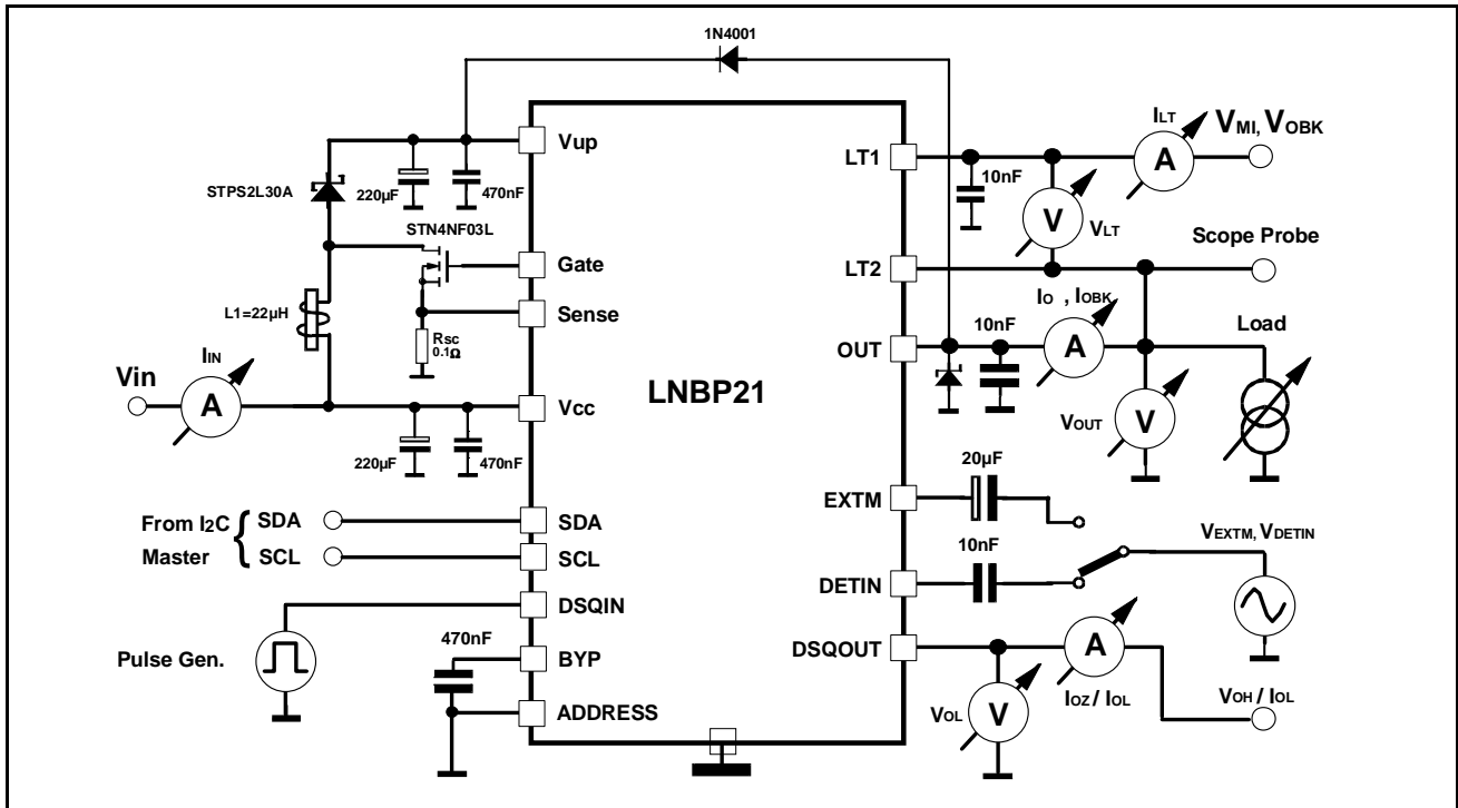
Figure 7: Test Circuit
