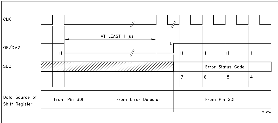
Figure 18. Detection diagram
