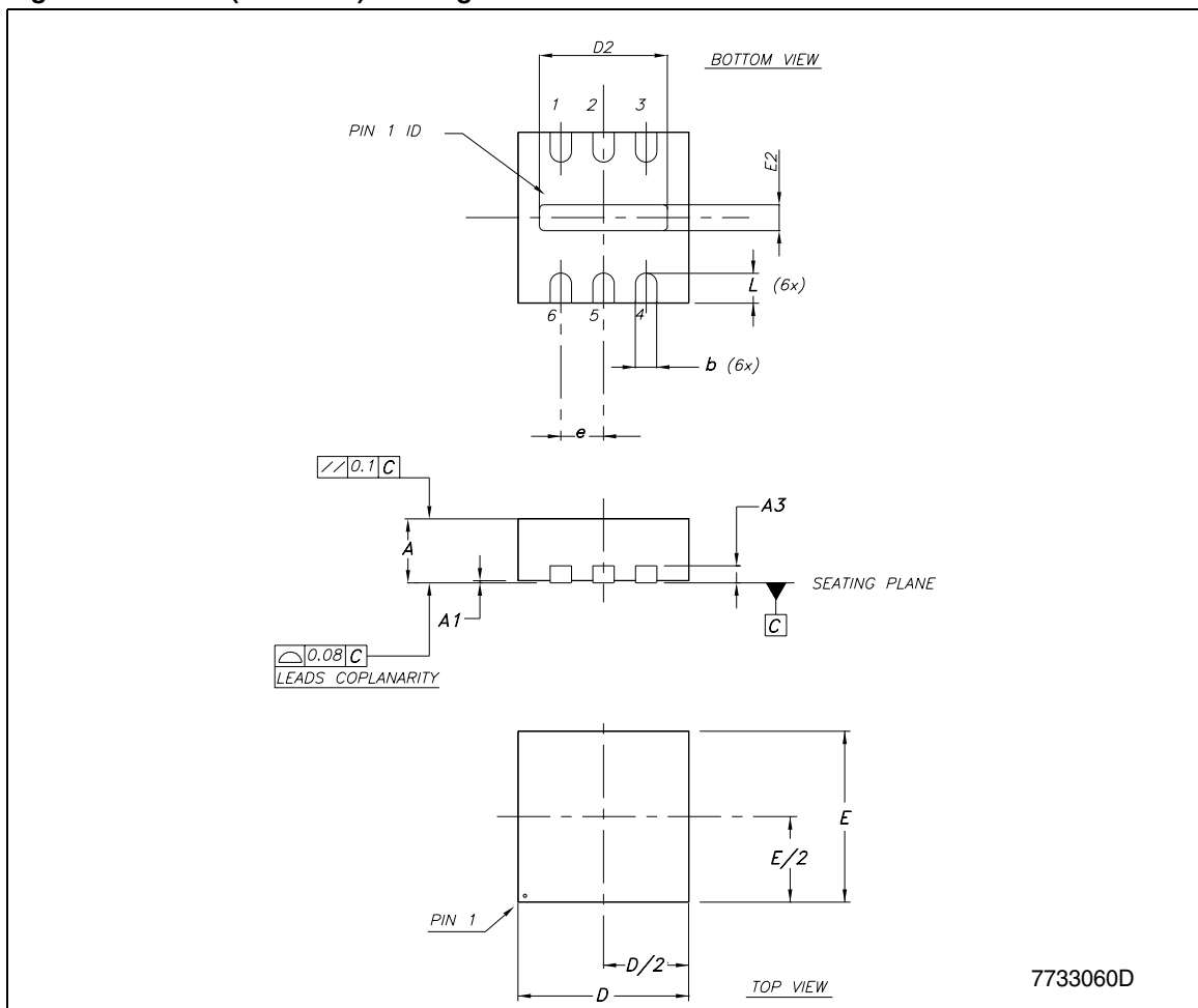
Figure 21. DFN6 (2 x 2 mm.) drawing
