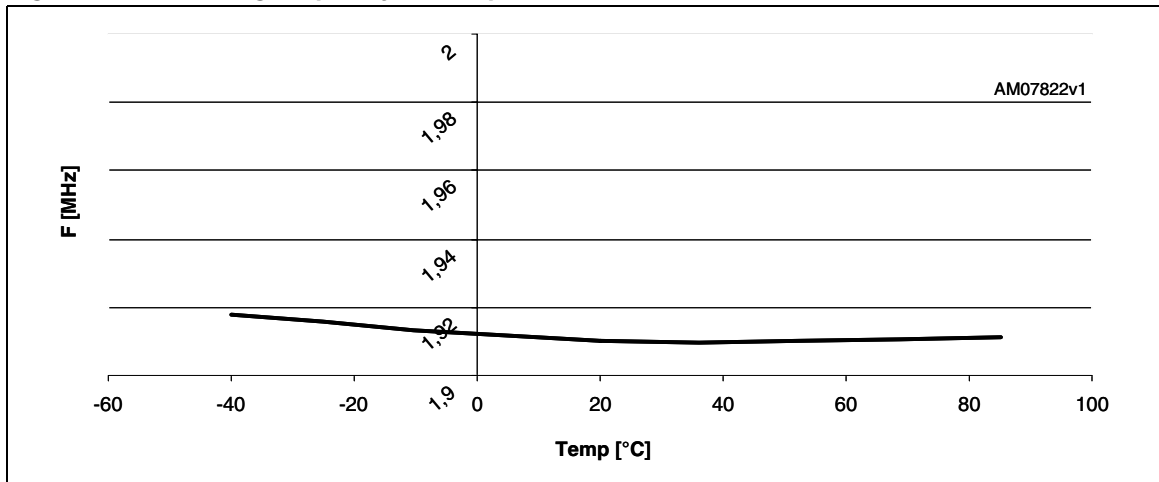
Figure 7. Switching frequency vs. temperature
