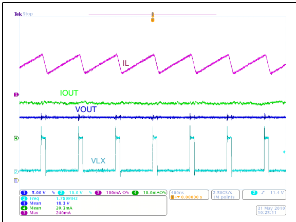
Figure 14. Switching waveform at V_{IN} = 12\text{ V}
