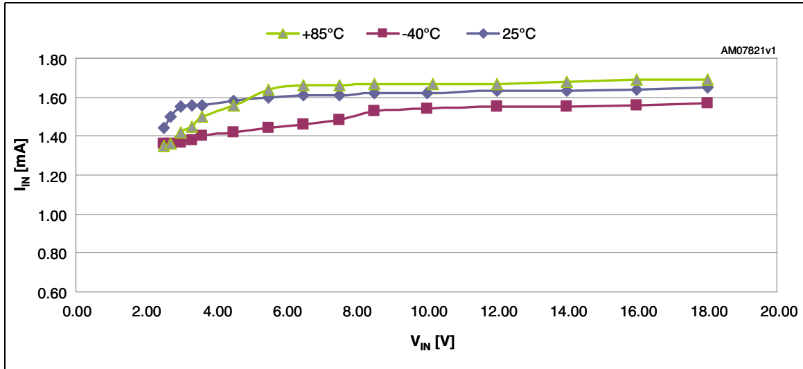
Figure 6. STLA02 driver current consumption vs. V_{IN}
