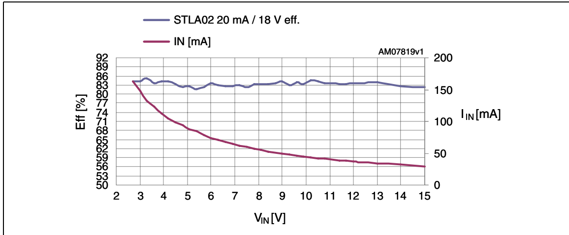
Figure 4. Efficiency at 20 mA current load
