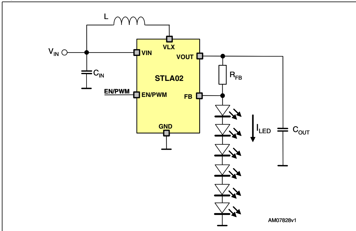
Figure 3. Application schematic
