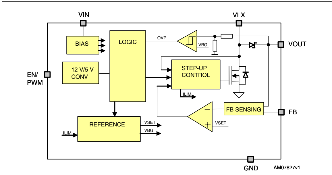
Figure 1. Block diagram
