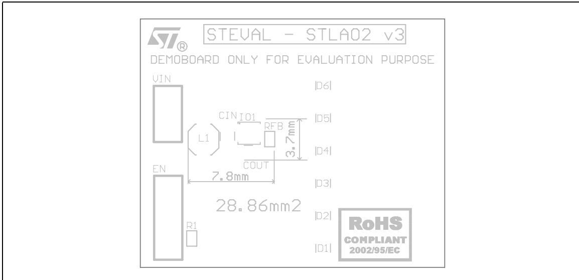
Figure 20. Top overlay
