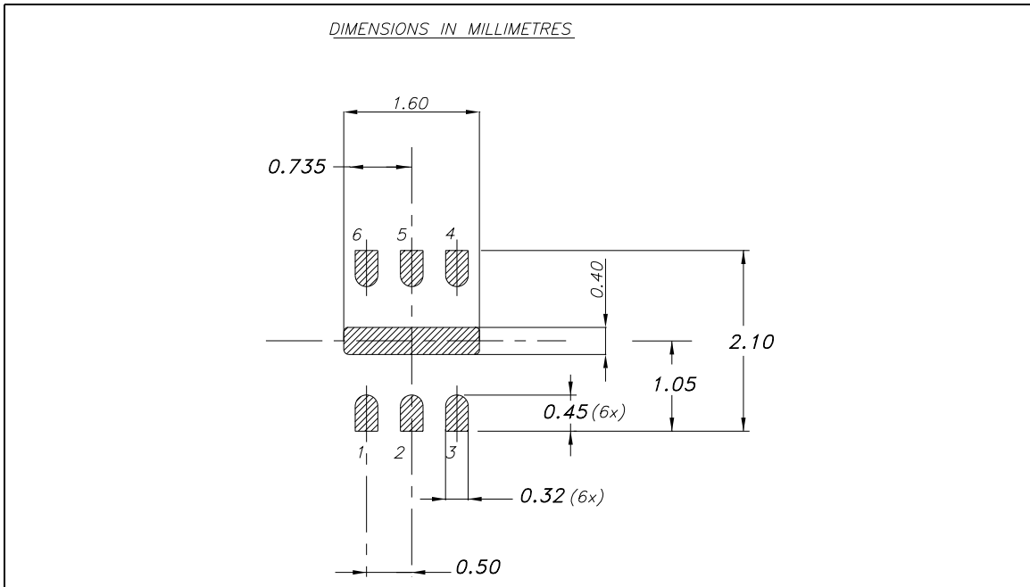
Figure 23. DFN6 (2 x 2 mm) footprint recommended data
