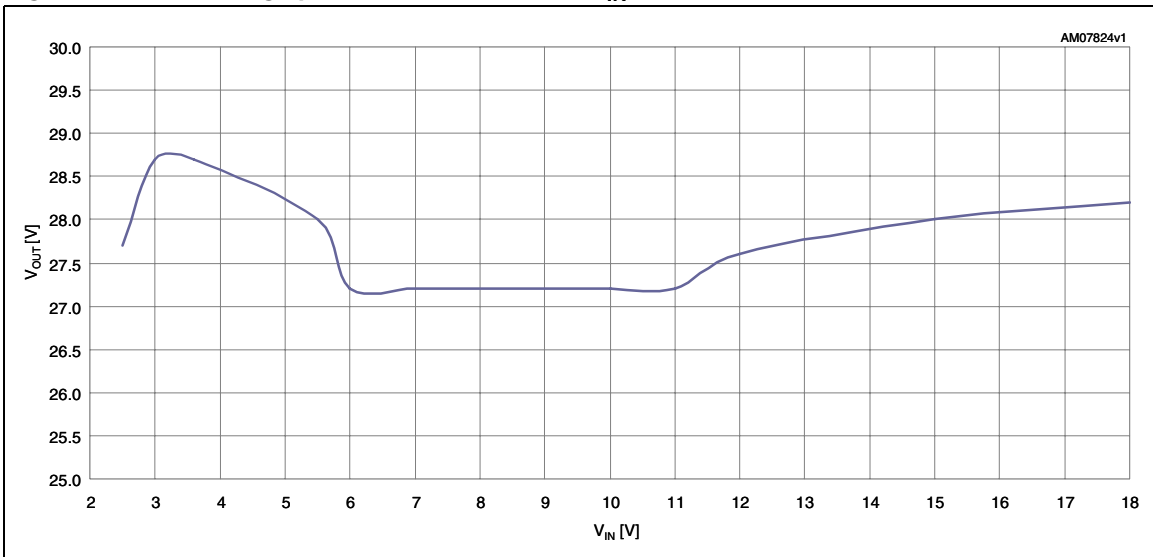
Figure 9. Overvoltage protection threshold vs. V_{IN}
