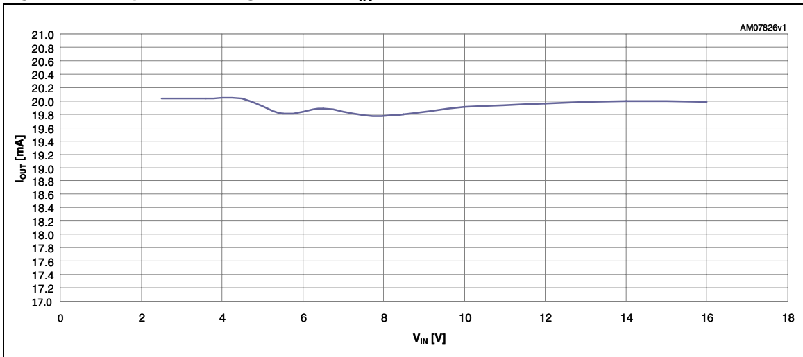
Figure 11. Output current regulation vs. V_{IN}
