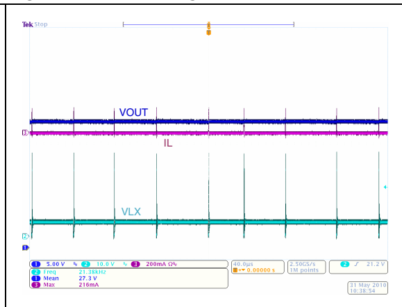
Figure 15. Overvoltage function
