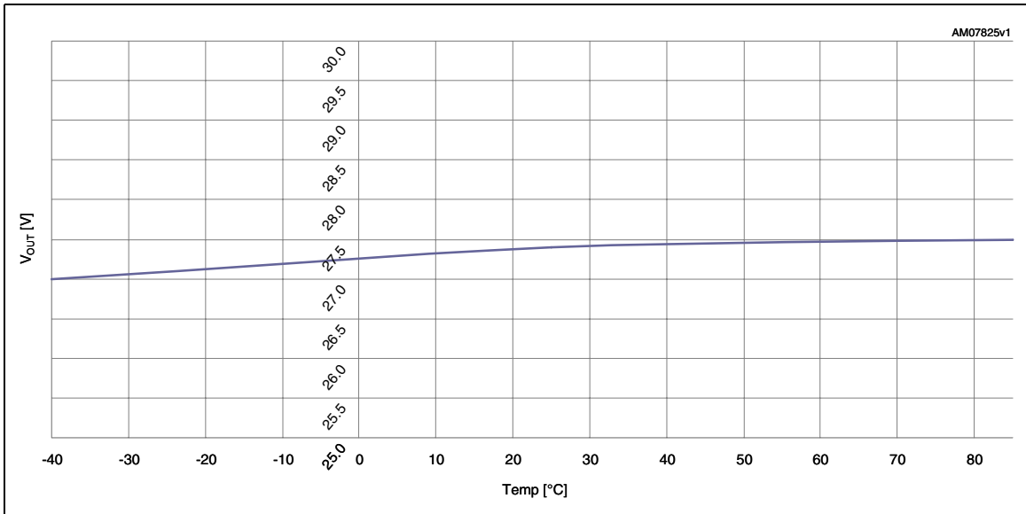
Figure 10. Overvoltage protection threshold vs. temp
