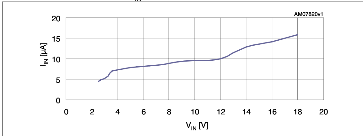
Figure 5. Quiescent current vs. V_{IN}
