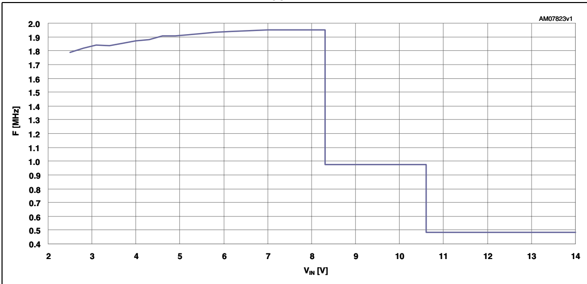
Figure 8. Switching frequency vs. V_{IN} @ P_{OUT} = 0.36\text{ W}
