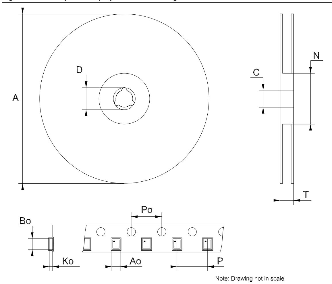
Figure 22. DFN6 (2 x 2 mm.) tape and reel drawing
