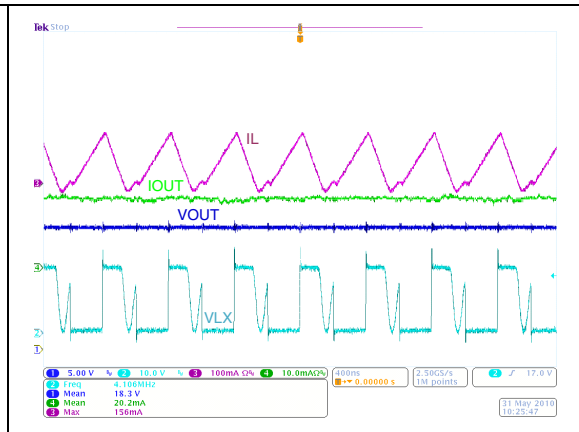
Figure 15. Overvoltage function
