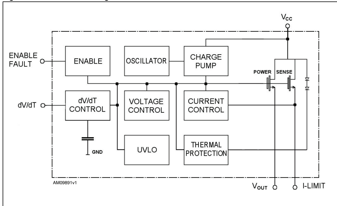
Figure 1. STEF05 block diagram
