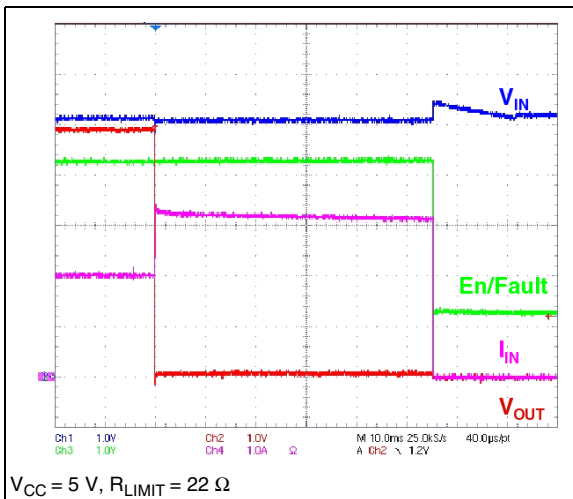
Figure 19. Thermal latch from 2 A load to short-circuit
