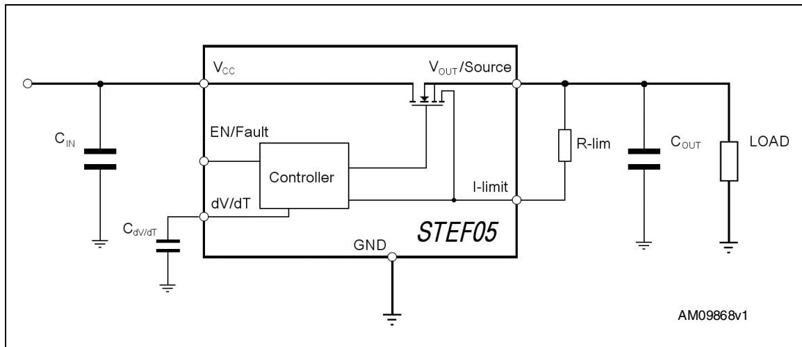
Figure 3. Application circuit
