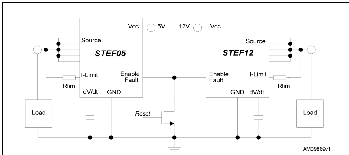
Figure 4. Typical HDD application circuit
