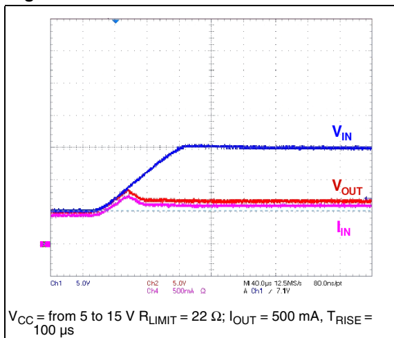
Figure 17. Line transient
