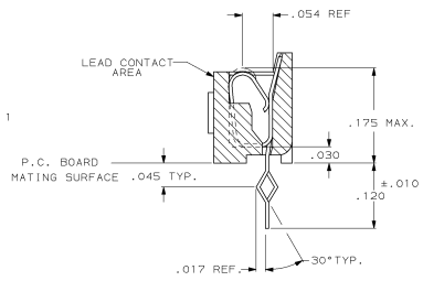
SECTION A-A ROTATED 90° CW SCALE 10:1 FOR -6, -7 & -8 ONLY
