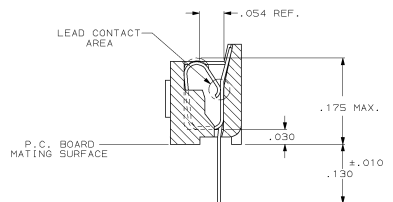
SECTION A-A ROTATED 90° CW SCALE 10:1 FOR -1, -2 & -3 ONLY
