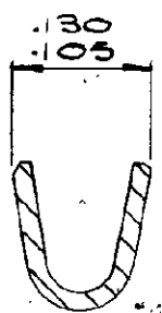
SECTION AA SCALE 6:1
