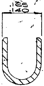
SECTION B-B SCALE 6:1
