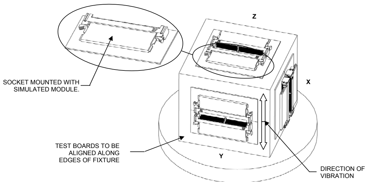
Figure 1 Vibration & Mechanical Shock Mounting Fixture
