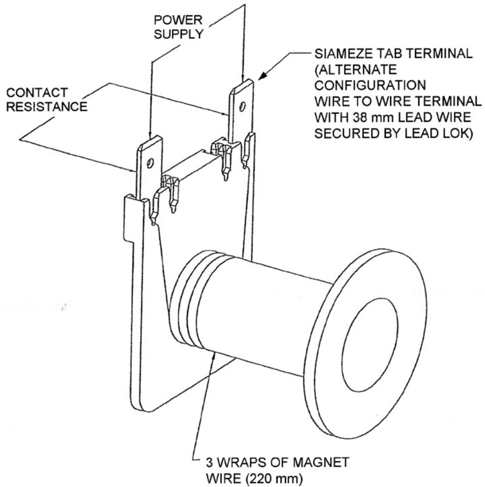
Figure 3 Test Configuration
