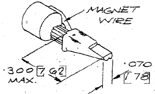
CRIMPED VIEW.
