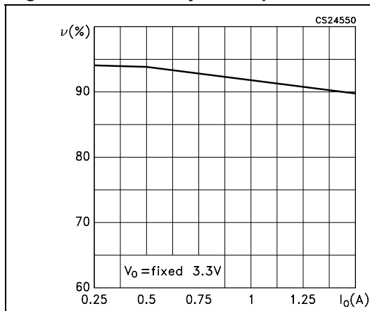
Figure 7. Efficiency vs. output current
