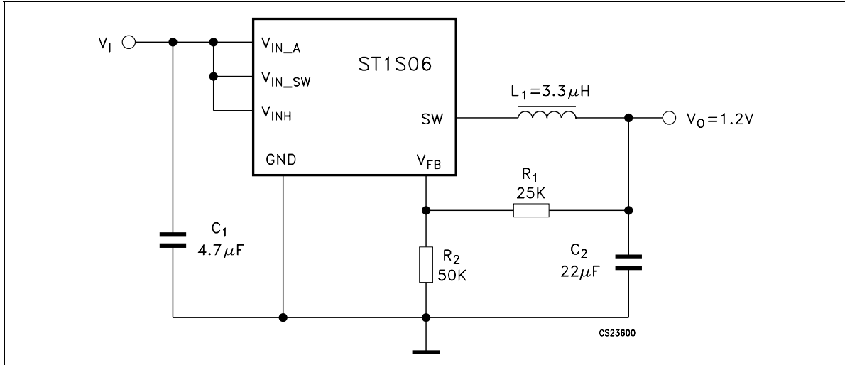
Figure 24. Application circuit
