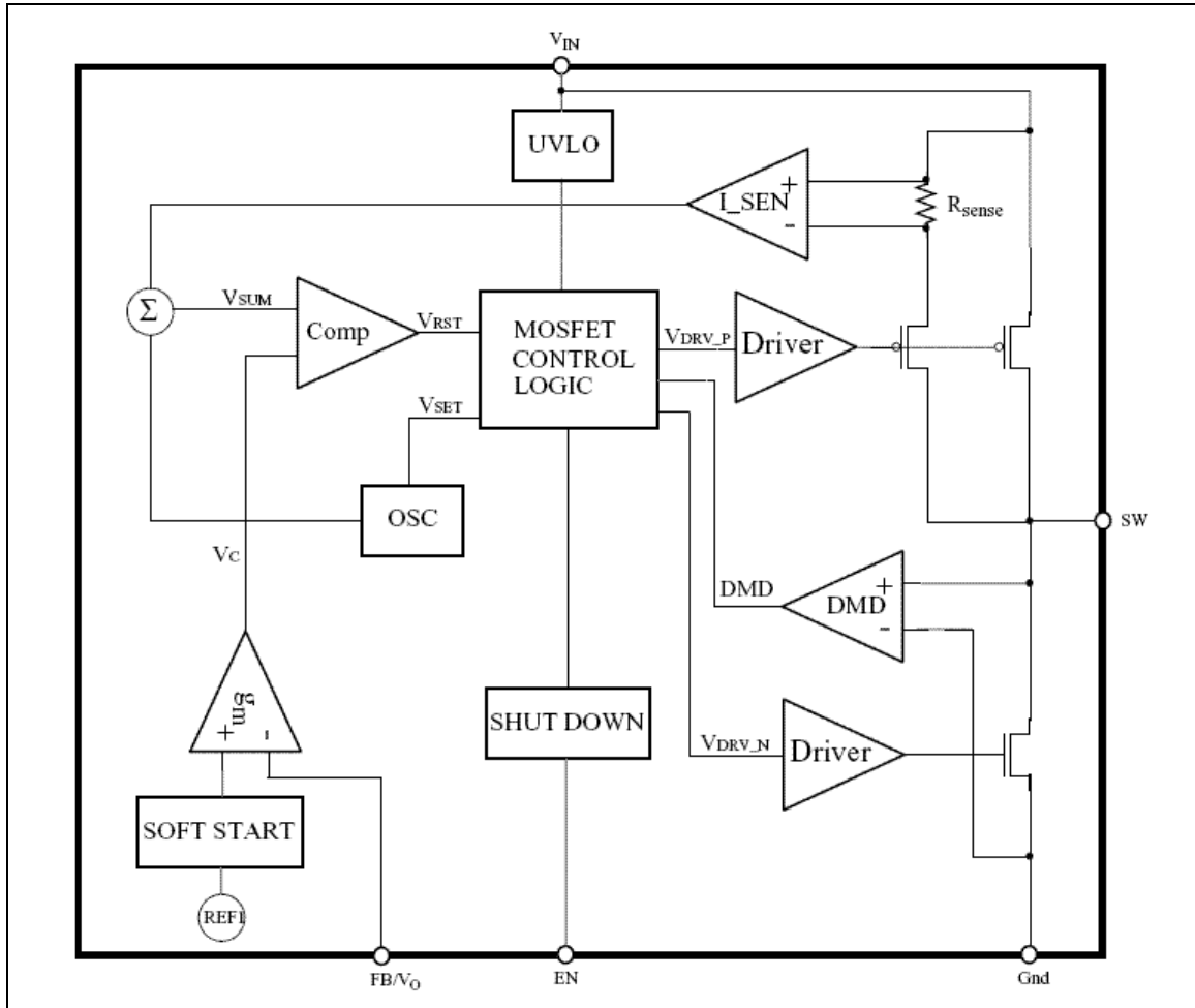
Figure 1. Schematic diagram
