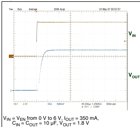
Figure 24. Start-up transient
