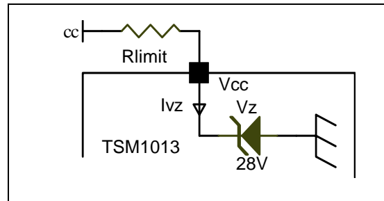
Fig. 4: Clamp voltage
