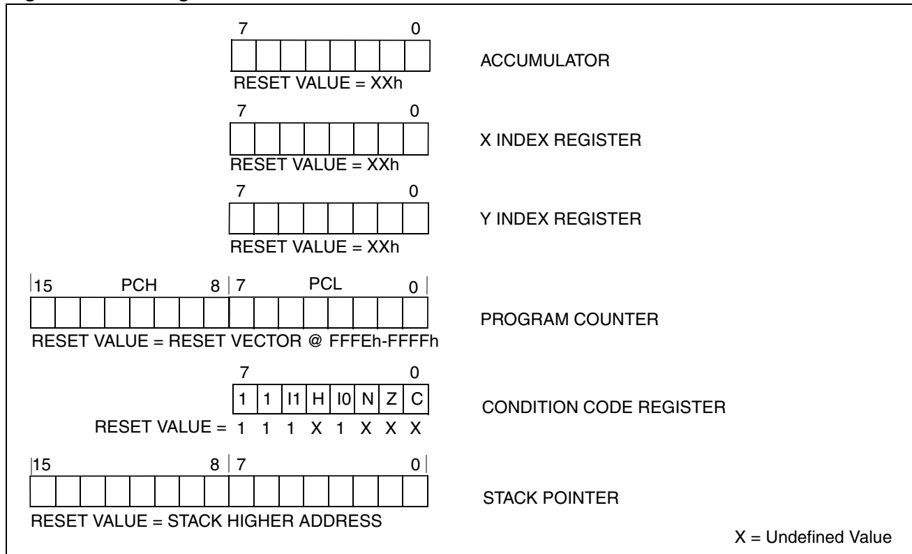
Figure 13. CPU Registers
