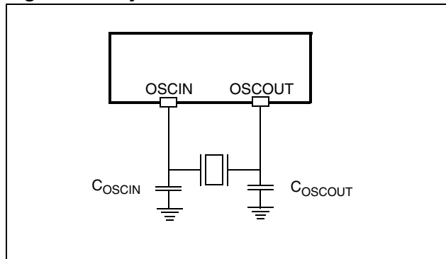
Figure 16. Crystal Resonator
