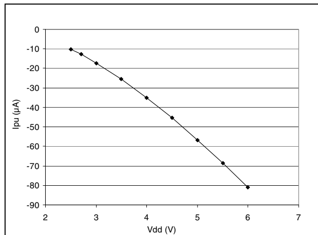
Figure 77. Typical I_{PU} vs. V_{DD} with V_{IN}=V_{SS}
