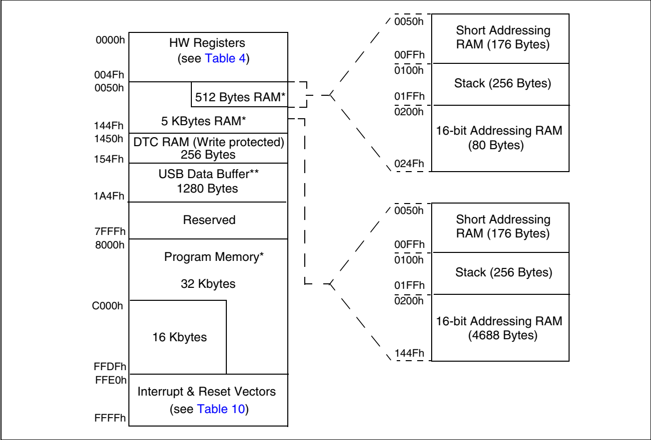
Figure 10. Memory Map
