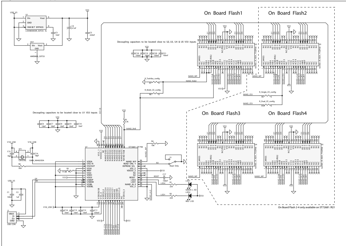
Figure 3. Application schematic
