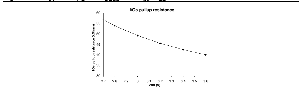
Figure 9. Typical R_{PU} vs. V_{DD33} with V_{IN}=V_{SS}
