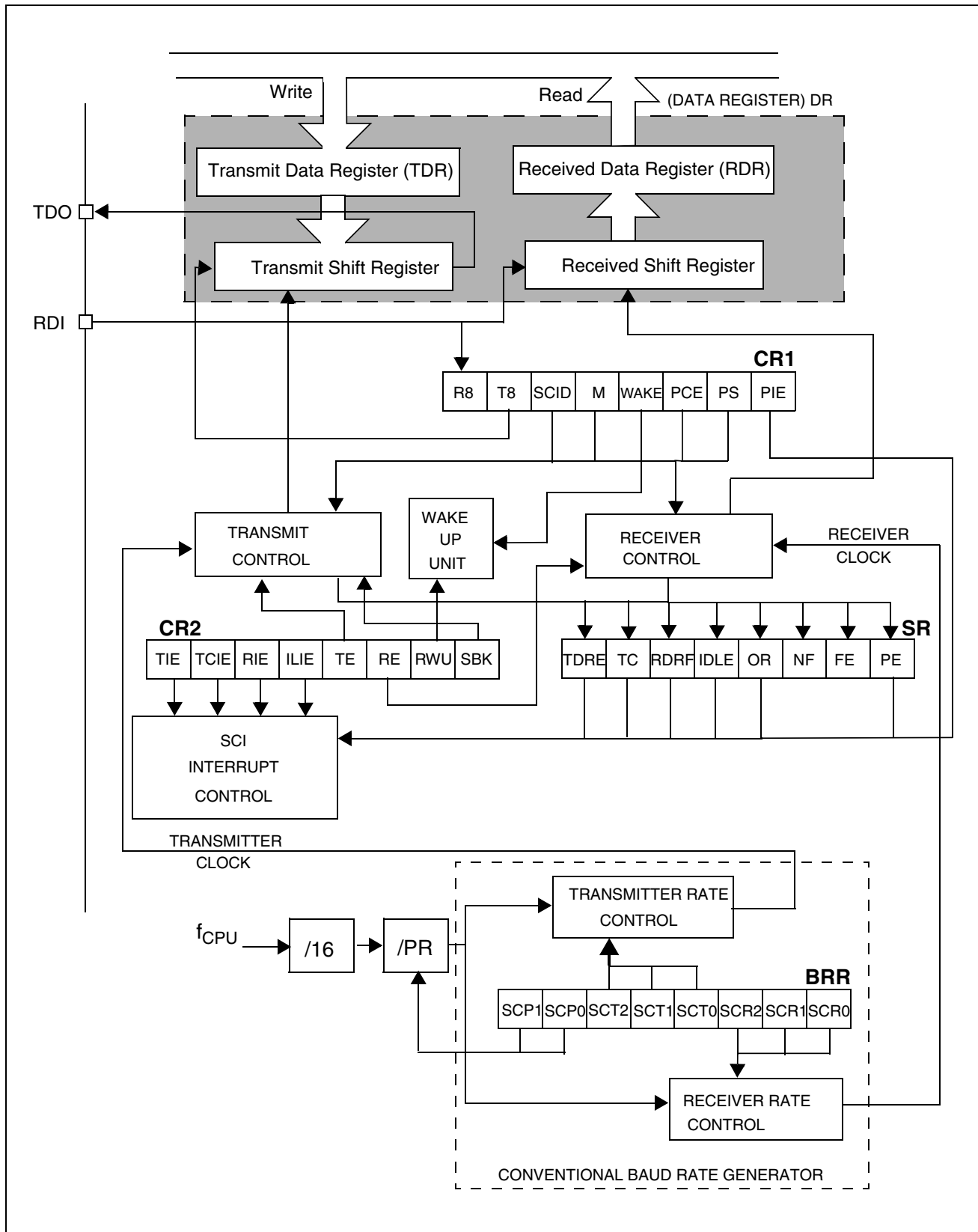
Figure 57. SCI Block Diagram
