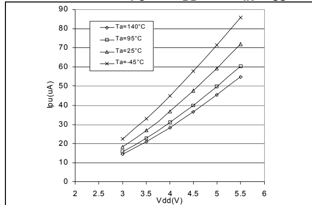
Figure 77. Typical I_{PU} vs. V_{DD} with V_{IN}=V_{SS}
