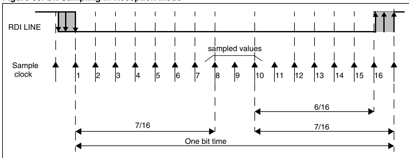
Figure 60. Bit Sampling in Reception Mode
