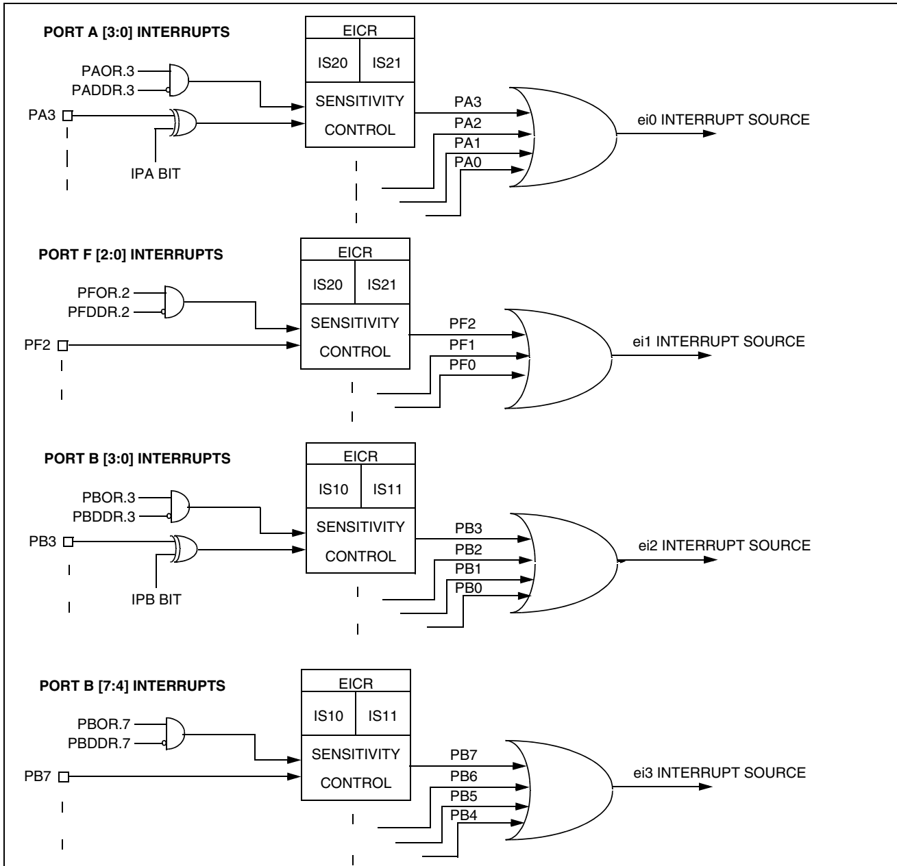
Figure 21. External Interrupt Control bits
