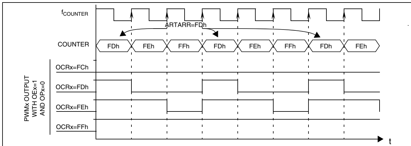
Figure 36. PWM Signal from 0% to 100% Duty Cycle
