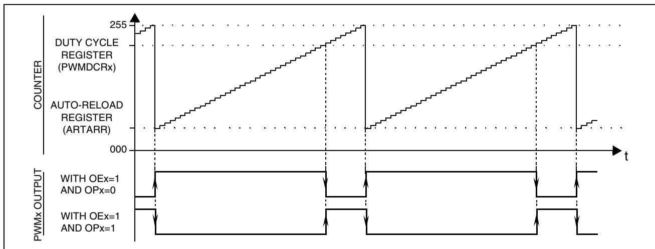
Figure 35. PWM Auto-reload Timer Function
