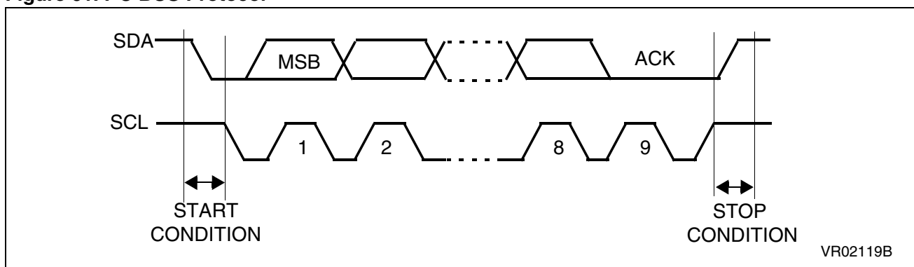
Figure 61. I 2 C BUS Protocol
