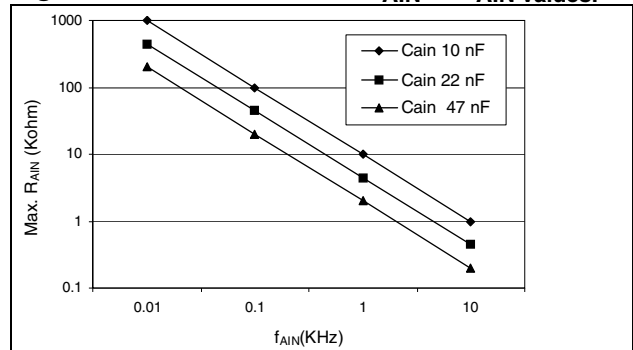
Figure 92. Recommended C_{AIN} & R_{AIN} values. 2)
