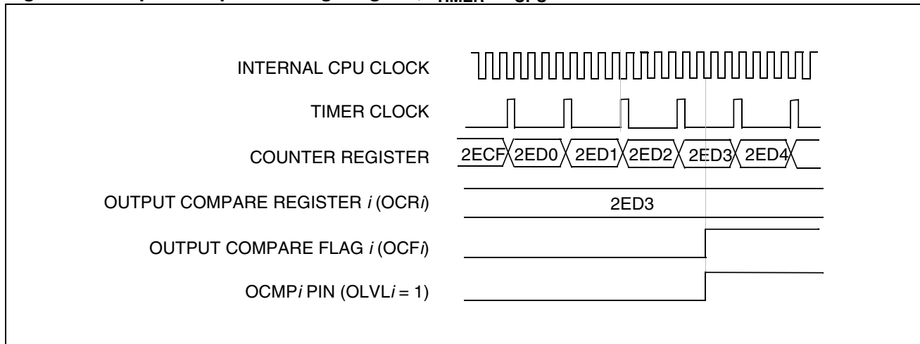
Figure 47. Output Compare Timing Diagram, f_{\text{TIMER}} = f_{\text{CPU}}/4
