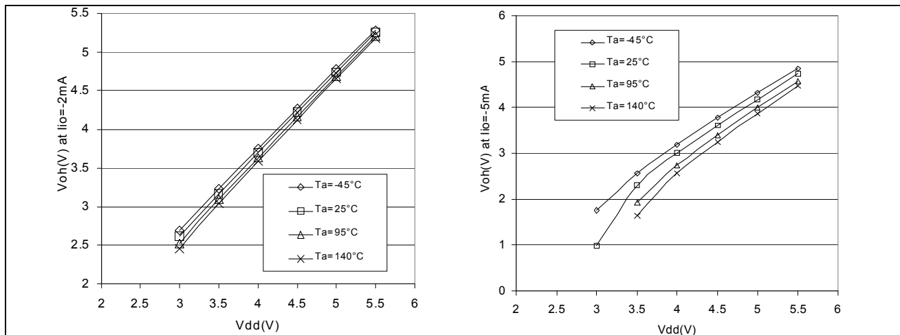
Figure 83. Typical V_{DD}-V_{OH} vs. V_{DD}
