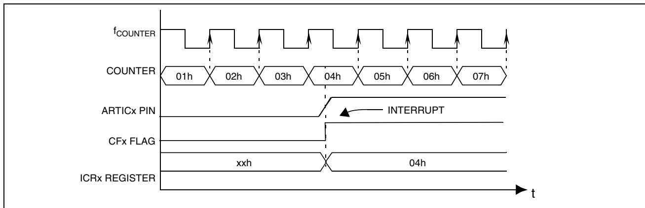
Figure 38. Input Capture Timing Diagram
