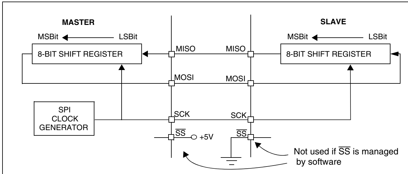
Figure 51. Single Master/ Single Slave Application
