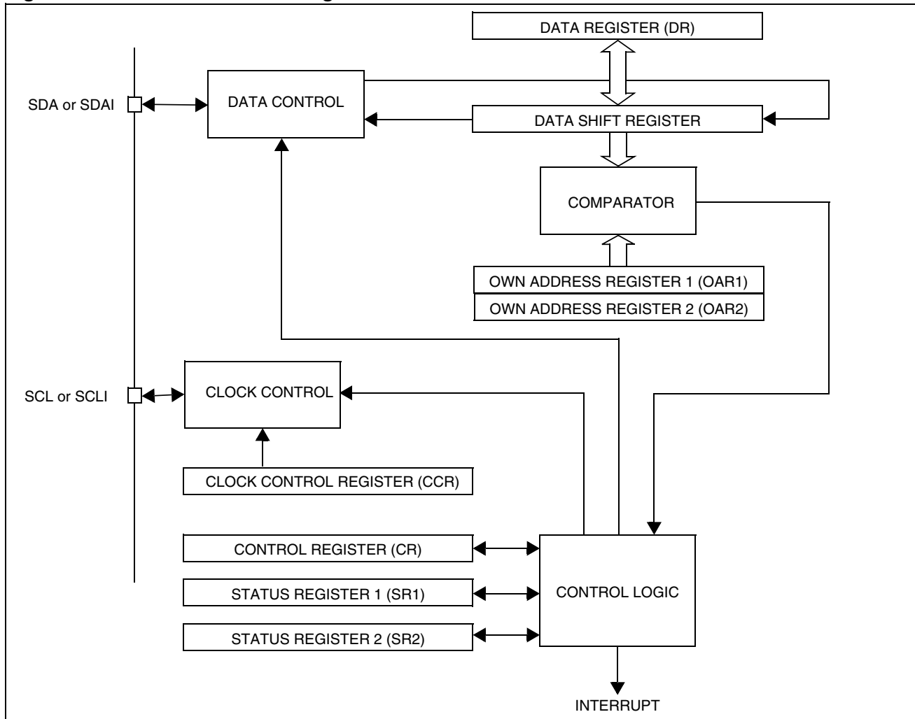
Figure 62. I 2 C Interface Block Diagram
