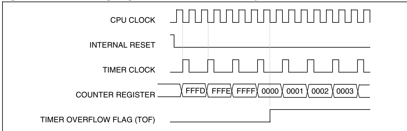
Figure 40. Counter Timing Diagram, Internal Clock Divided by 2
