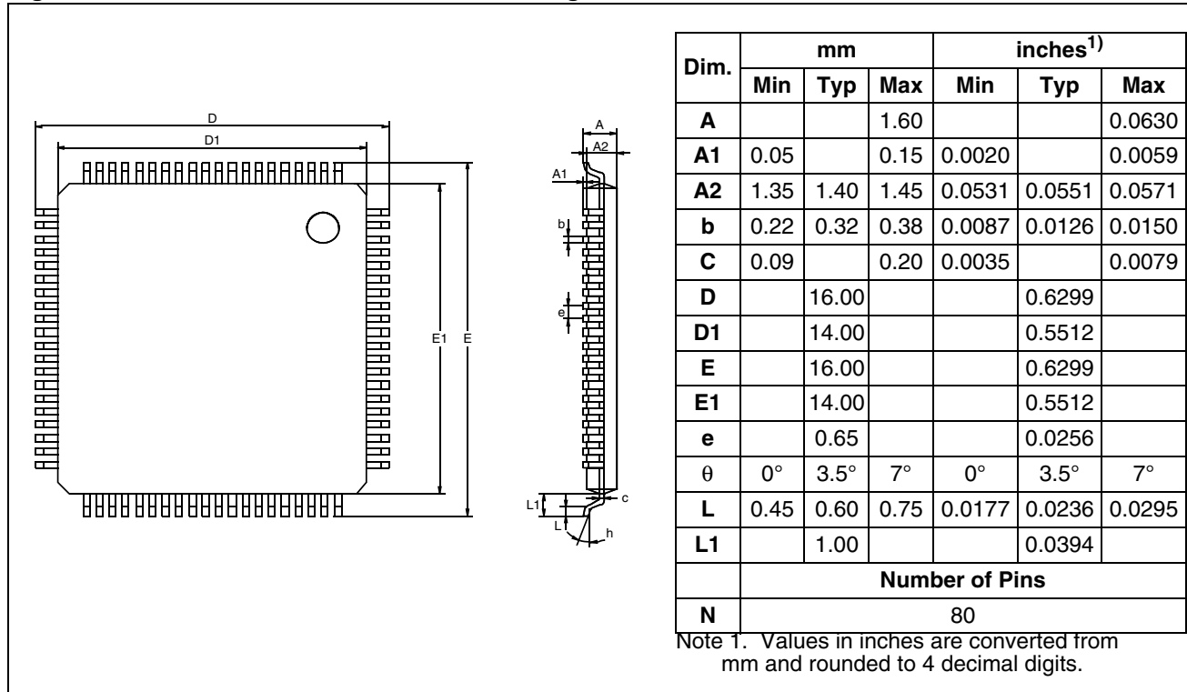
Figure 96. 80-Pin Low Profile Quad Flat Package
