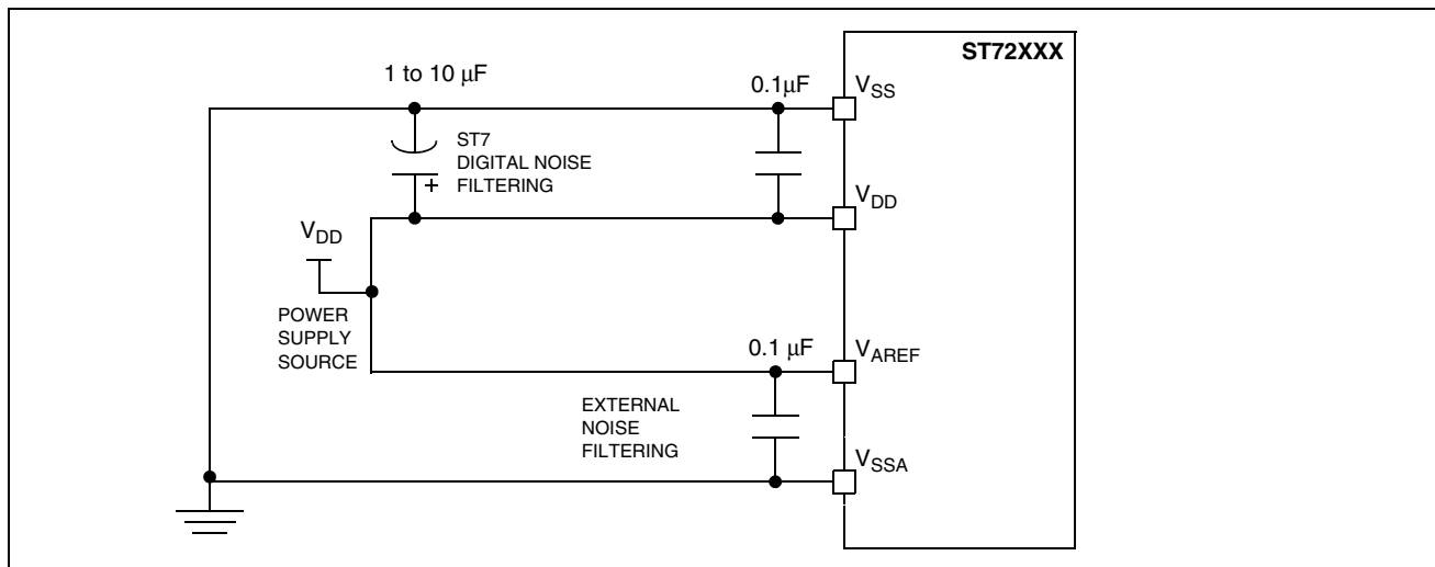
Figure 94. Power Supply Filtering
