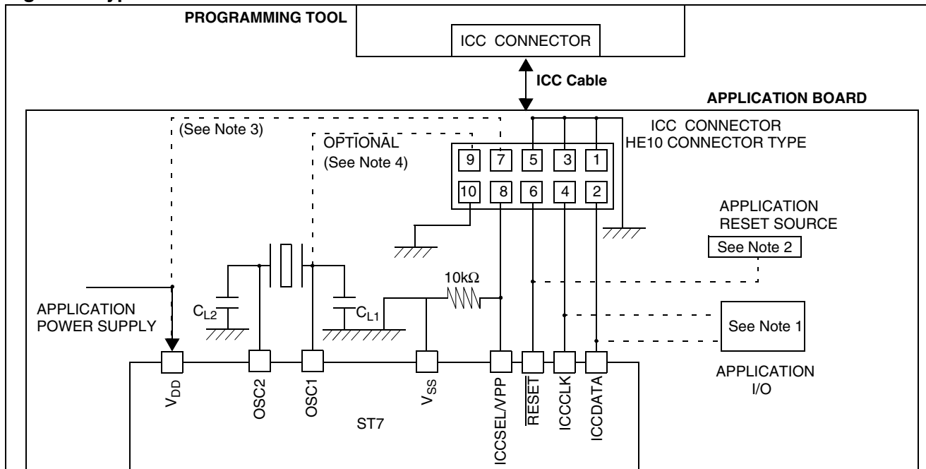
Figure 5. Typical ICC Interface
