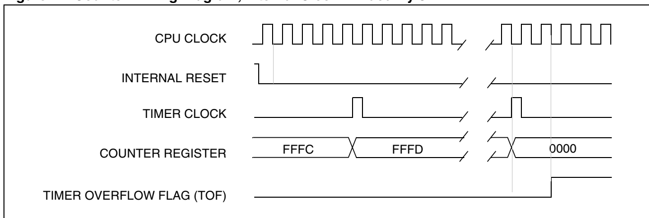
Figure 42. Counter Timing Diagram, Internal Clock Divided By 8
