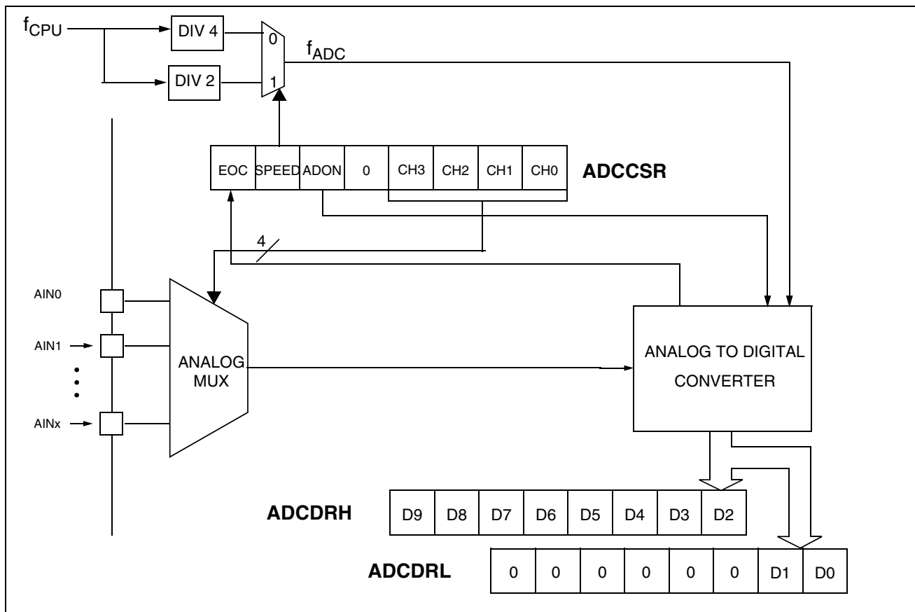
Figure 65. ADC Block Diagram
