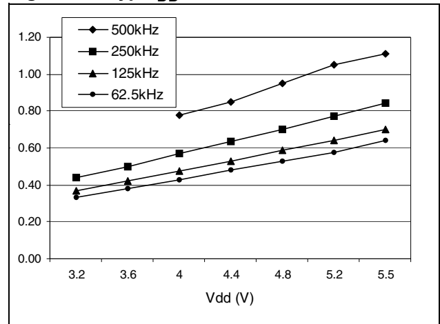
Figure 72. Typ. I_{DD} in Slow-wait mode
