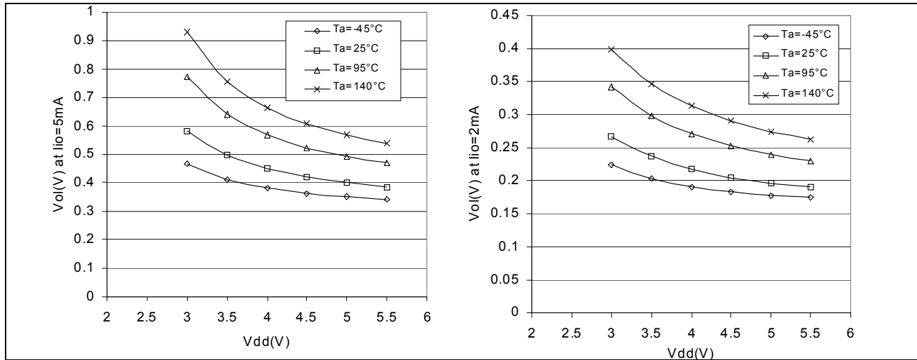
Figure 82. Typical V_{OL} vs. V_{DD} (high-sink)
