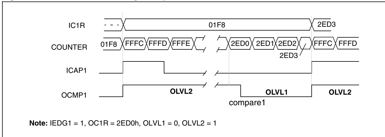
Figure 48. One Pulse Mode Timing Example
