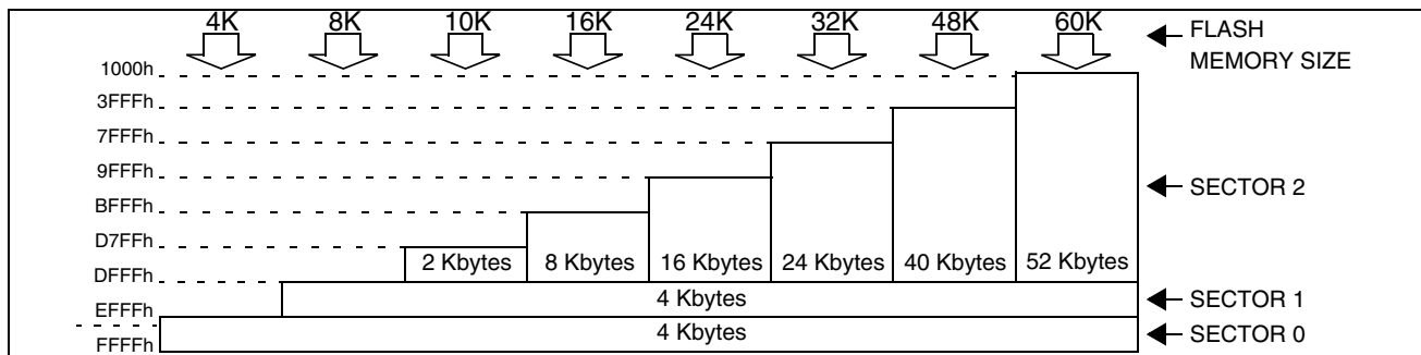
Figure 4. Memory Map and Sector Address
