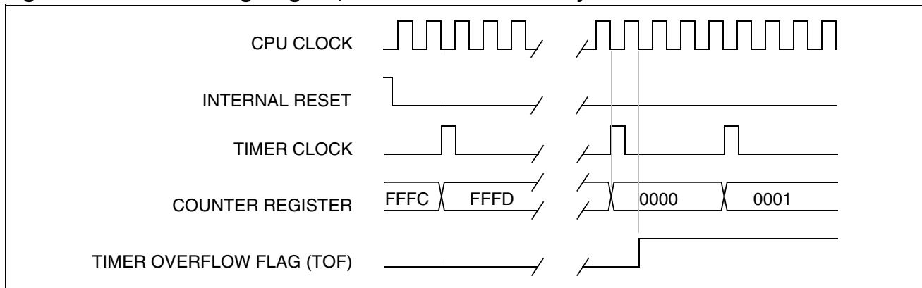
Figure 41. Counter Timing Diagram, Internal Clock Divided by 4
