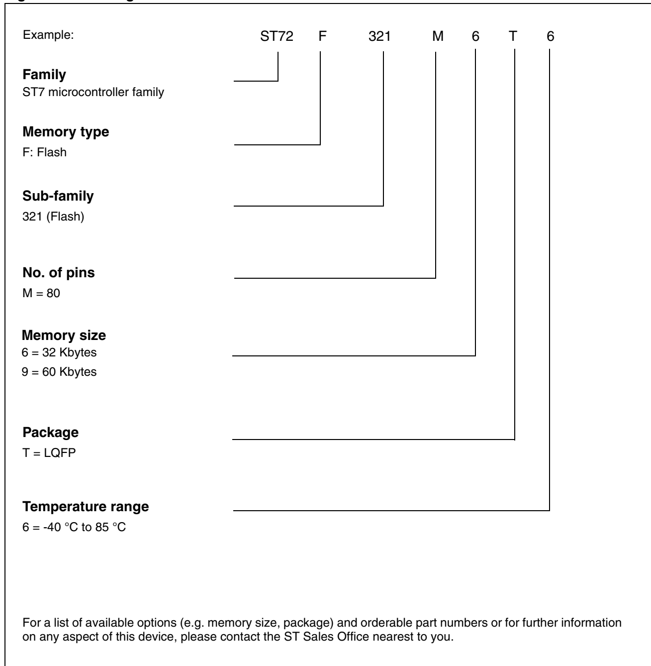
Figure 97. Ordering information scheme
