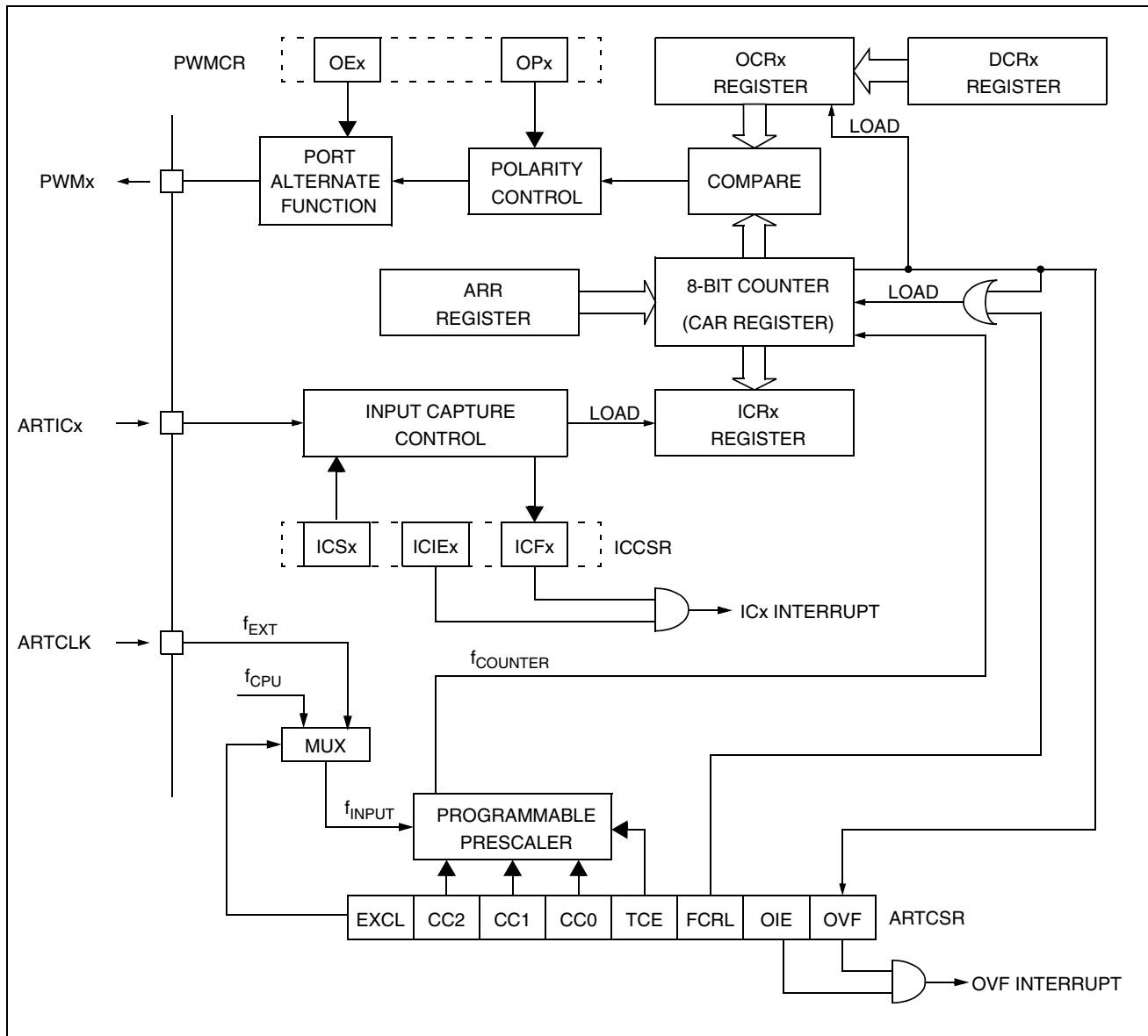
Figure 33. PWM Auto-Reload Timer Block Diagram
