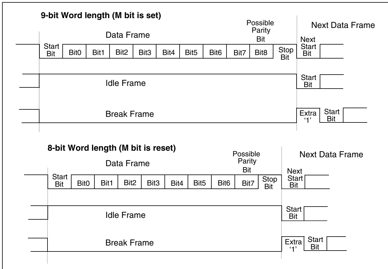
Figure 58. Word Length Programming
