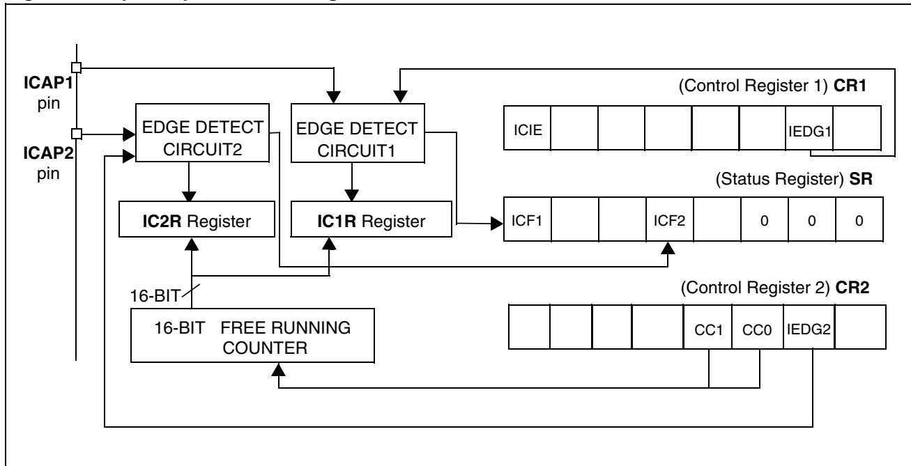
Figure 43. Input Capture Block Diagram
