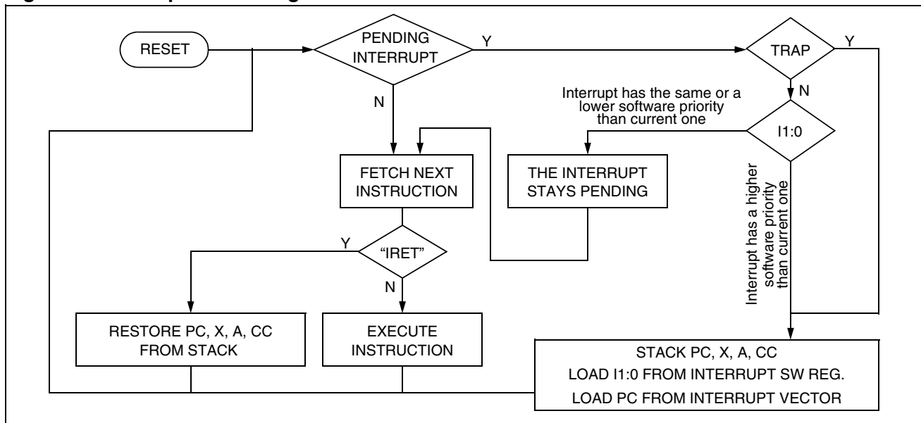
Figure 17. Interrupt Processing Flowchart
