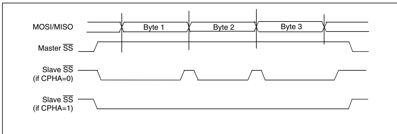
Figure 53. Hardware/Software Slave Select Management
