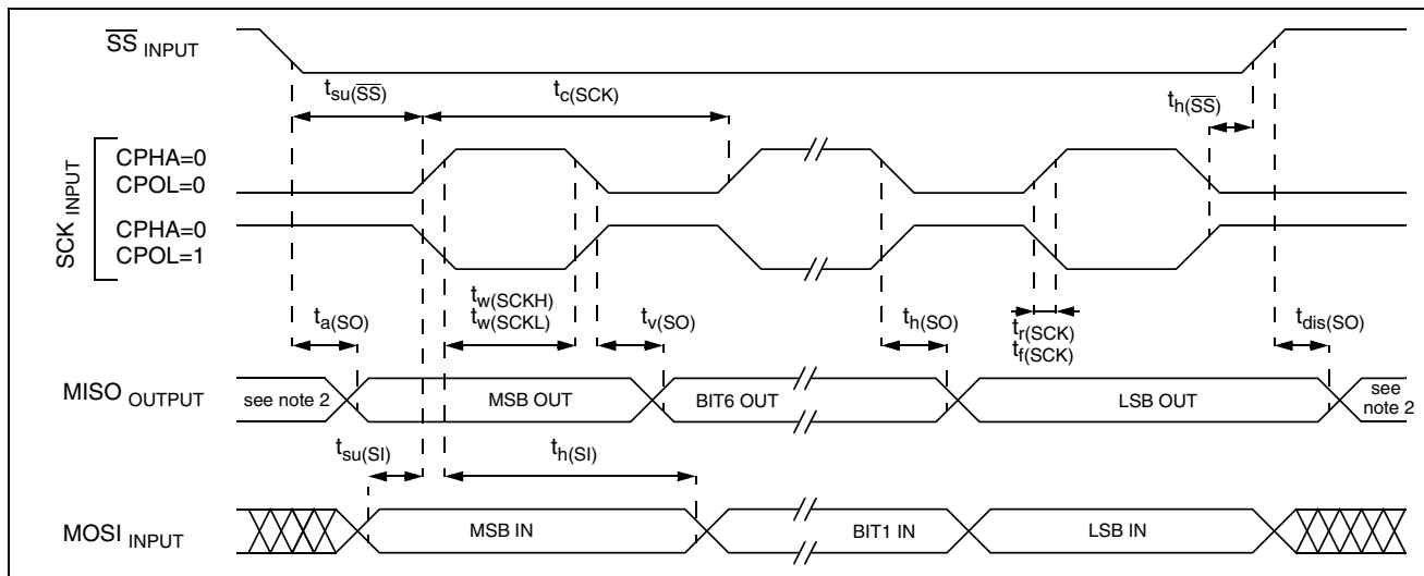
Figure 87. SPI Slave Timing Diagram with CPHA=0 3)
