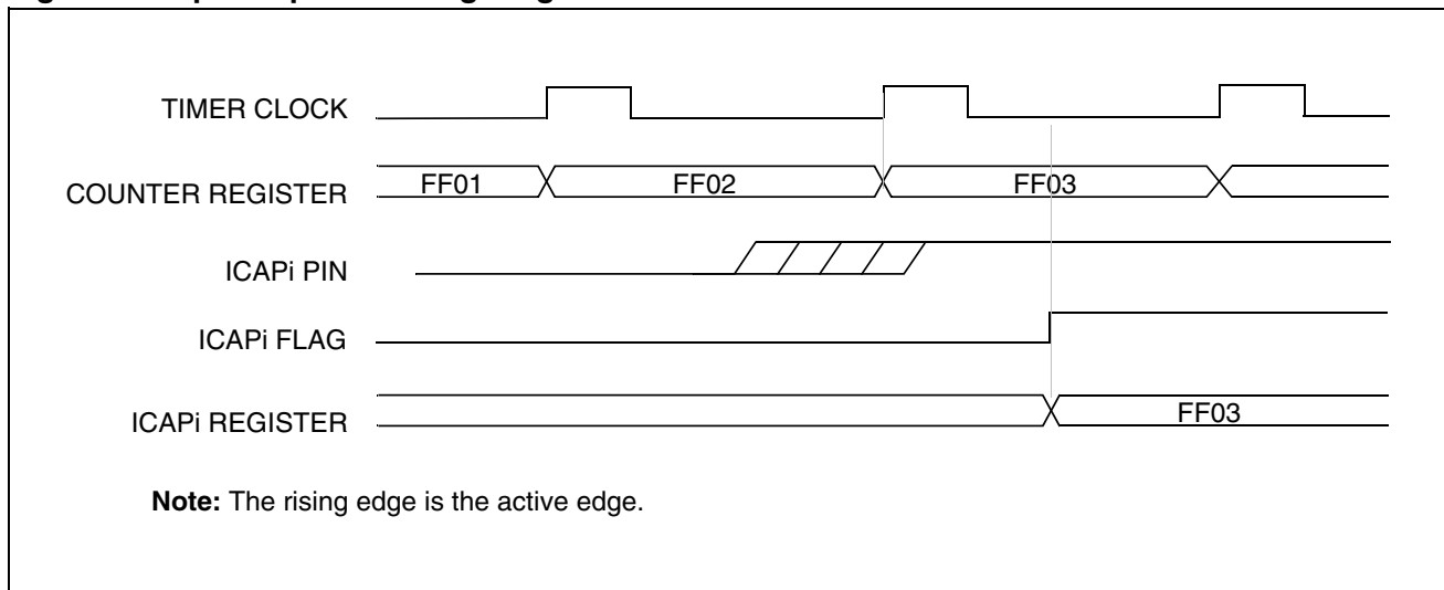
Figure 44. Input Capture Timing Diagram
