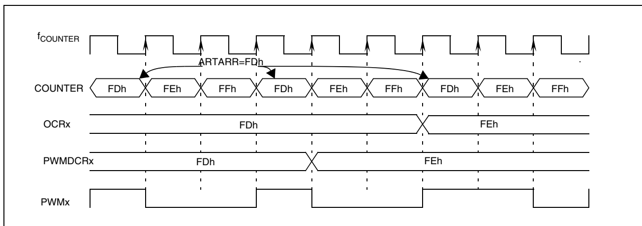
Figure 34. Output compare control
