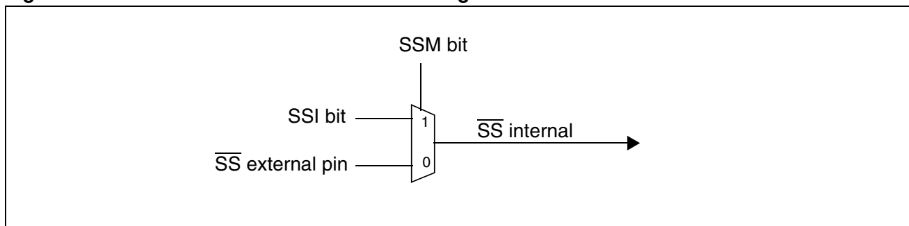
Figure 53. Hardware/Software Slave Select Management
