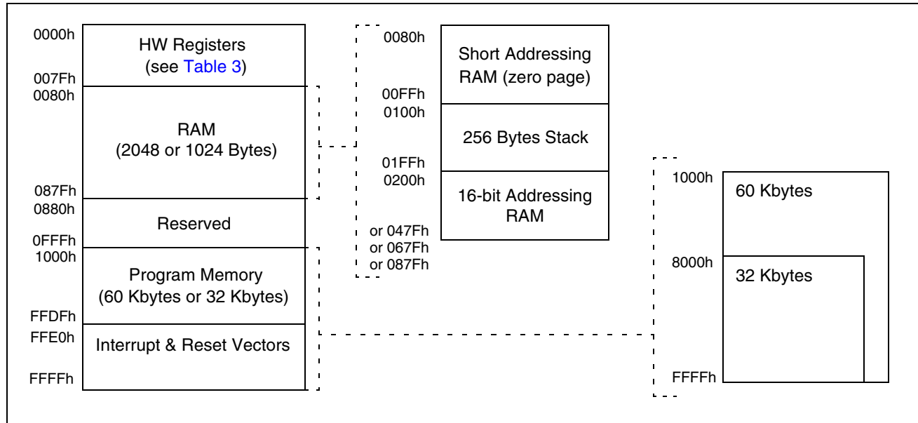
Figure 3. Memory Map
