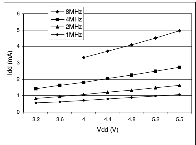
Figure 72. Typ. I_{DD} in Slow-wait mode
