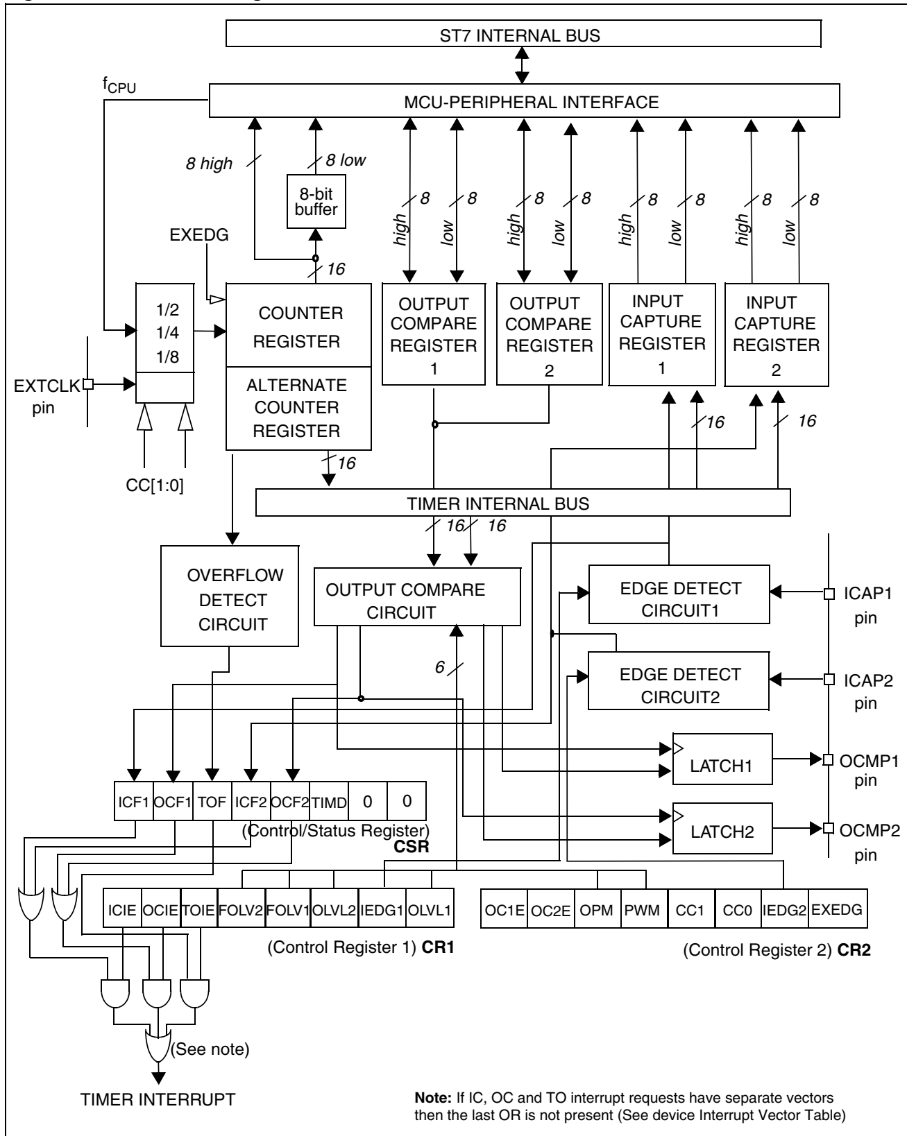
Figure 39. Timer Block Diagram
