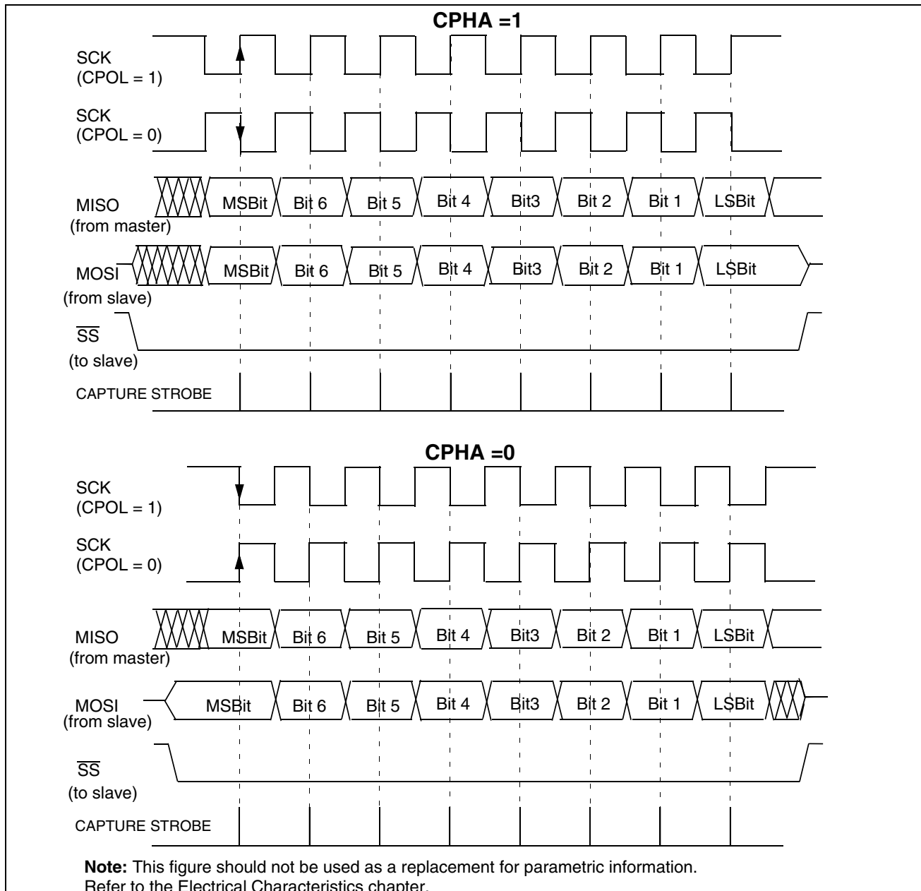
Figure 54. Data Clock Timing Diagram
