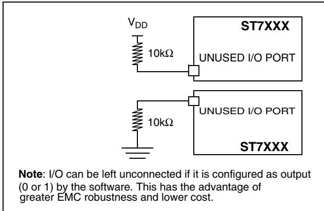
Figure 76. Unused I/O Pins configured as input
