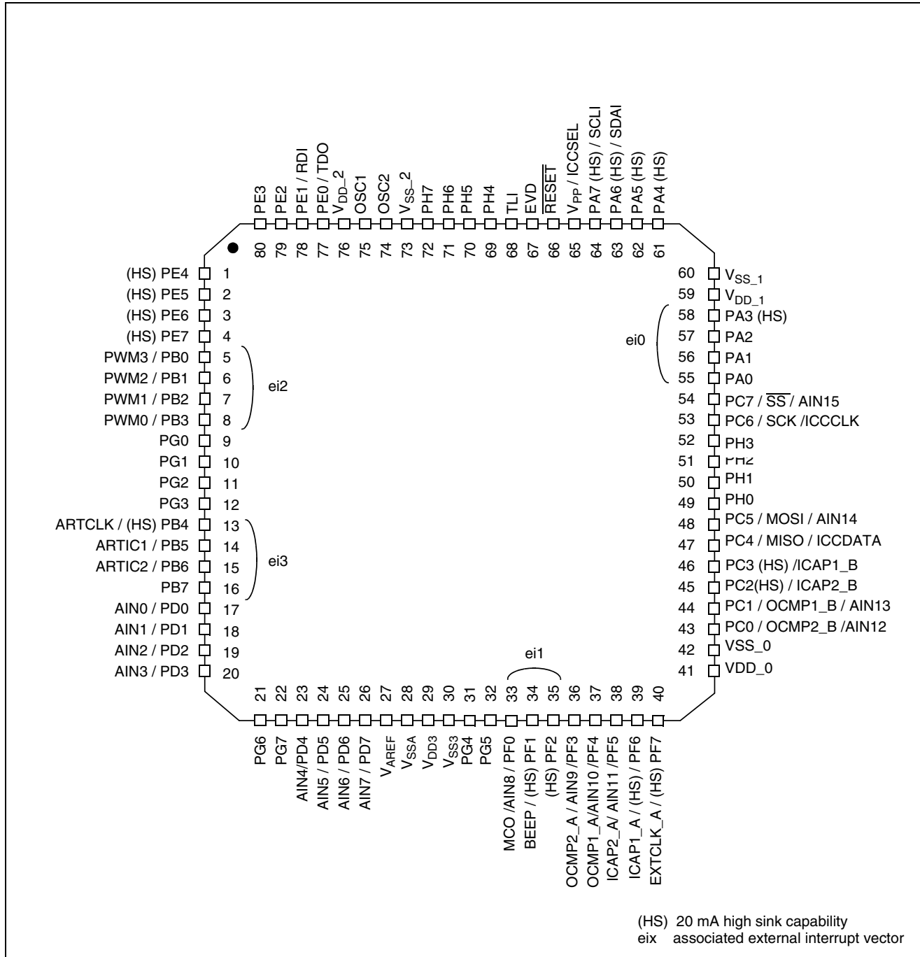
Figure 2. 80-Pin LQFP 14x14 Package Pinout
