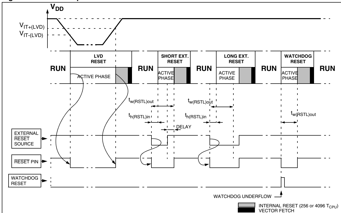
Figure 13. RESET Sequences
