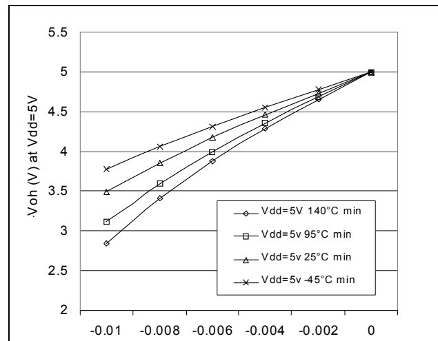
Figure 80. Typical V_{OH} at V_{DD}=5\text{ V}
