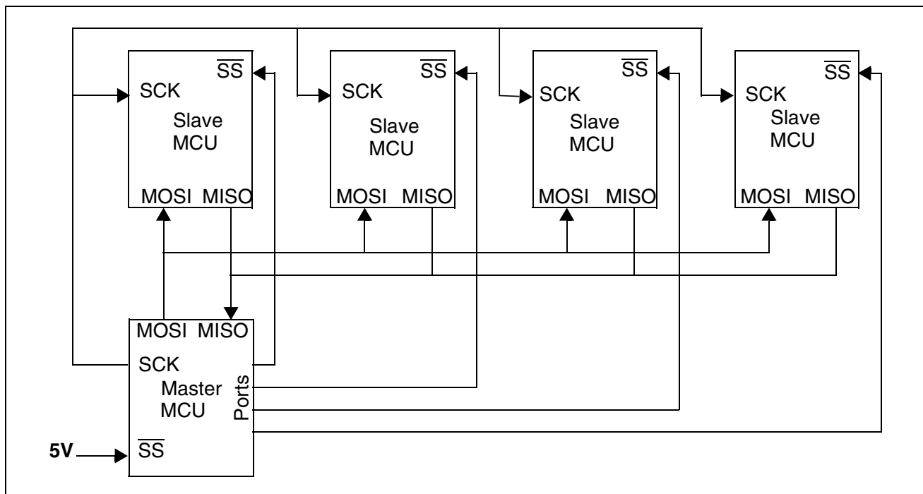
Figure 56. Single Master / Multiple Slave Configuration
