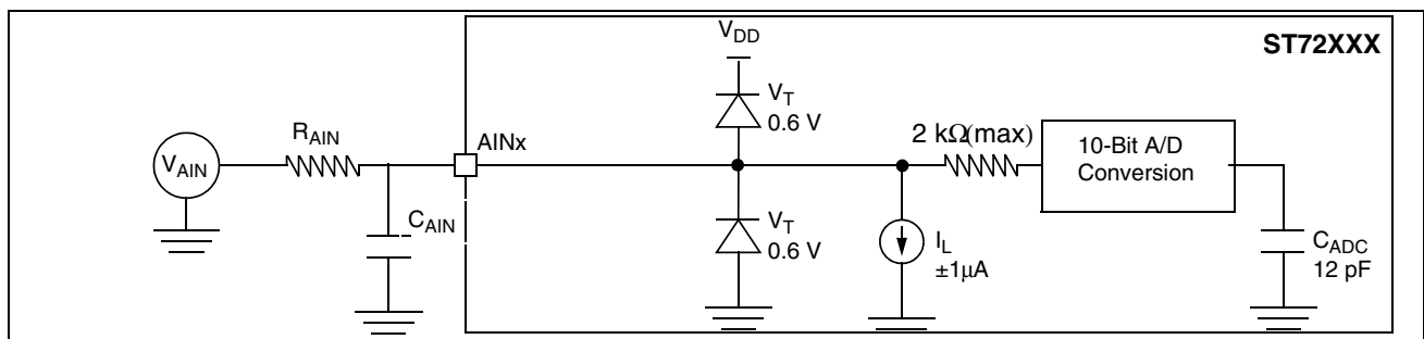
Figure 93. Typical A/D Converter Application
