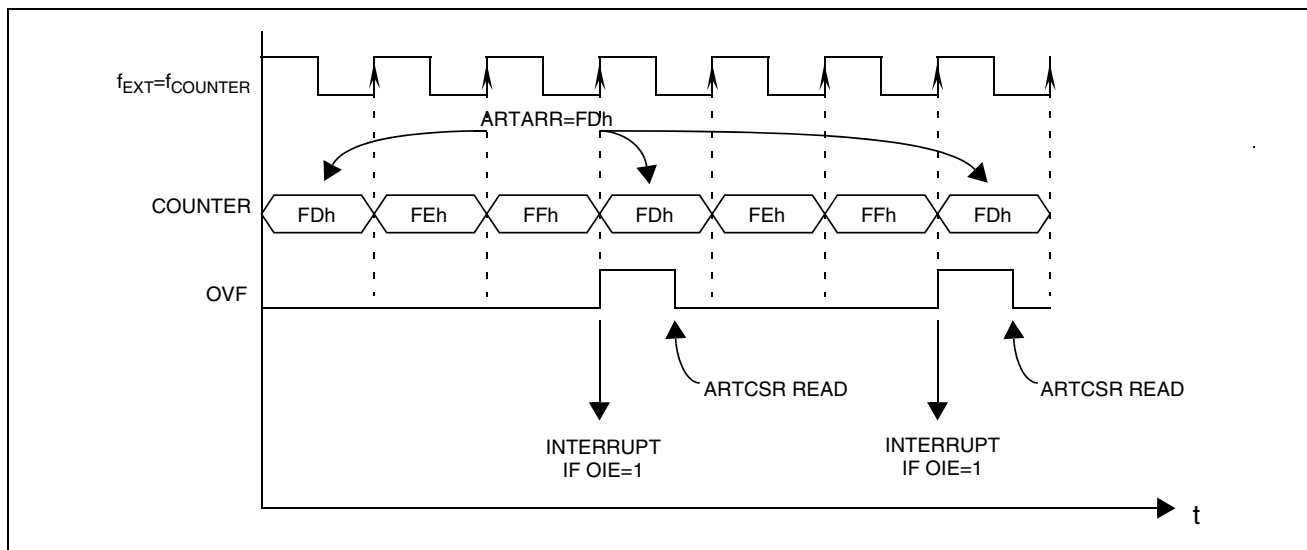
Figure 37. External Event Detector Example (3 counts)
