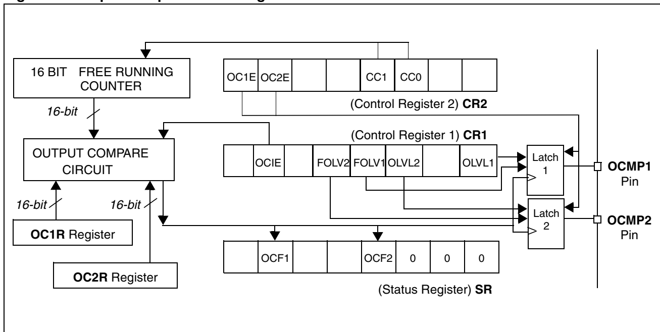
Figure 45. Output Compare Block Diagram
