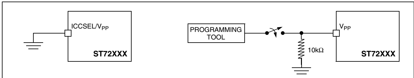
Figure 86. Two typical Applications with ICCSEL/V PP Pin 1)
