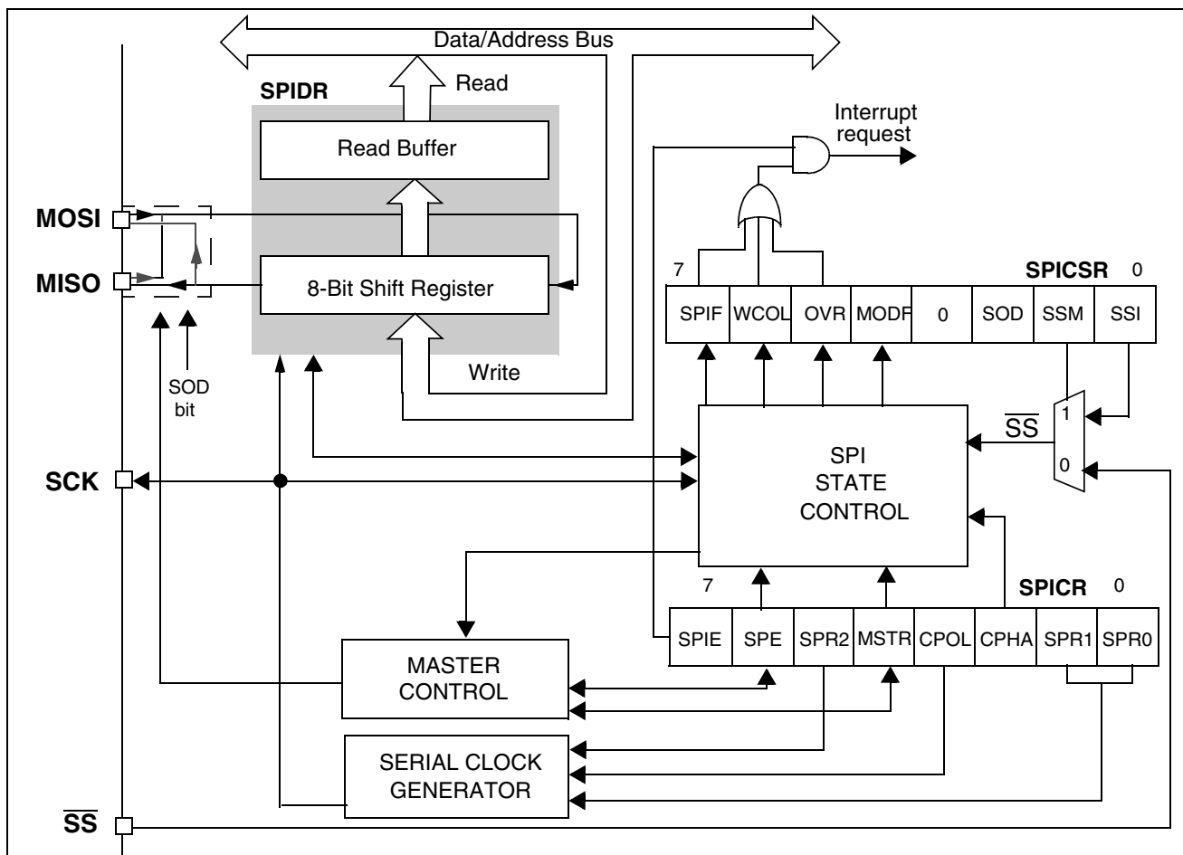
Figure 50. Serial Peripheral Interface Block Diagram
