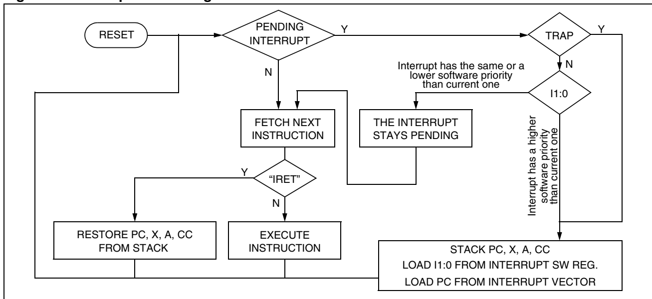
Figure 15. Interrupt Processing Flowchart
