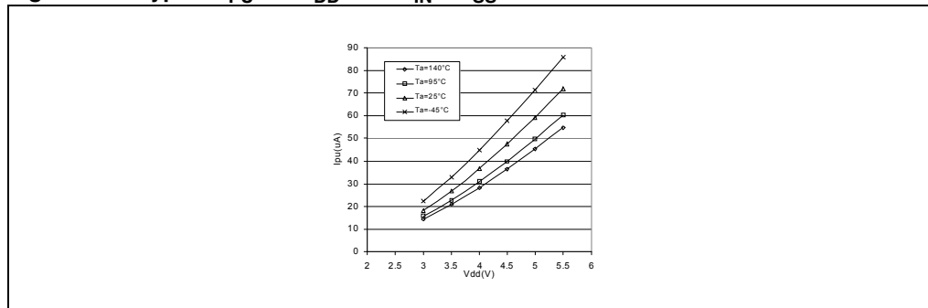
Figure 69. Typical I PU vs. V DD with V IN = V SS
