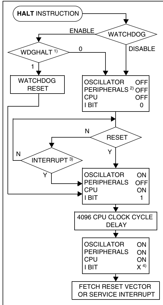
Figure 19. HALT Mode Flow-chart
