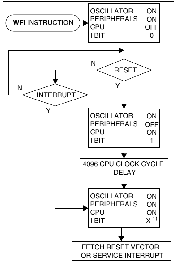
Figure 17. WAIT Mode Flowchart
