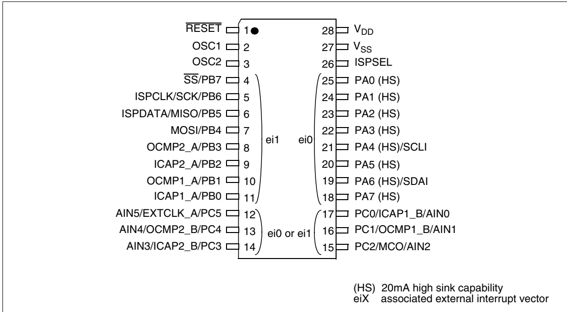
Figure 2. 28-Pin SO Package Pinout
