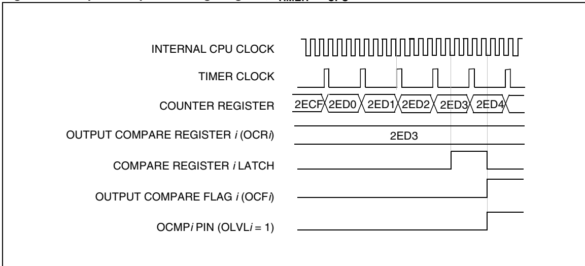
Figure 33. Output Compare Timing Diagram, f_{\text{TIMER}} = f_{\text{CPU}}/4
