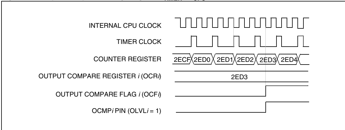
Figure 32. Output Compare Timing Diagram, f_{\text{TIMER}} = f_{\text{CPU}}/2
