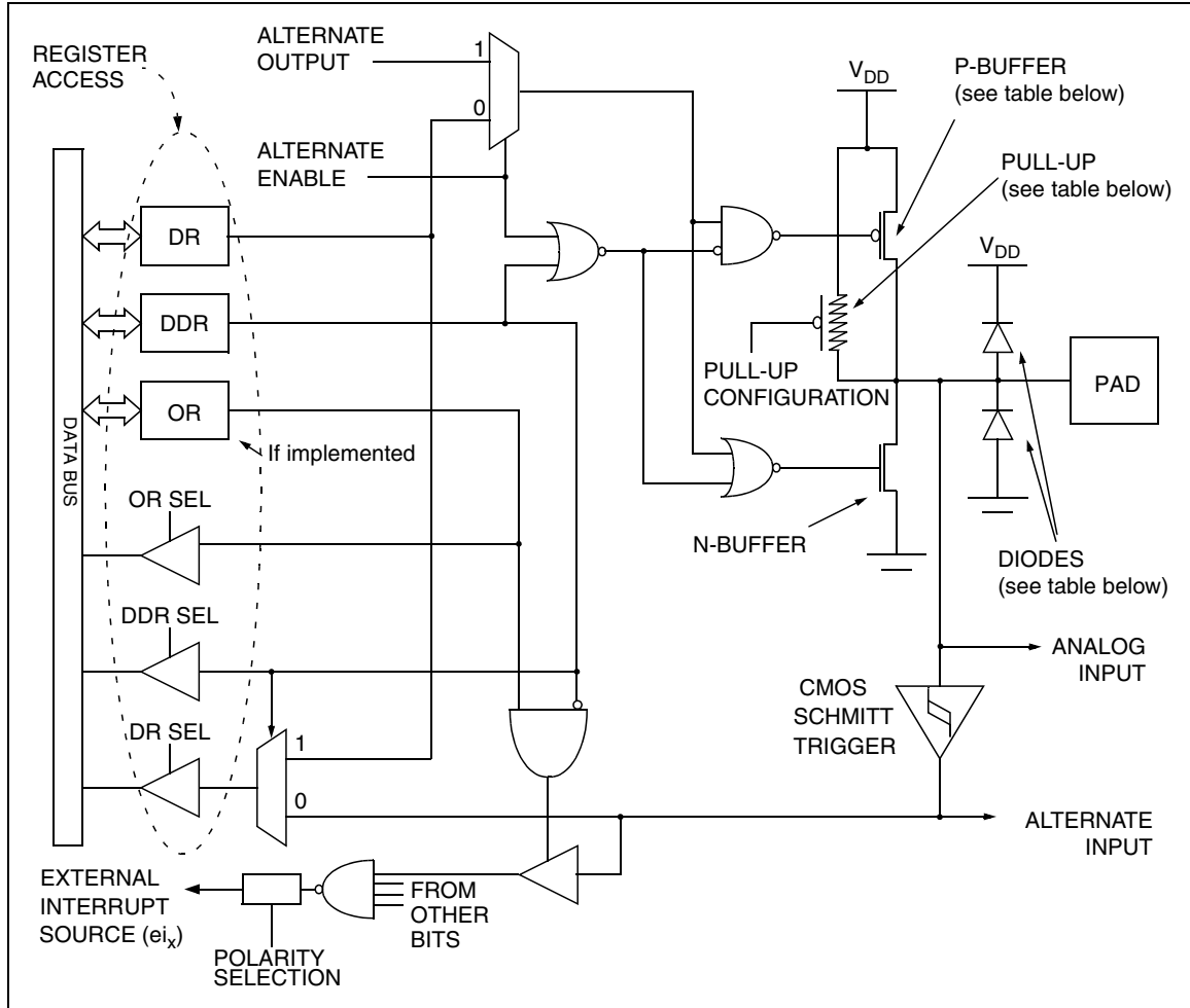
Figure 20. I/O Port General Block Diagram
