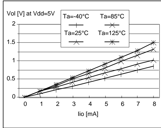
Figure 87. Typical V_{OL} at V_{DD}=5V (RESET)
