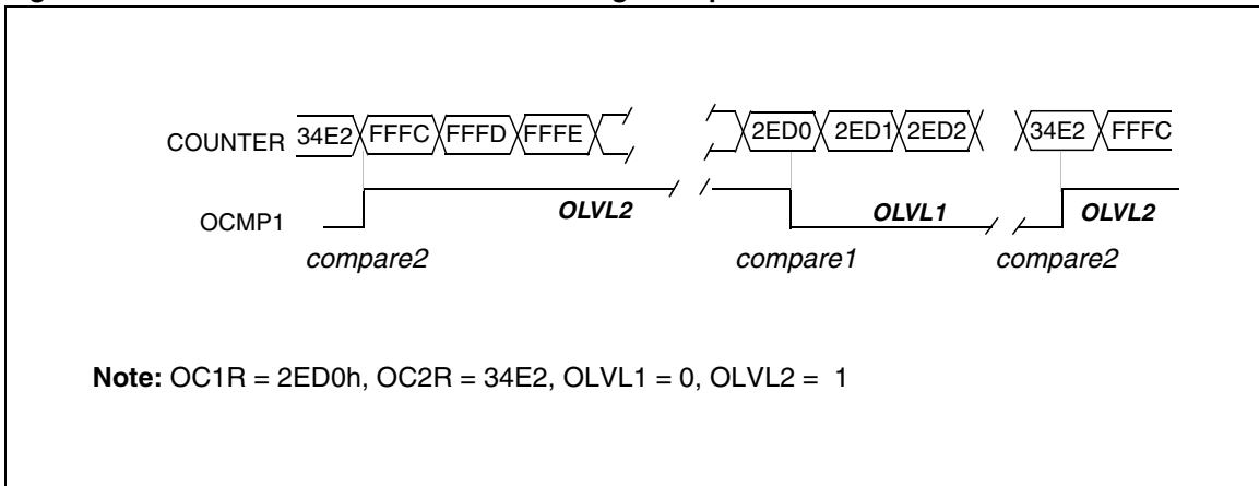
Figure 35. Pulse Width Modulation Mode Timing Example
