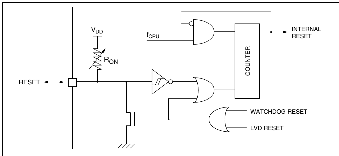
Figure 10. Reset Block Diagram
