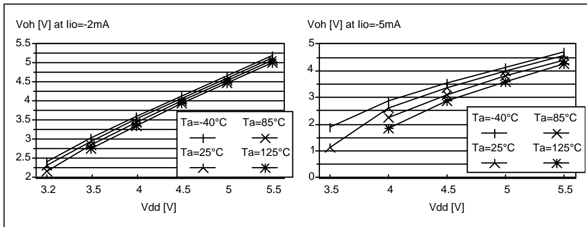
Figure 84. Typical V_{OH} vs. V_{DD}
