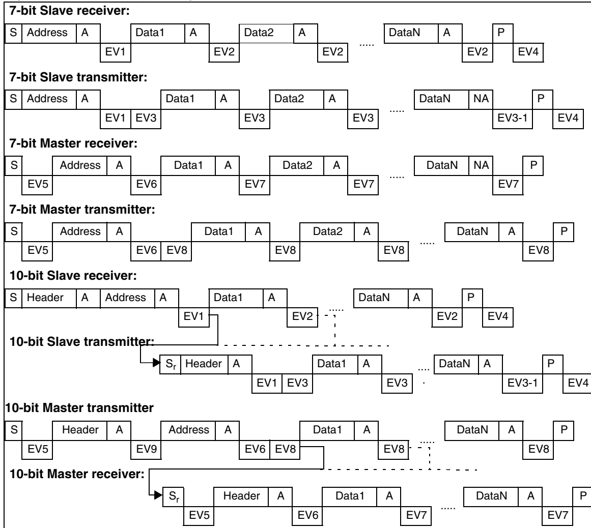
Figure 44. Transfer Sequencing
