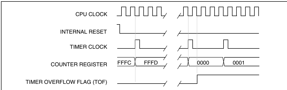
Figure 28. Counter Timing Diagram, internal clock divided by 8
