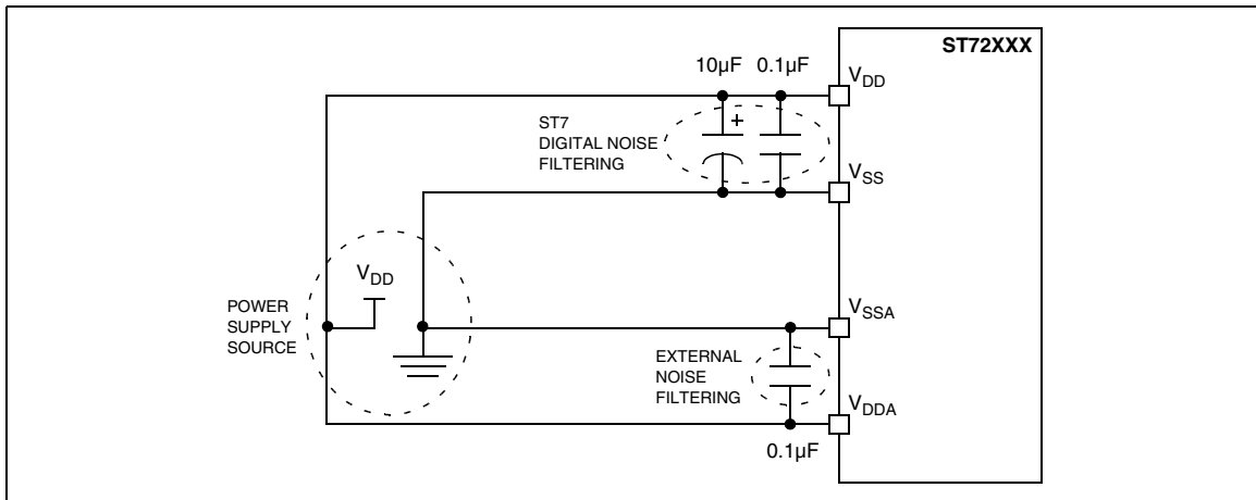
Figure 69. EMC Recommended star network power supply connection 2)
