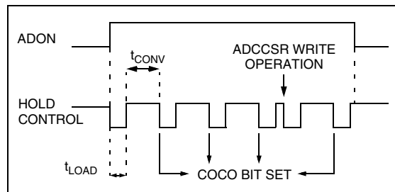
Figure 47. ADC Conversion Timings
