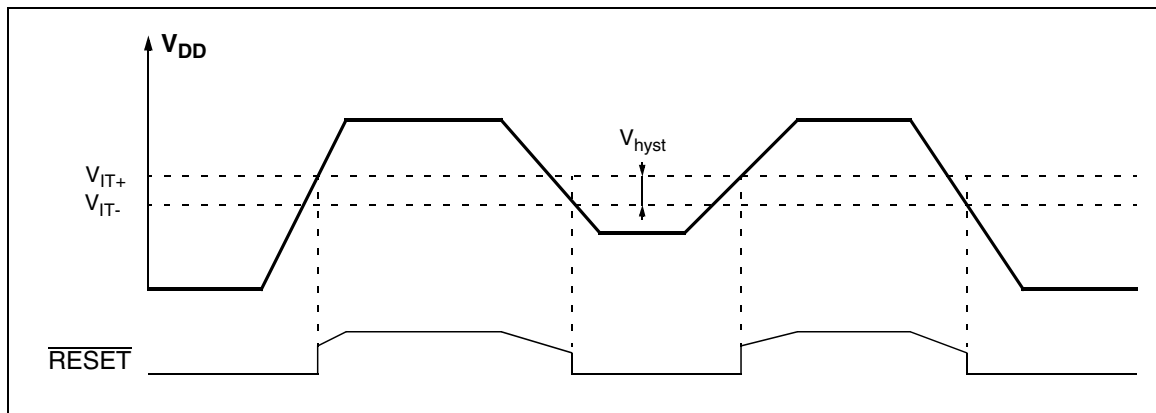
Figure 8. Low Voltage Detector vs Reset
