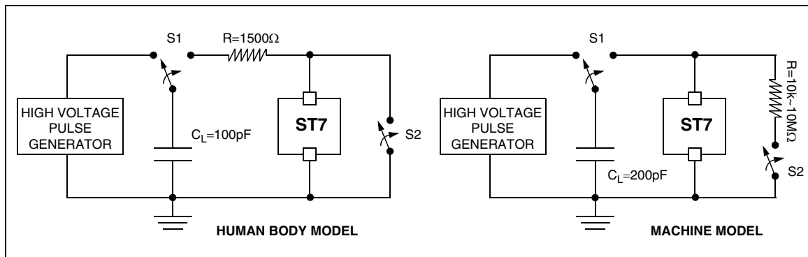
Figure 70. Typical Equivalent ESD Circuits
