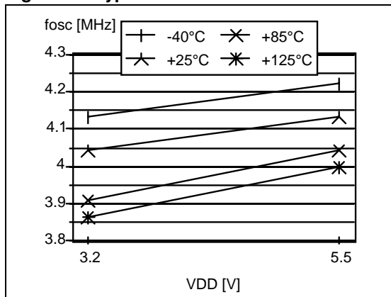
Figure 66. Typical Internal RC Oscillator
