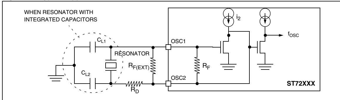
Figure 64. Typical Application with Ceramic Resonator
