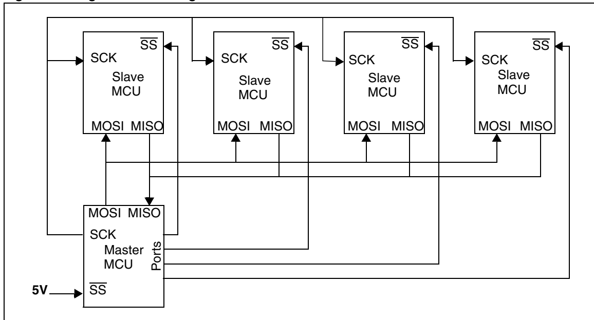
Figure 41. Single Master Configuration
