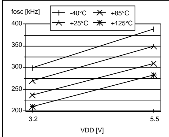
Figure 68. Typical Safe Oscillator Frequencies
