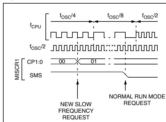
Figure 16. SLOW Mode Clock Transitions
