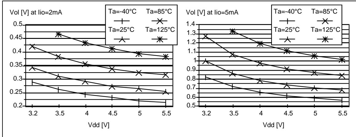
Figure 83. Typical V_{OL} vs. V_{DD} (high-sink I/Os)
