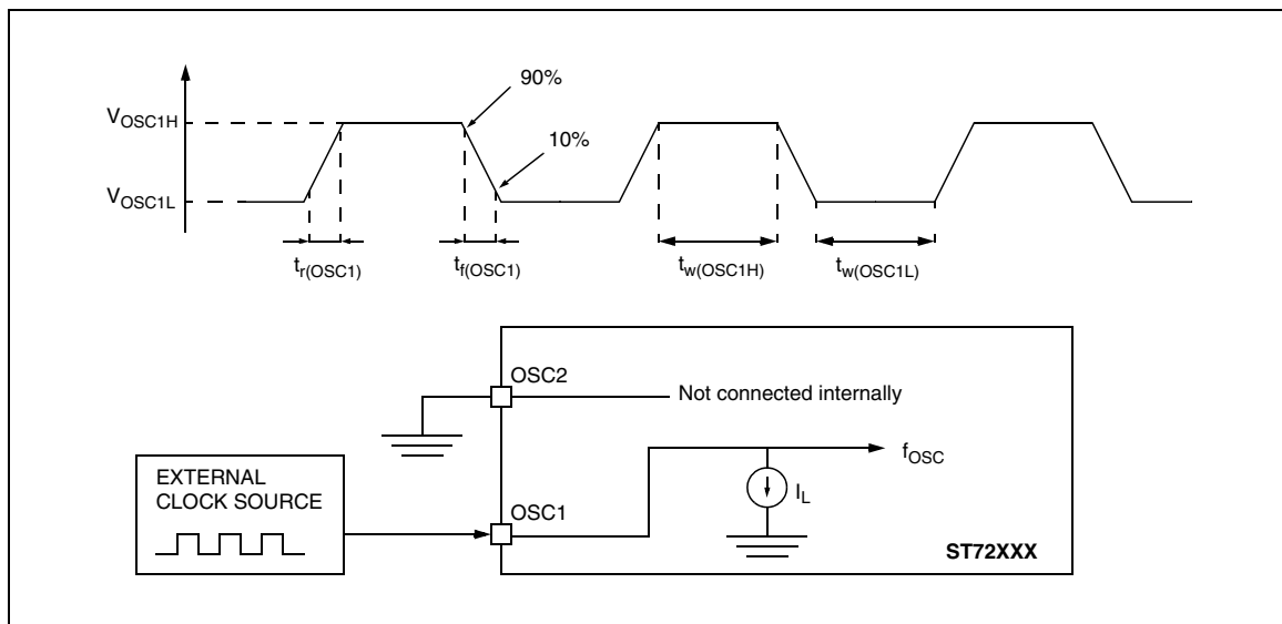
Figure 62. Typical Application with an External Clock Source
