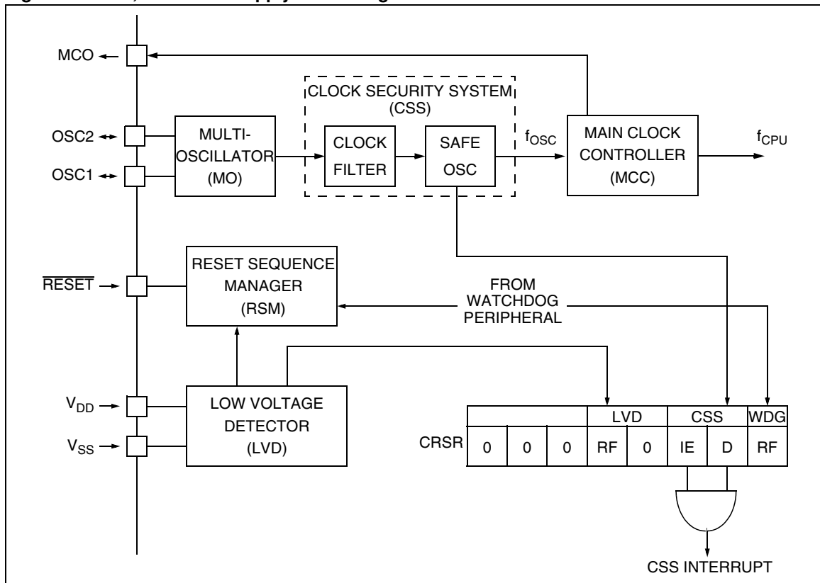
Figure 7. Clock, Reset and Supply Block Diagram
