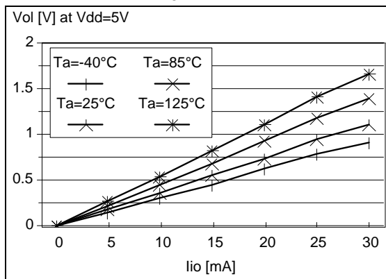
Figure 80. Typical V_{OL} at V_{DD}=5V (high-sink)
