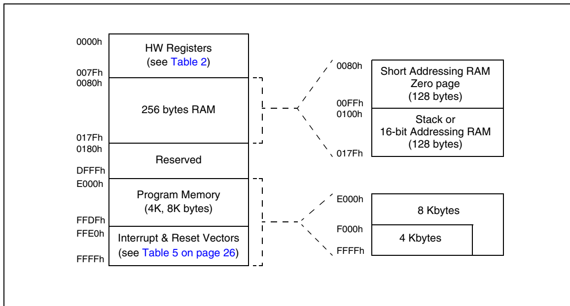
Figure 3. Memory Map
