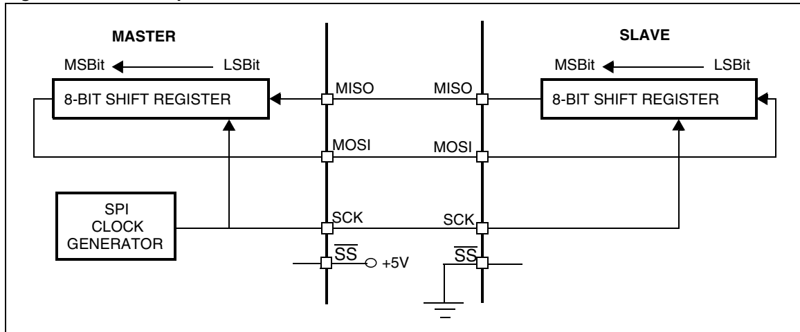
Figure 36. Serial Peripheral Interface Master/Slave
