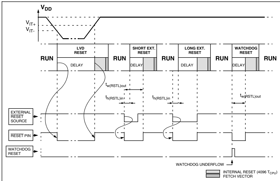
Figure 11. RESET Sequences
