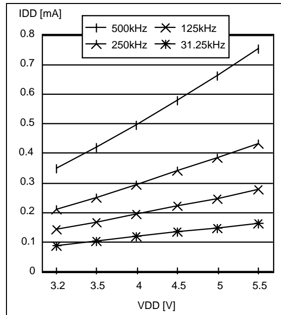
Figure 59. Typical I_{DD} in SLOW vs. f_{CPU}
