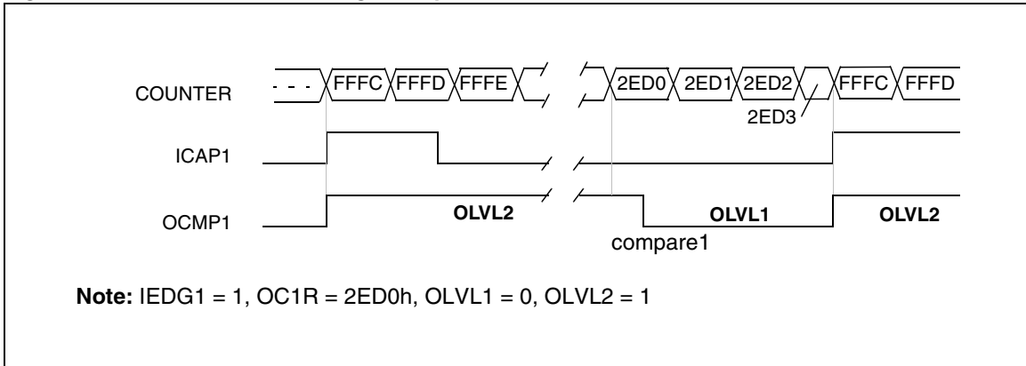
Figure 34. One Pulse Mode Timing Example
