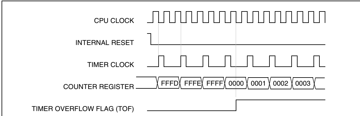
Figure 27. Counter Timing Diagram, internal clock divided by 4
