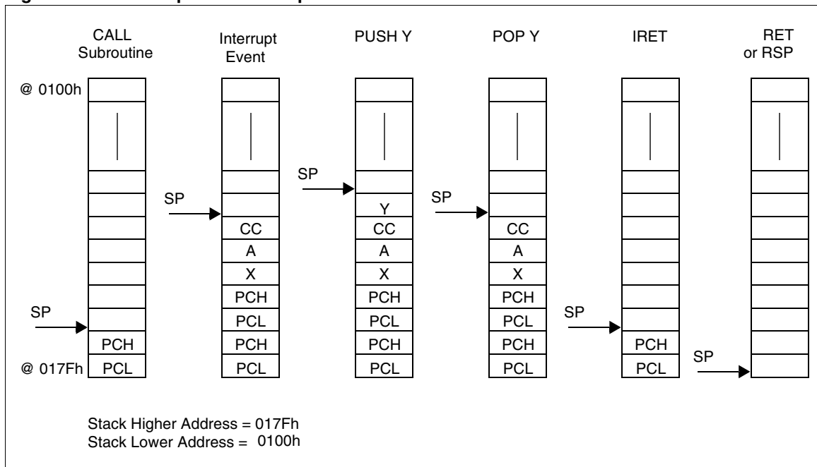
Figure 6. Stack Manipulation Example
