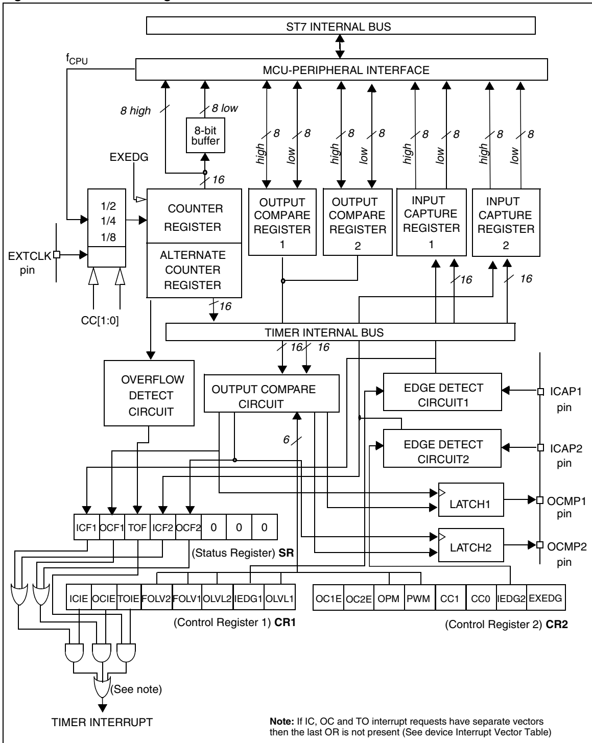
Figure 25. Timer Block Diagram
