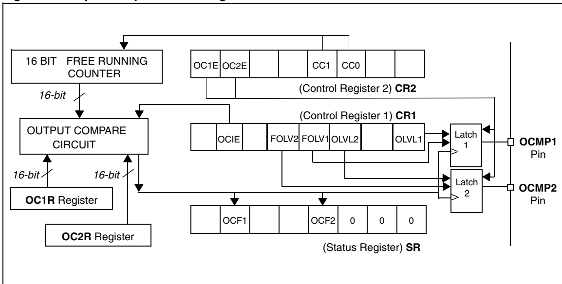
Figure 31. Output Compare Block Diagram
