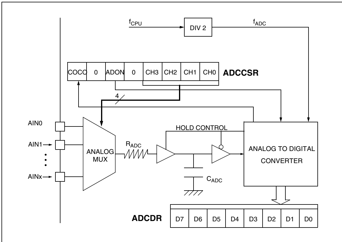
Figure 46. ADC Block Diagram
