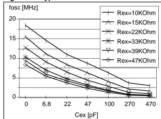
Figure 67. Typical External RC Oscillator
