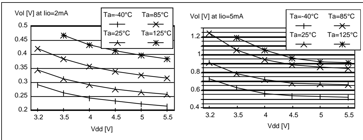
Figure 88. Typical V_{OL} vs. V_{DD} (RESET)
