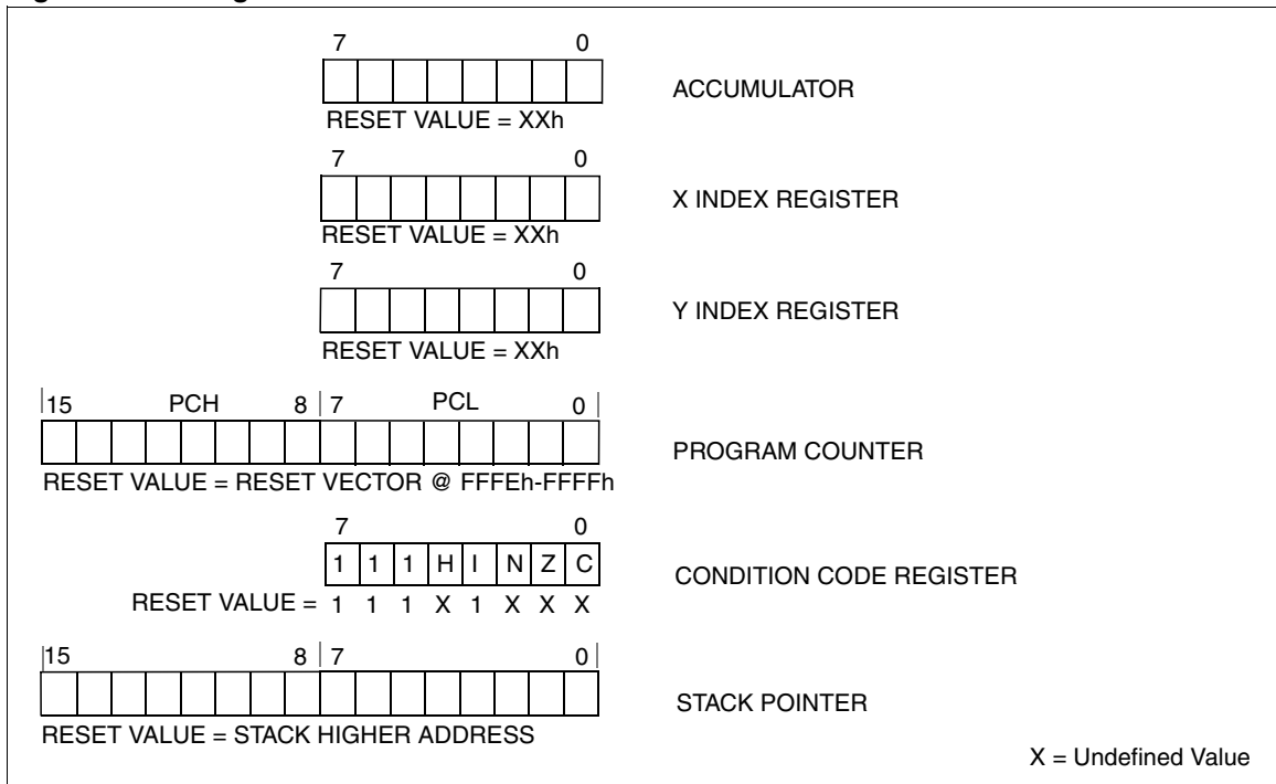
Figure 5. CPU Registers
