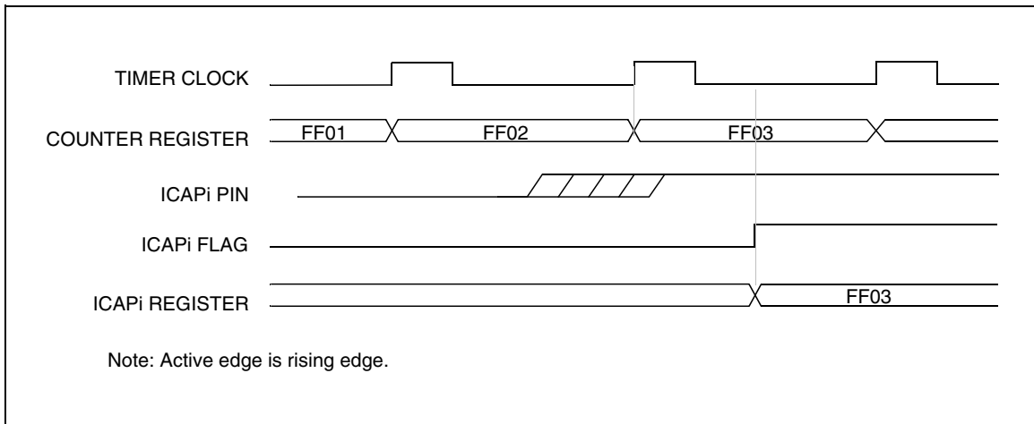
Figure 30. Input Capture Timing Diagram
