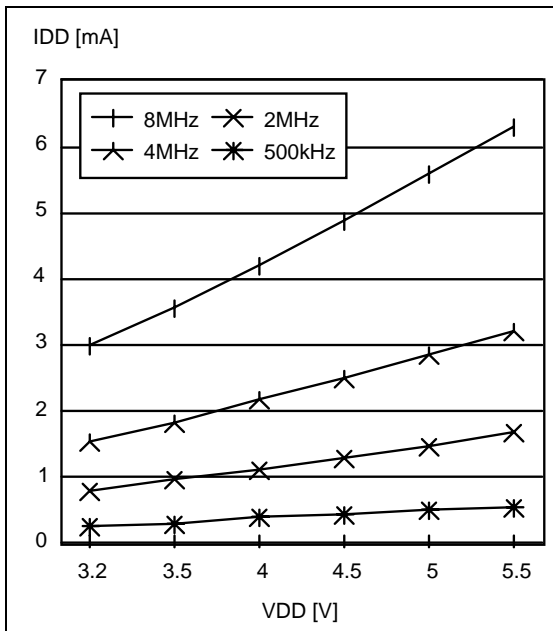
Figure 58. Typical I_{DD} in RUN vs. f_{CPU}
