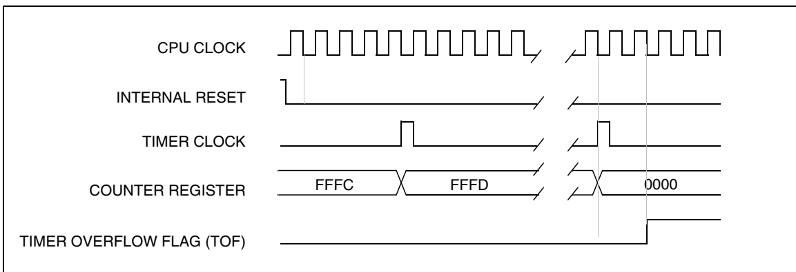
Figure 28. Counter Timing Diagram, internal clock divided by 8
