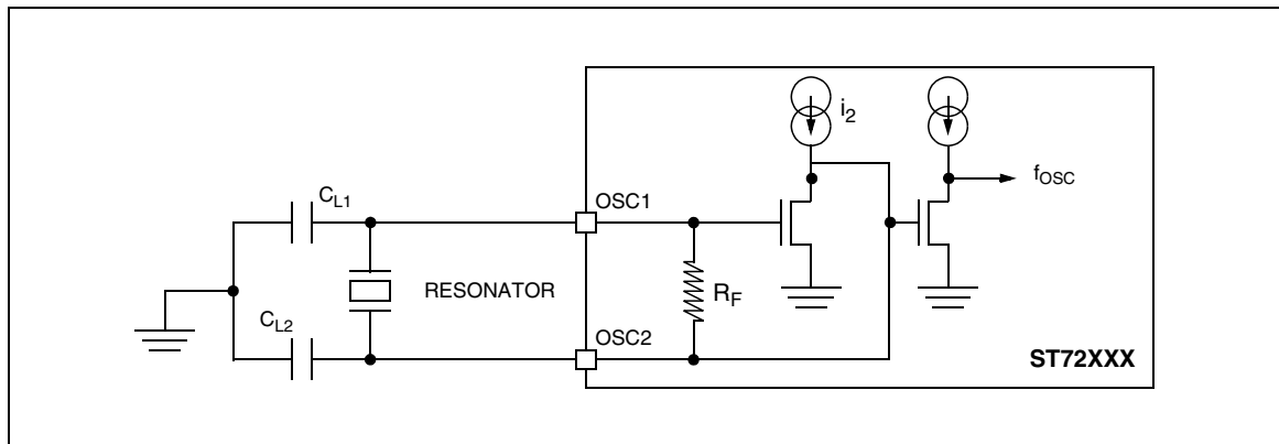
Figure 63. Typical Application with a Crystal Resonator
