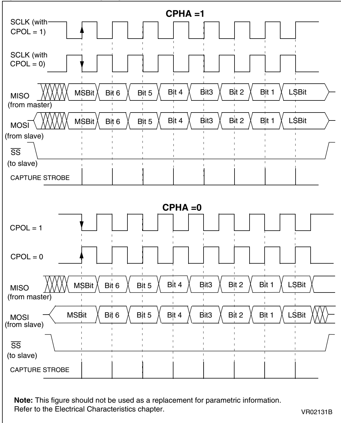
Figure 39. Data Clock Timing Diagram
