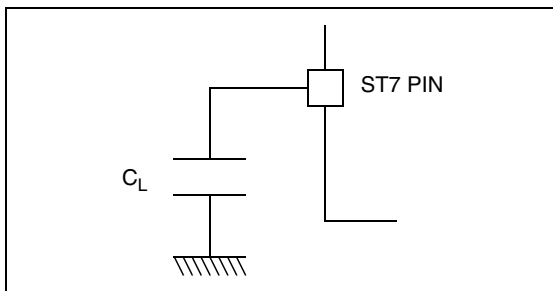
Figure 48. Pin Loading Conditions
