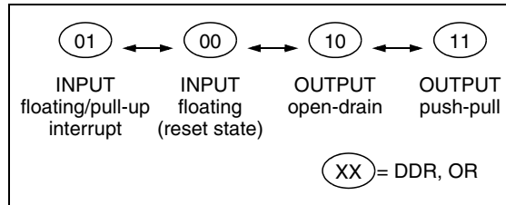
Figure 21. Interrupt I/O Port State Transitions
