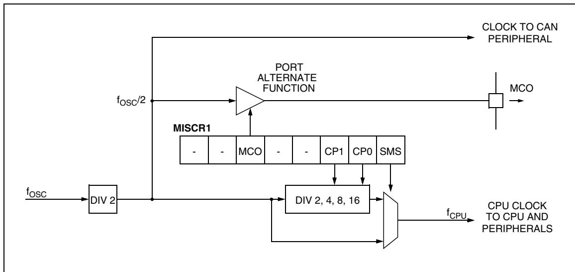
Figure 13. Main Clock Controller (MCC) Block Diagram
