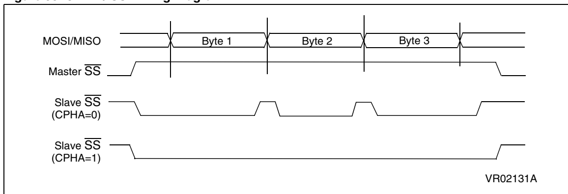
Figure 38. CPHA / \overline{SS} Timing Diagram
