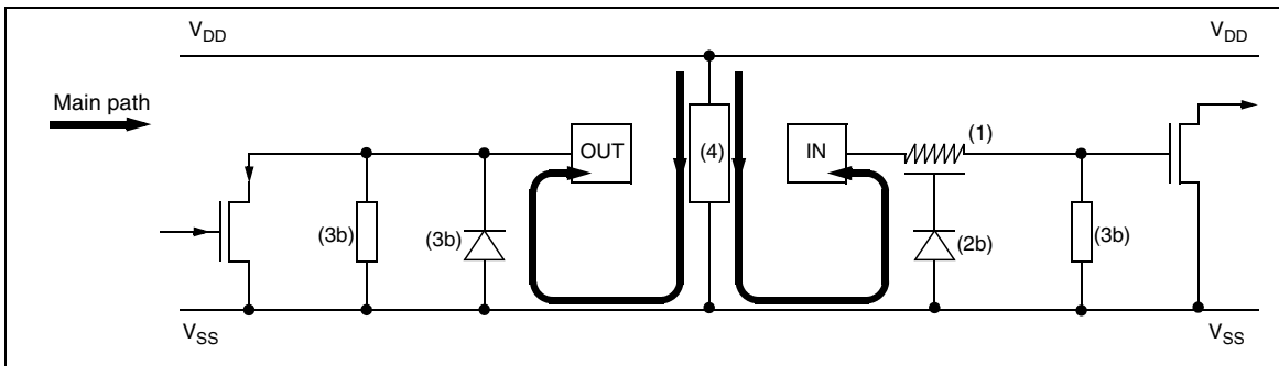
Figure 76. Multisupply Configuration
