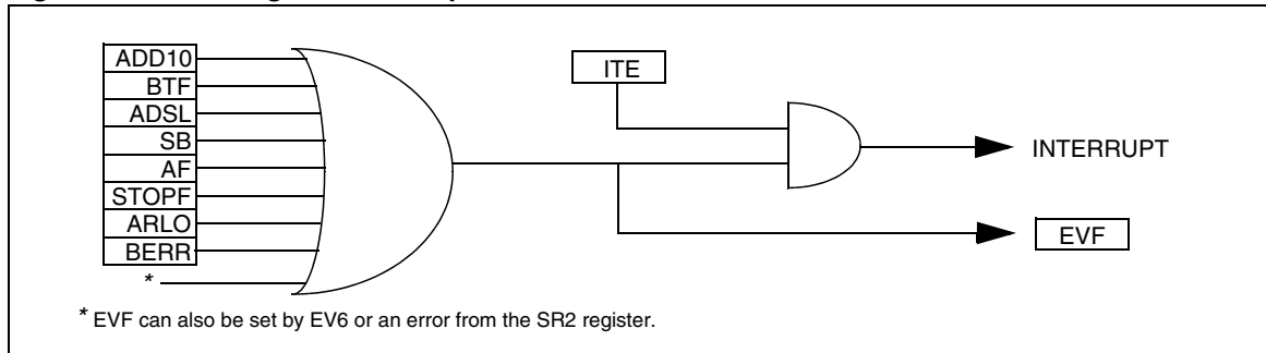
Figure 45. Event Flags and Interrupt Generation
