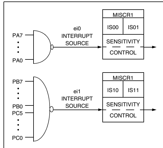
Figure 23. Ext. Interrupt Sensitivity (EXTIT=1)
