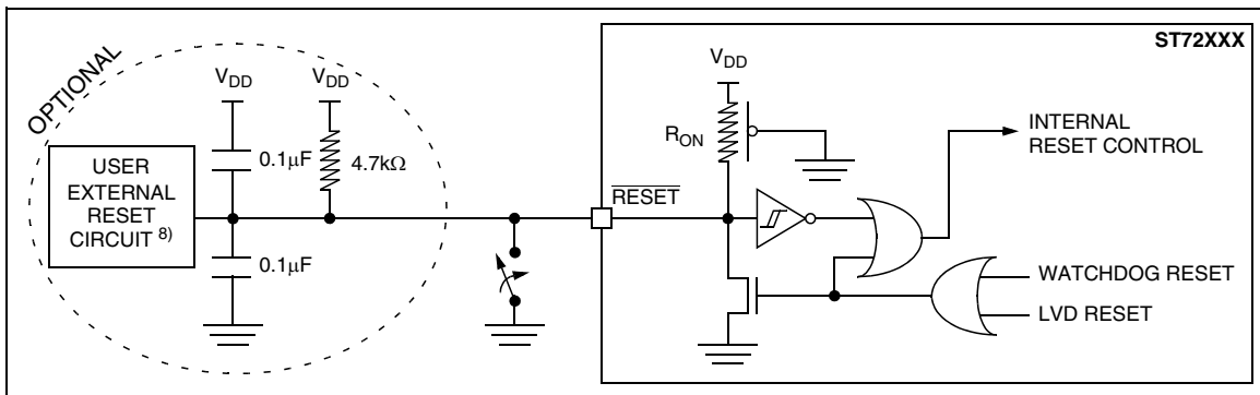
Figure 85. Typical Application with \overline{\text{RESET}} pin 8)
