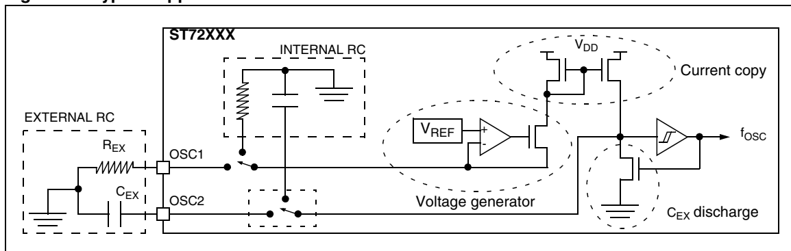
Figure 66. Typical Internal RC Oscillator
