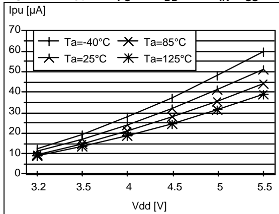
Figure 78. Typical I_{PU} vs. V_{DD} with V_{IN} = V_{SS}
