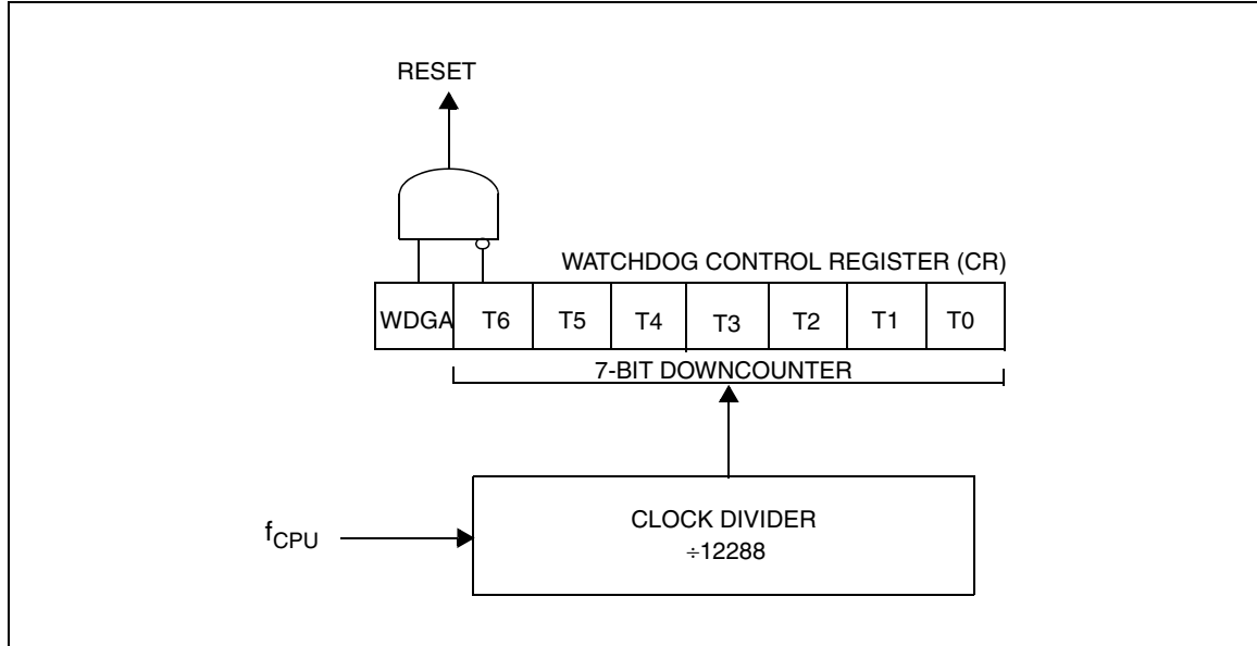
Figure 24. Watchdog Block Diagram
