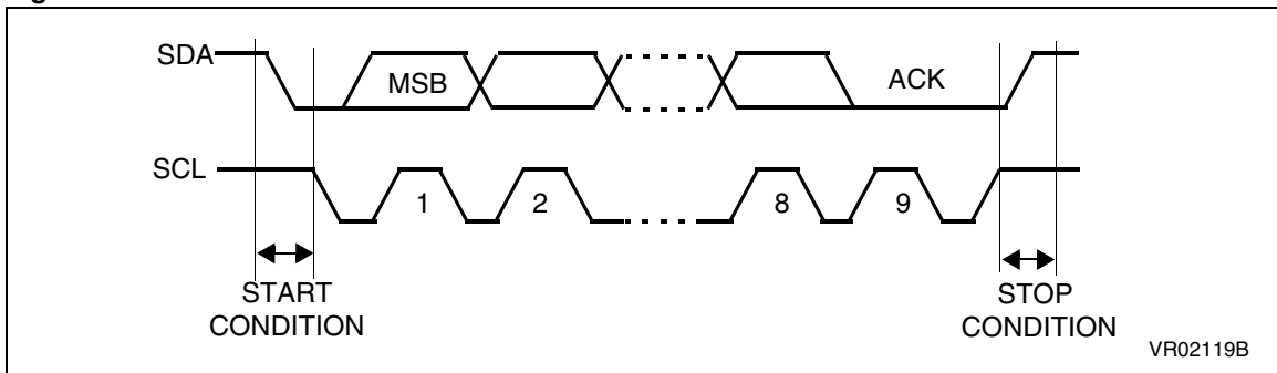
Figure 42. I 2 C BUS Protocol
