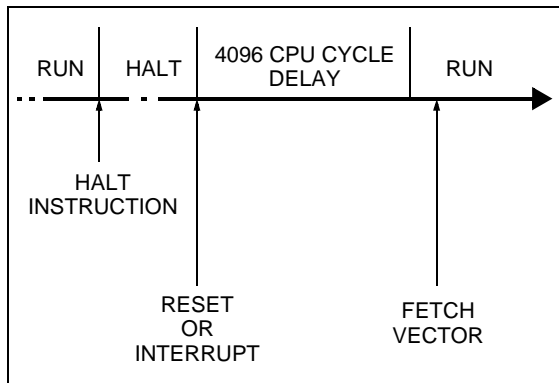
Figure 18. HALT Mode Timing Overview
