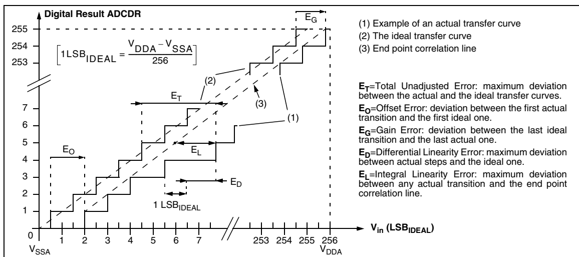
Figure 95. ADC Accuracy Characteristics
