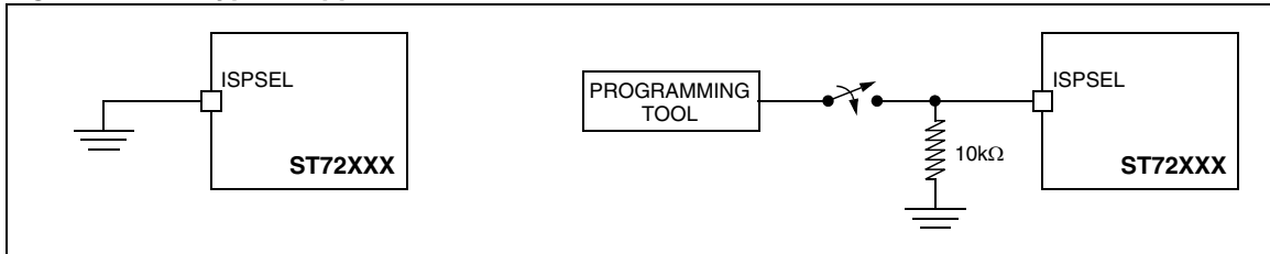
Figure 89. Two typical Applications with ISPSEL Pin 2)
