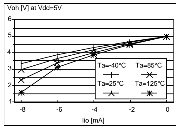
Figure 81. Typical V_{OH} at V_{DD}=5V
