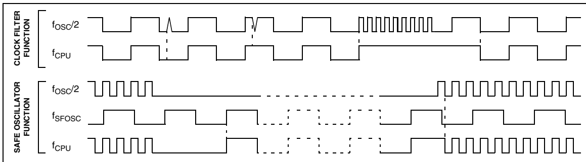
Figure 12. Clock Filter Function and Safe Oscillator Function
