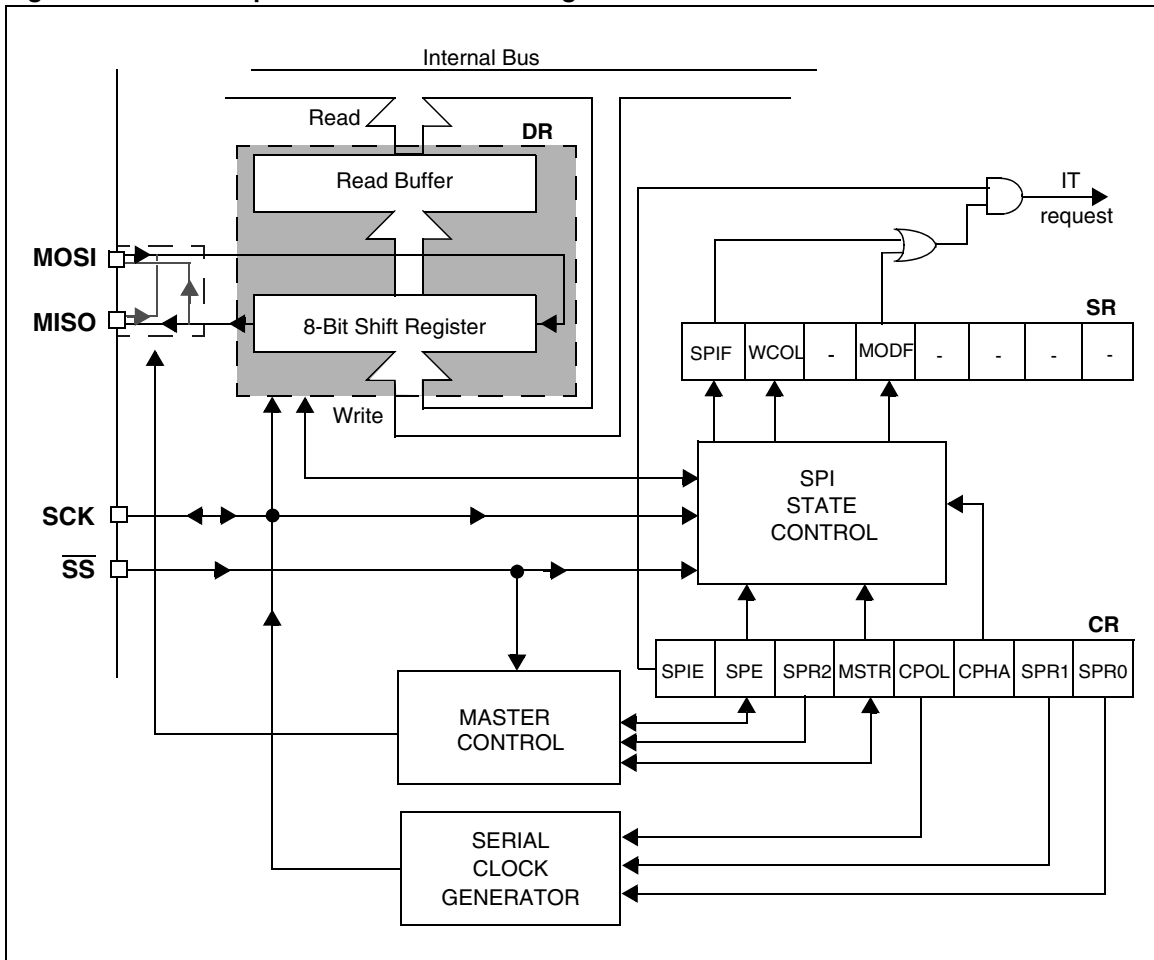
Figure 37. Serial Peripheral Interface Block Diagram
