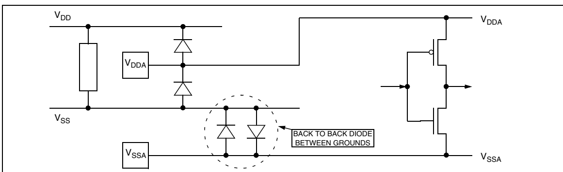
Figure 76. Multisupply Configuration
