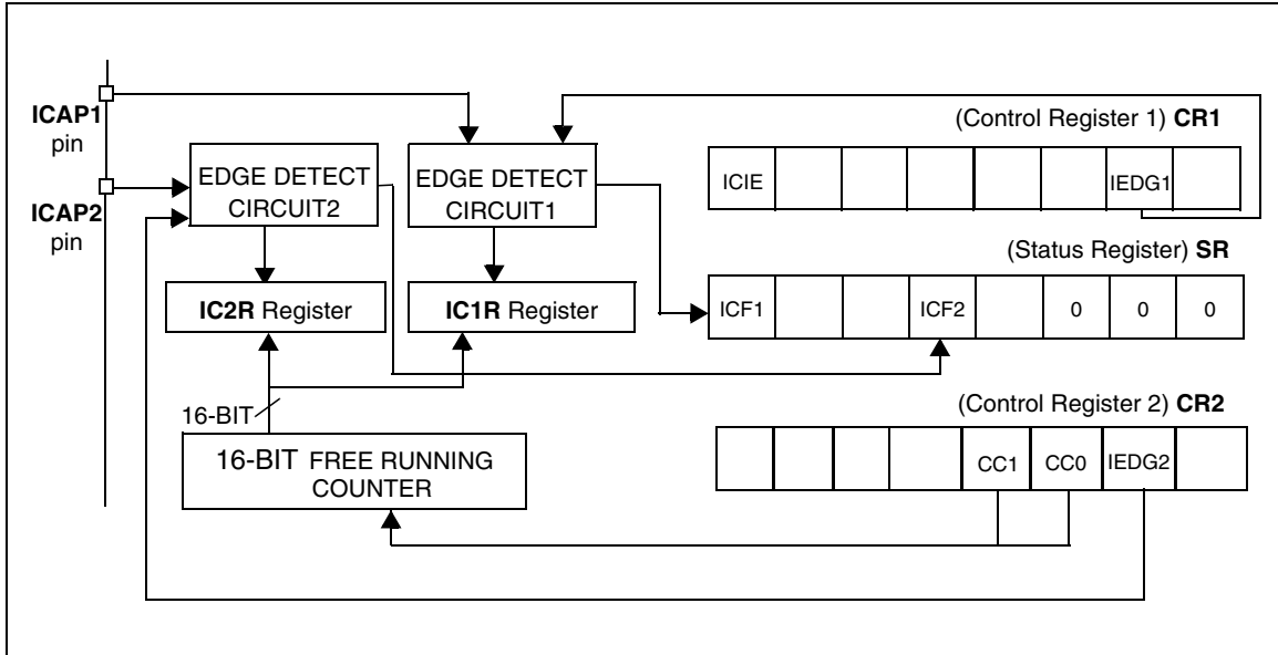
Figure 29. Input Capture Block Diagram
