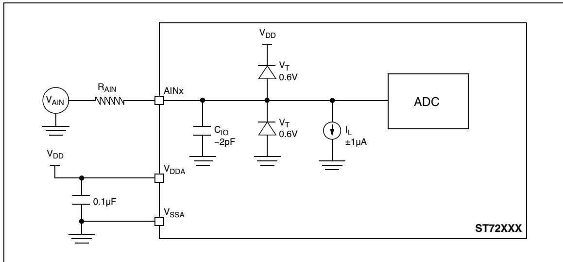
Figure 94. Typical Application with ADC
