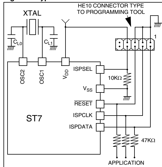
Figure 4. Typical Remote ISP Interface
