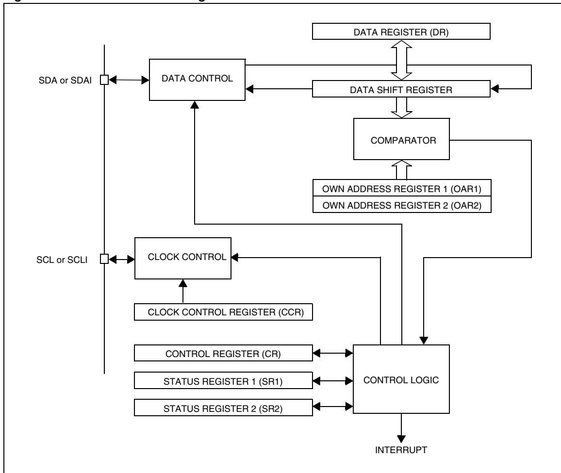
Figure 43. I 2 C Interface Block Diagram
