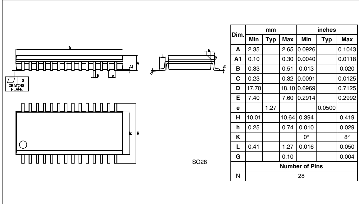
Figure 96. 28-Pin Plastic Small Outline Package, 300-mil Width
