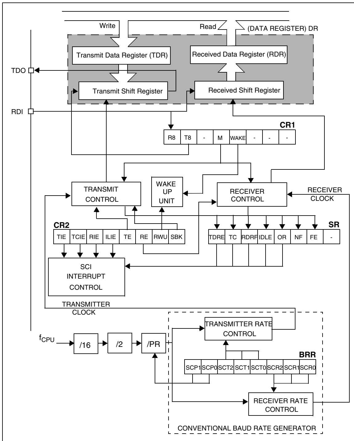
Figure 47. SCI Block Diagram
