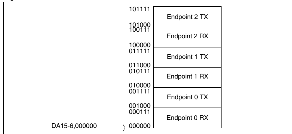
Figure 45. DMA buffers
