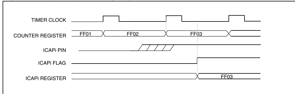
Figure 33. Input Capture timing diagram
