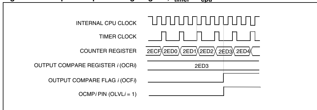
Figure 36. Output Compare timing diagram, f_{timer} = f_{CPU}/4
