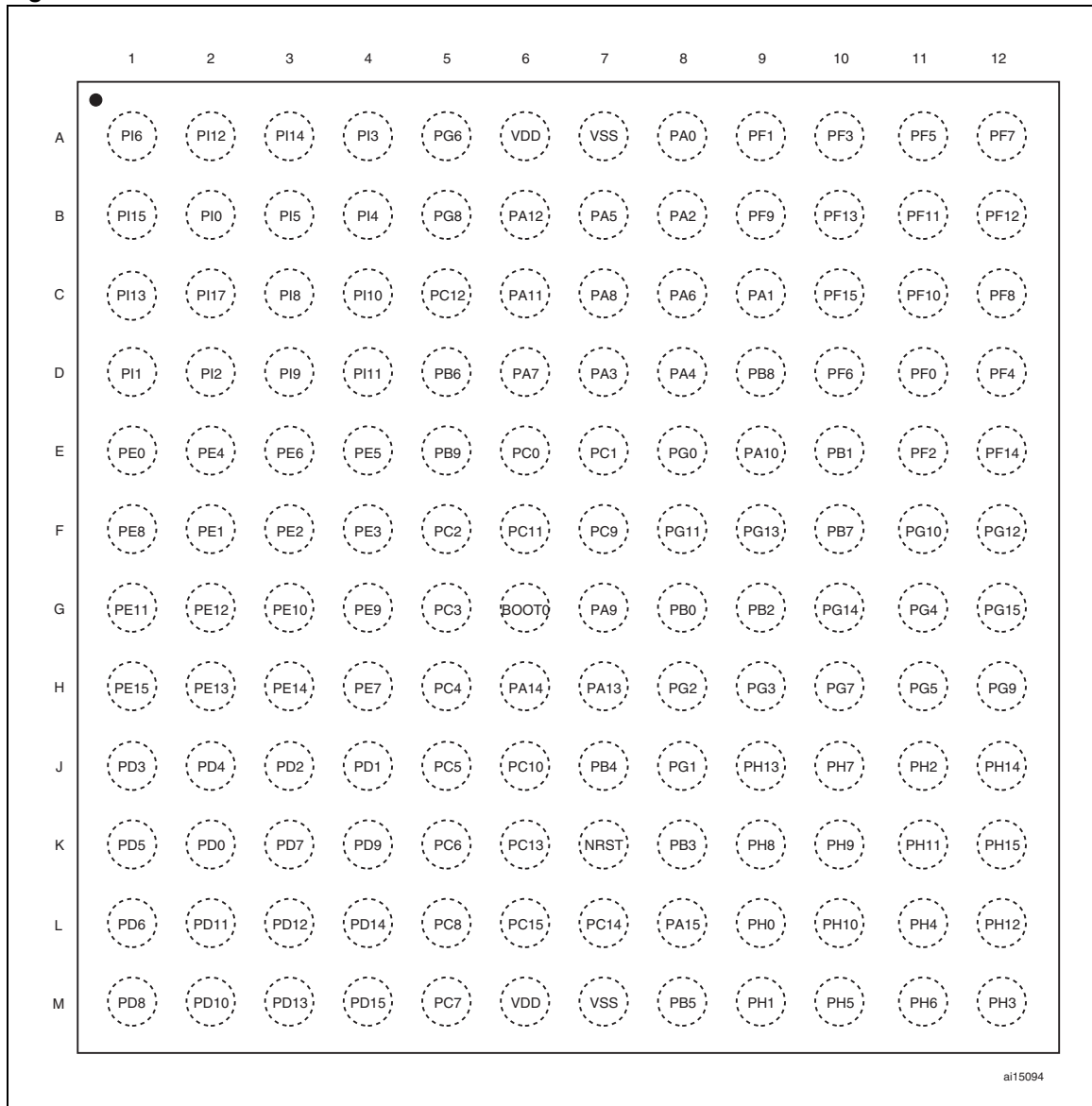
Figure 2. STM32TS60 device UFBGA144 ballout
