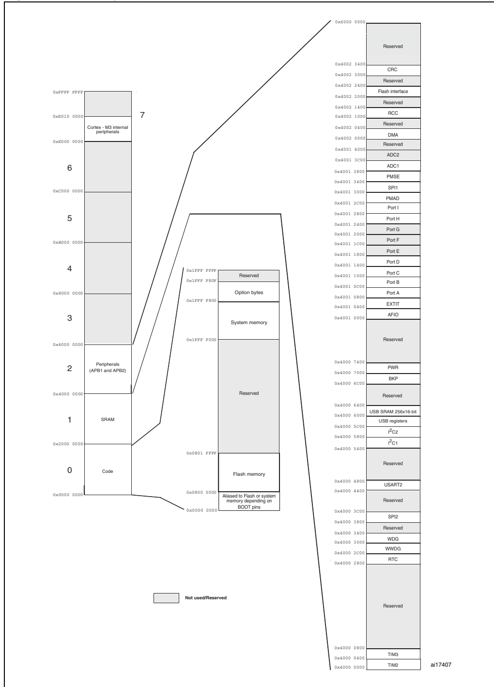
Figure 3. Memory map
