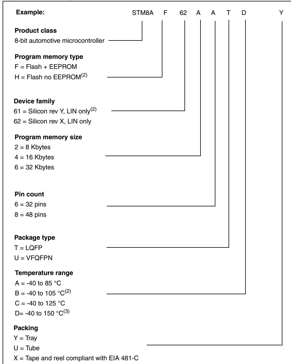
Figure 45. Ordering information scheme
