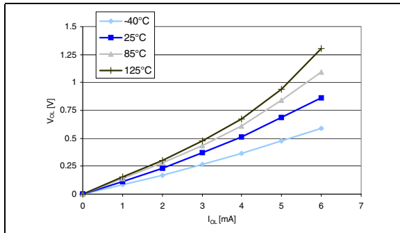
Figure 23. Typ. V_{OL} @ V_{DD} = 3.3 V (standard ports)
