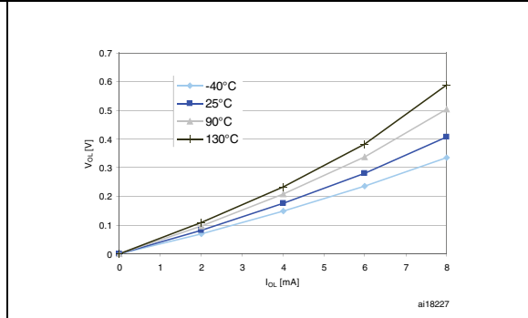
Figure 25. Typ. V_{OL} @ V_{DD} = 1.8\text{ V} (high sink ports)
