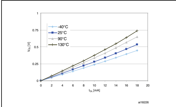
Figure 24. Typ. V_{OL} @ V_{DD} = 3.0\text{ V} (high sink ports)
