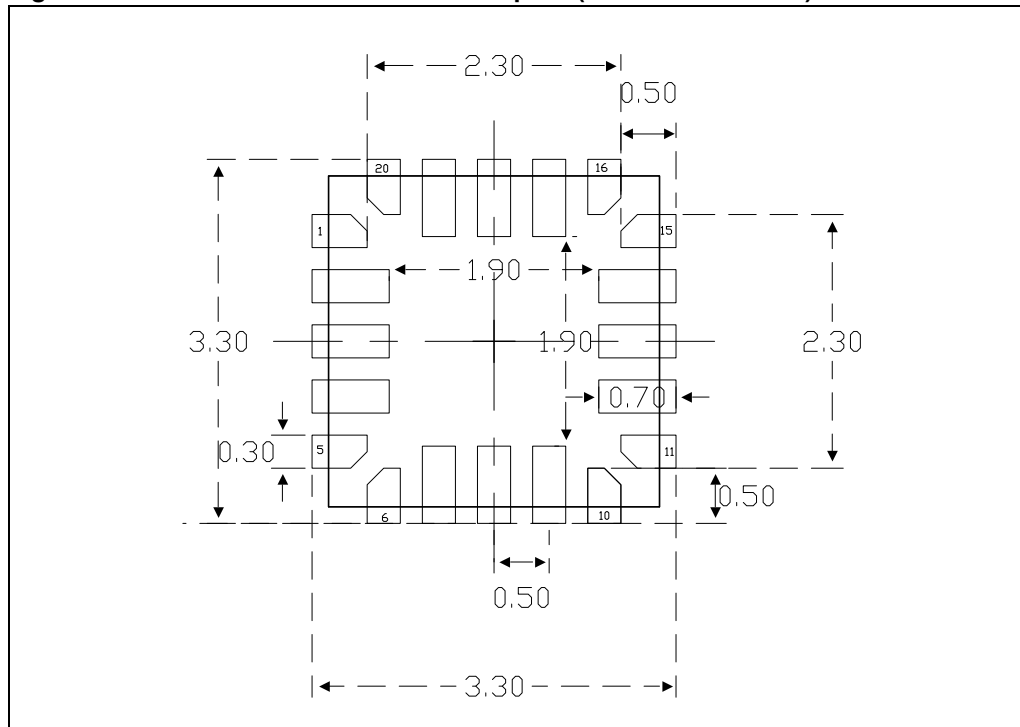
Figure 48. UFQFPN20 recommended footprint (dimensions in mm)
