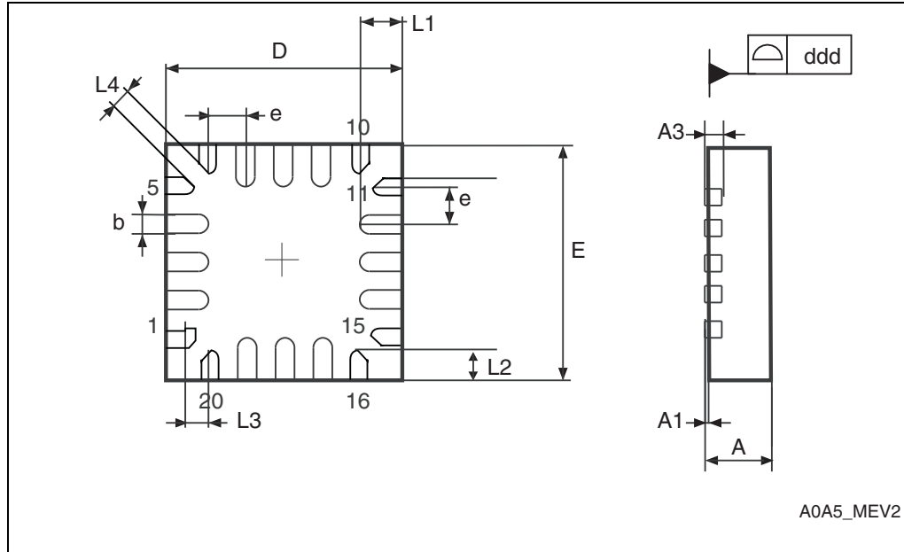
Figure 47. UFQFPN20 - 20-lead ultra thin fine pitch quad flat package outline (3x3)
