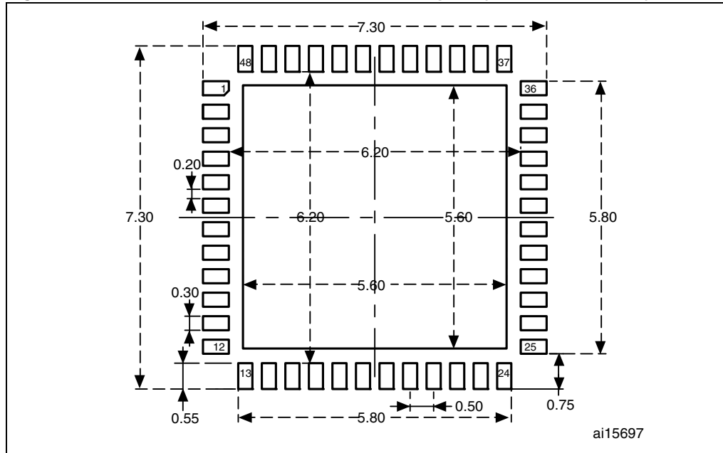
Figure 61. UFQFPN48 7x7 mm recommended footprint (dimensions in mm)
