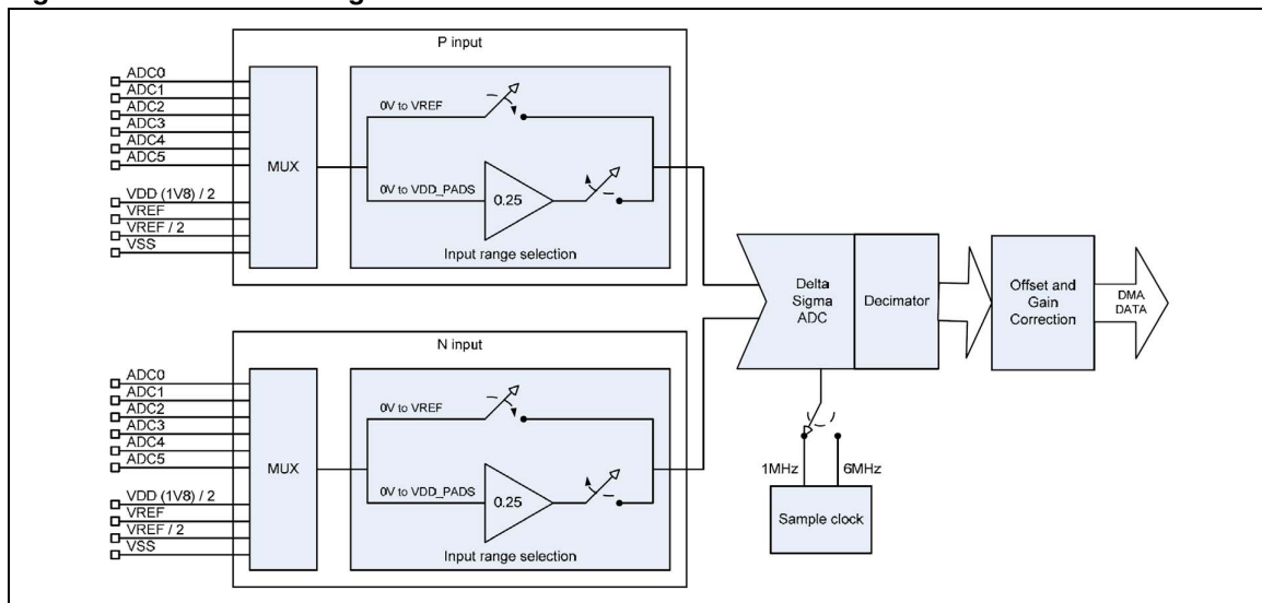
Figure 51. ADC block diagram
