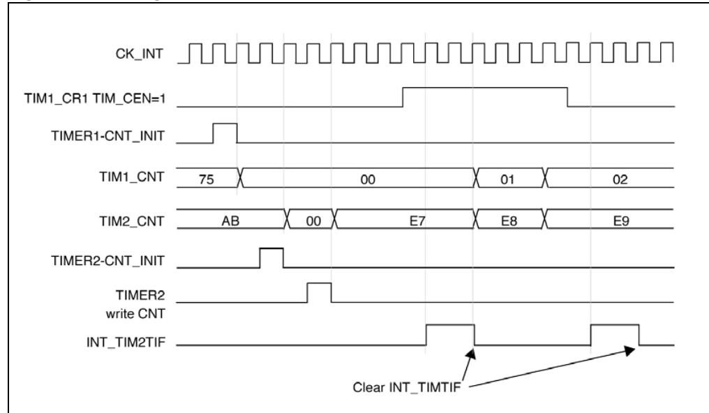
Figure 47. Gating Timer 2 with enable of Timer 1
