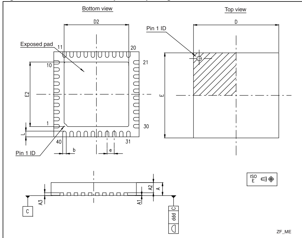
Figure 59. VFQFPN40 6x6mm pitch 0.5 package outline
