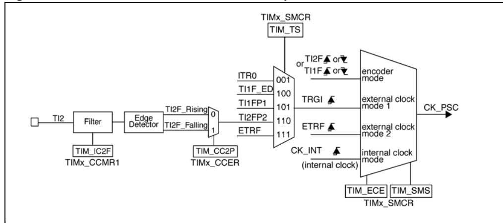
Figure 27. TIM2 external clock connection example
