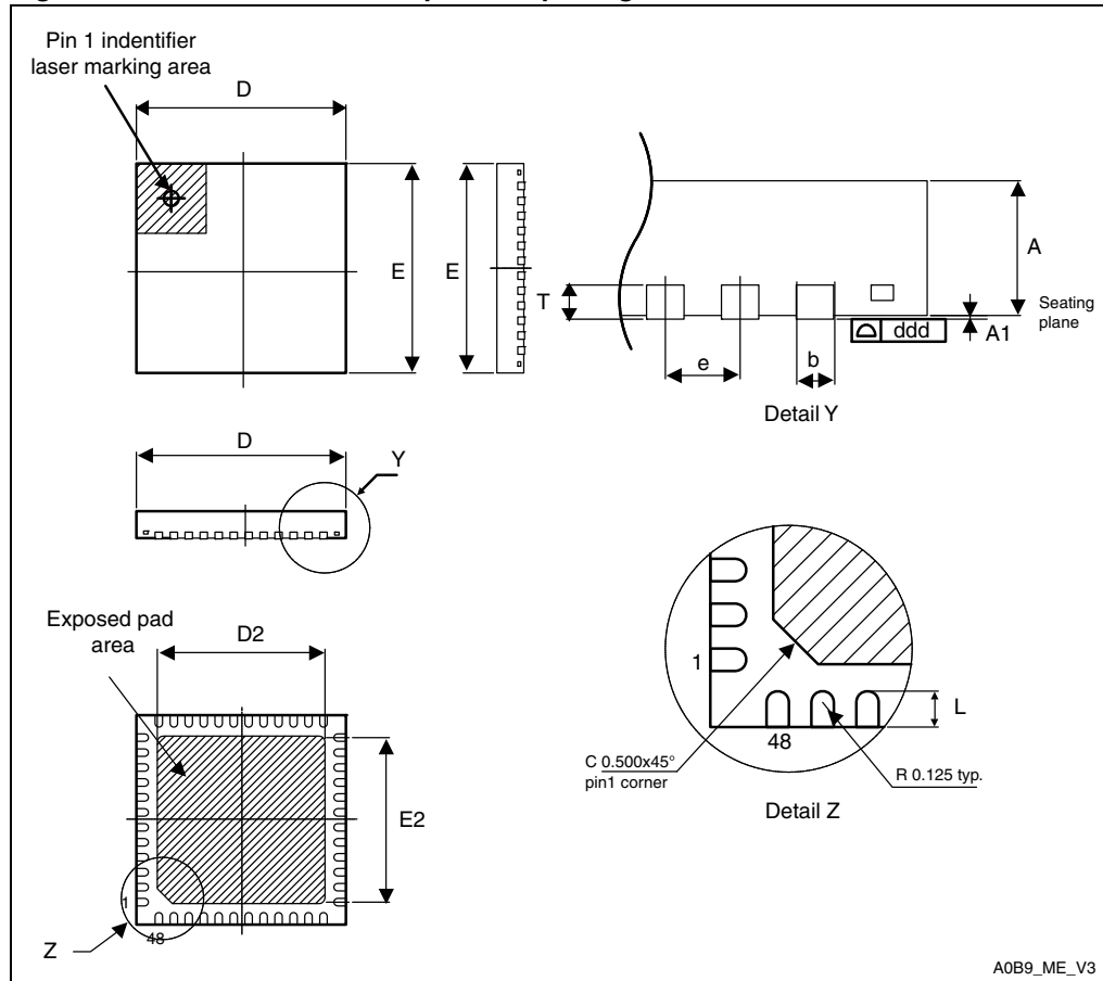
Figure 60. UFQFPN48 7x7 mm pitch 0.5 package outline
