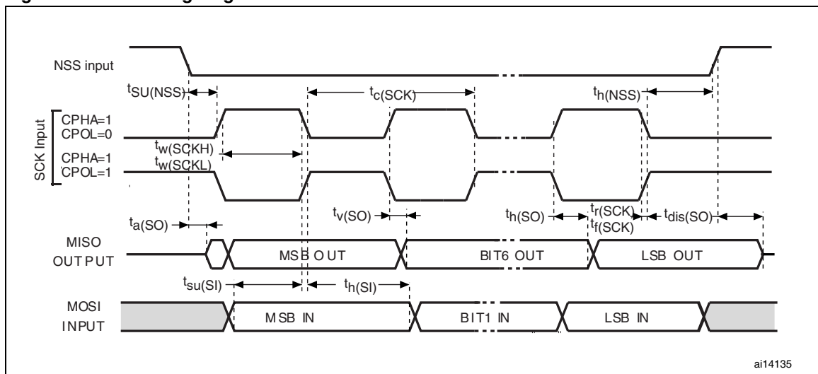
Figure 31. SPI timing diagram - slave mode and CPHA = 1
