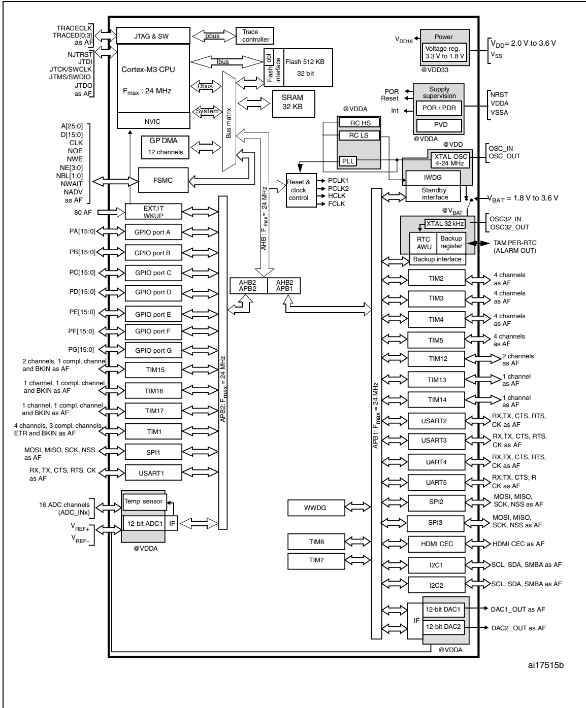
Figure 1. STM32F100xx value line block diagram
