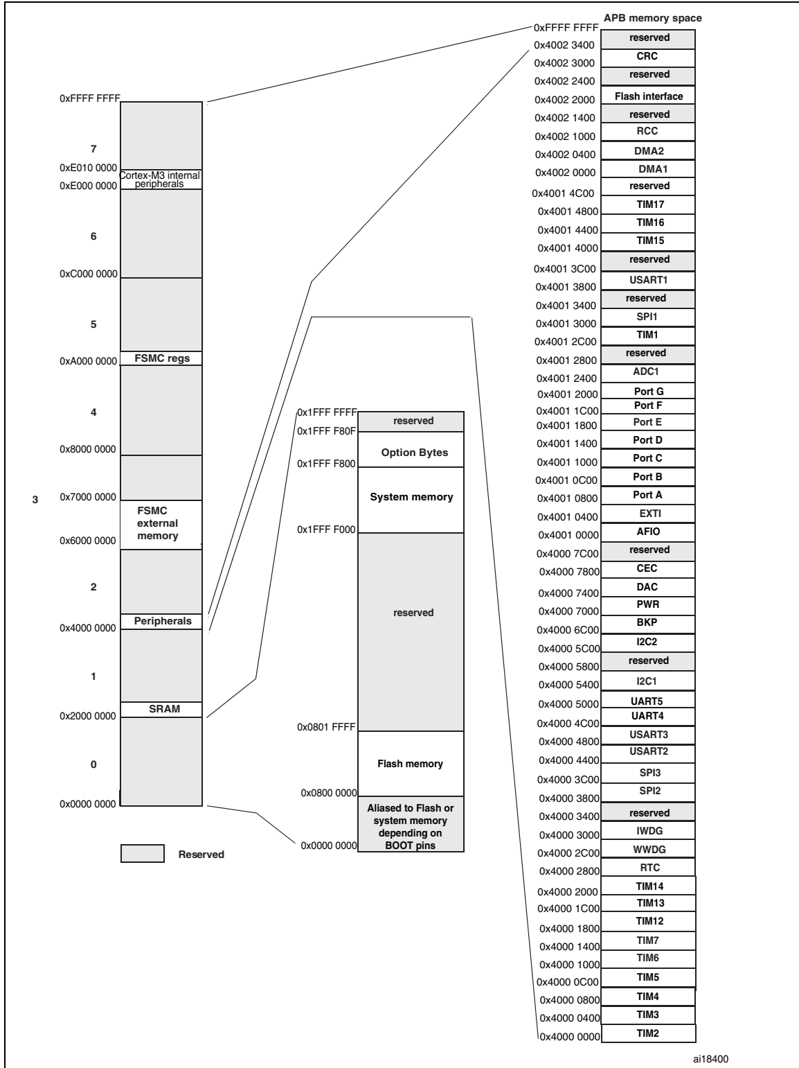
Figure 6. Memory map
