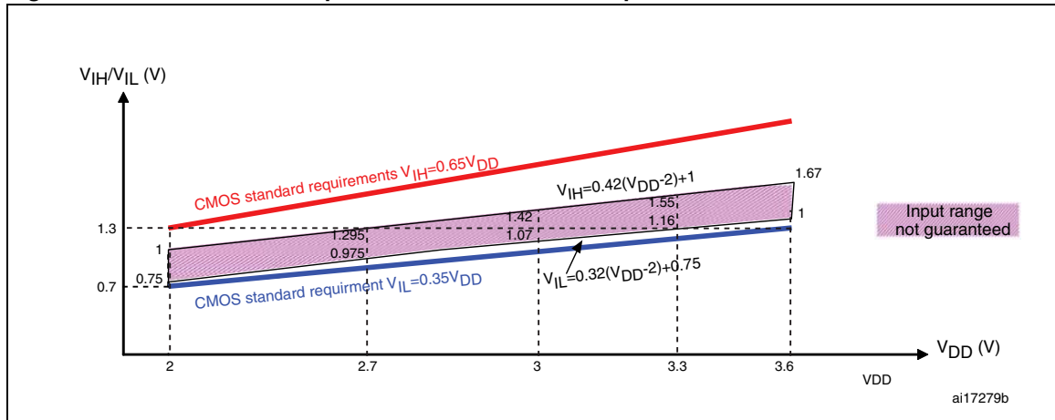
Figure 25. 5 V tolerant I/O input characteristics - CMOS port
