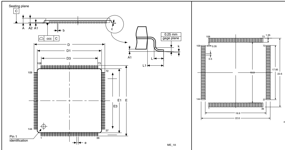
Figure 38. LQFP144, 20 x 20 mm, 144-pin thin quad flat package outline
