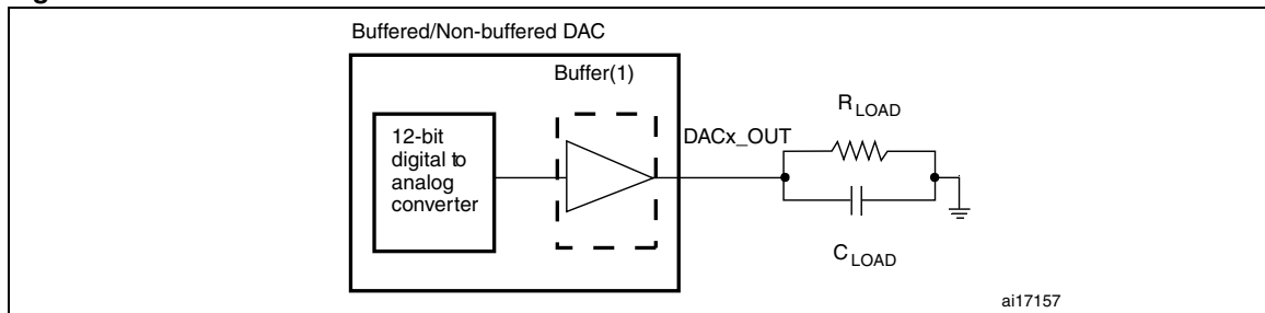
Figure 37. 12-bit buffered /non-buffered DAC
