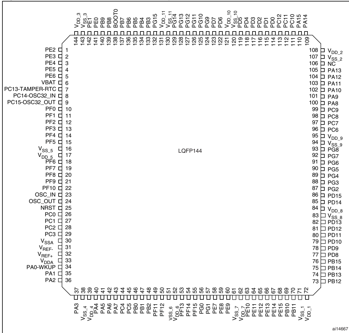
Figure 3. STM32F100xx value line LQFP144 pinout
