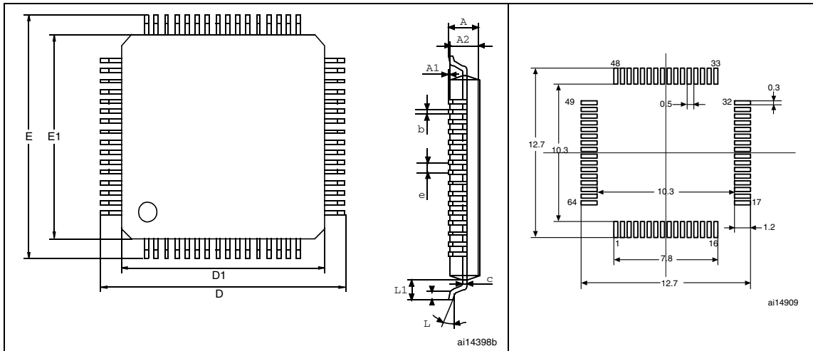
Figure 42. LQFP64 – 10 x 10 mm, 64 pin low-profile quad flat package outline
