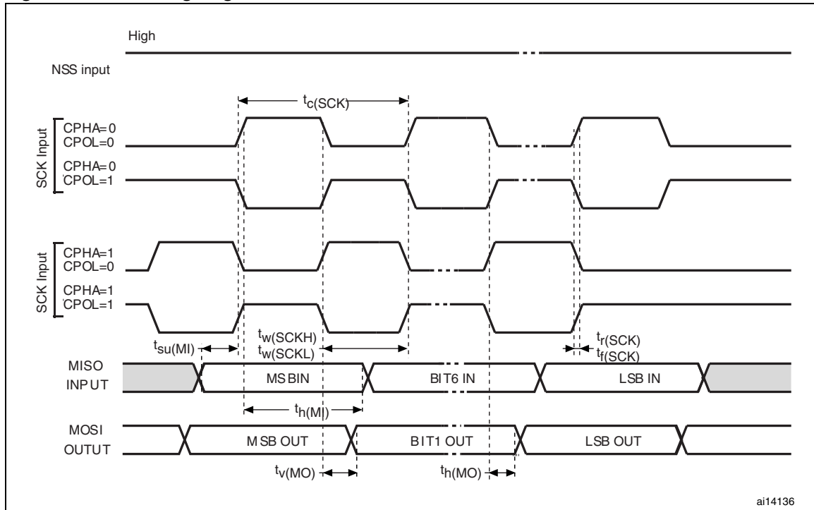
Figure 32. SPI timing diagram - master mode
