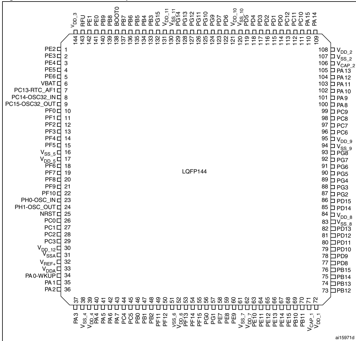
Figure 11. STM32F21x LQFP144 pinout
