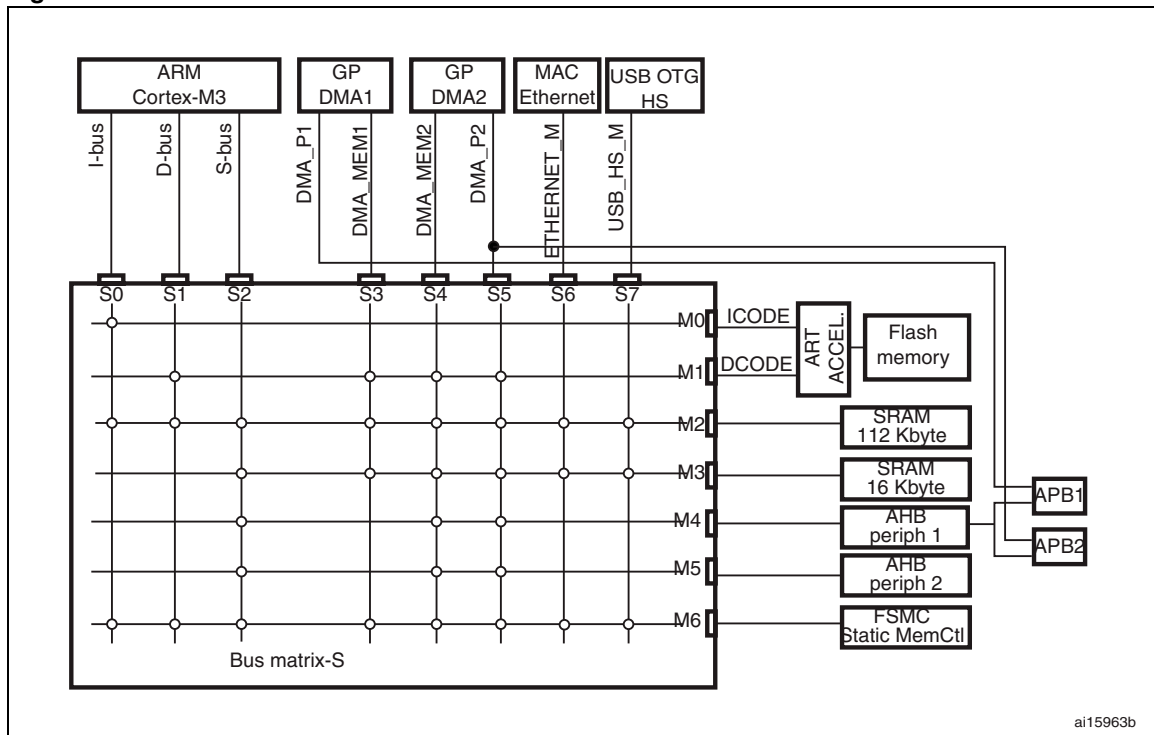
Figure 6. Multi-AHB matrix
