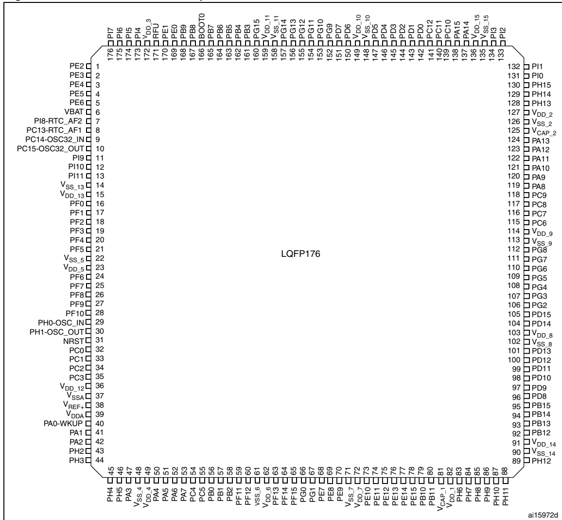
Figure 12. STM32F21x LQFP176 pinout
