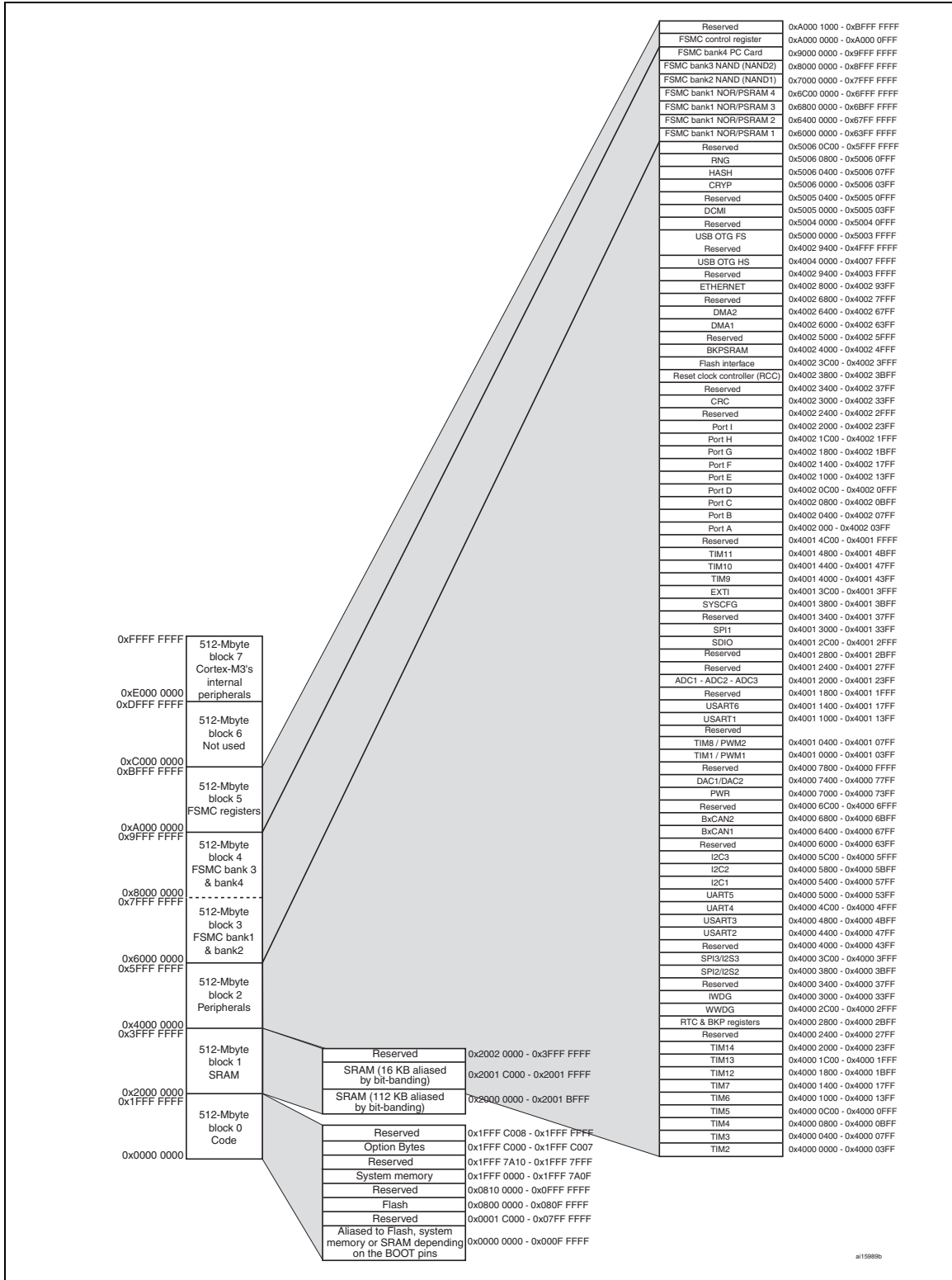
Figure 14. Memory map
