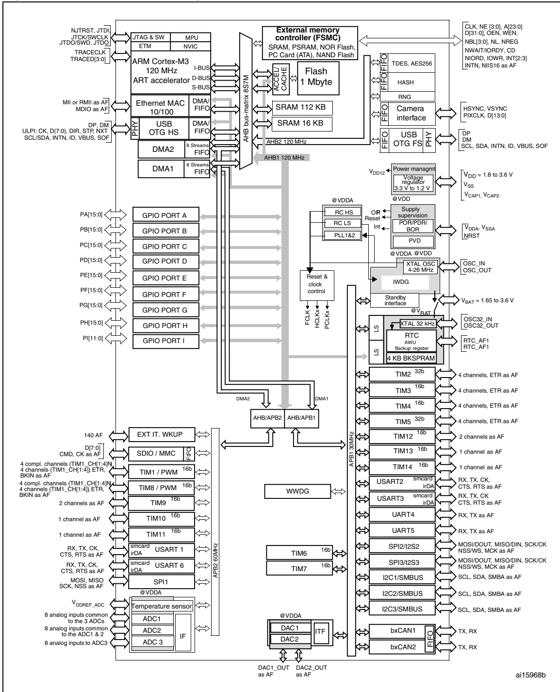
Figure 5. STM32F21x block diagram
