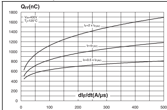
Figure 7. Reverse recovery charges versus di_F/dt (90 % confidence)
