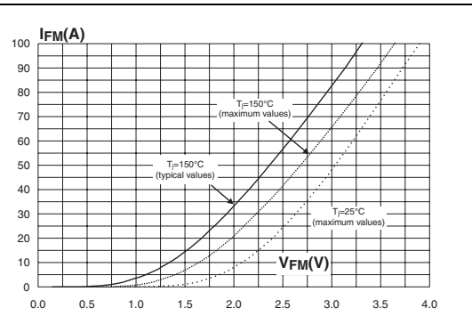
Figure 2. Forward voltage drop versus forward current
