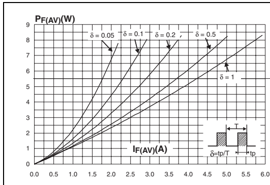
Figure 1. Conduction losses versus average current
