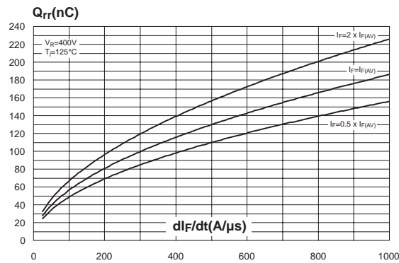
Fig. 6: Reverse recovery charges versus di_F/dt (typical values).
