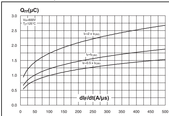
Figure 7. Reverse recovery charges versus di_F/dt (typical values)
