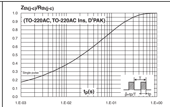
Figure 4. Relative variation of thermal impedance junction to case versus pulse duration (TO-220AC, TO-220AC Ins, D²PAK)
