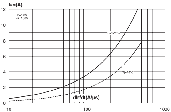
Fig. 10: Reverse recovery current versus di_F/dt (90% confidence, per diode).
