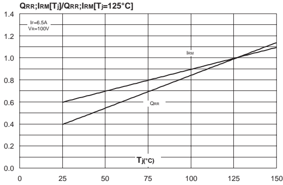
Fig. 11: Dynamic parameters versus junction temperature.
