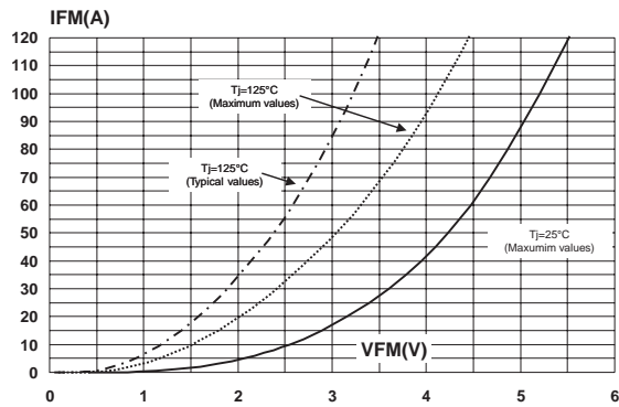
Fig. 2: Forward voltage drop versus forward current (per leg).
