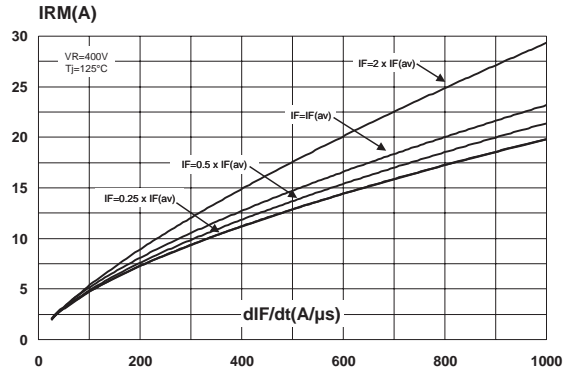
Fig. 4: Peak reverse recovery current versus di_F/dt (90% confidence, per leg).
