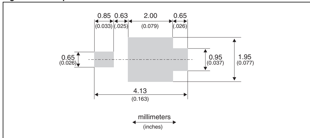
Figure 22. Footprint dimensions
