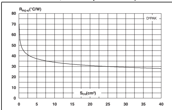
Figure 11. Thermal resistance junction to ambient versus copper surface under tab (epoxy printed board FR4, Cu = 35 µm - D 2 PAK)
