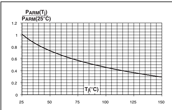
Figure 9. Normalized avalanche power derating versus junction temperature
