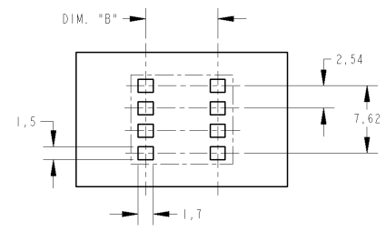
RECOMMENDED PCB LAYOUT SCALE 5:2
