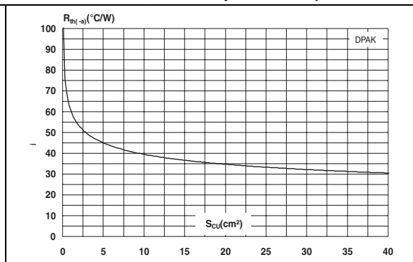
Figure 10. Thermal resistance junction to ambient versus copper surface area under tab (epoxy printed board FR4, Cu = 35 μm - DPAK)
