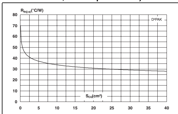
Figure 11. Thermal resistance junction to ambient versus copper surface area under tab (epoxy printed board FR4, Cu = 35 μm - D 2 PAK)
