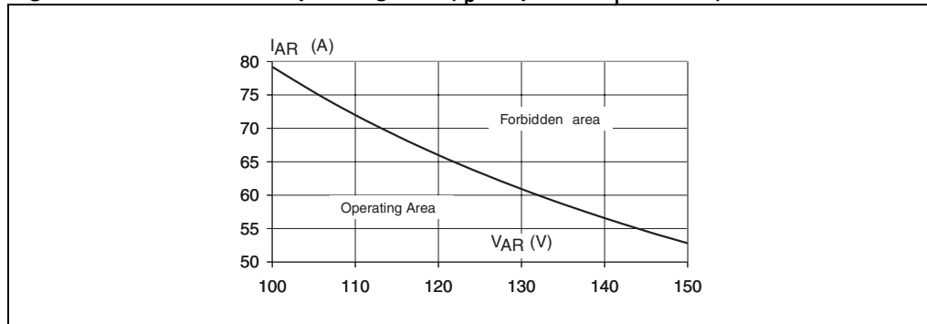
Figure 14. Reverse safe operating area ( t_p < 1 \mu\text{s} and T_j < 150 \text{ }^\circ\text{C} )
