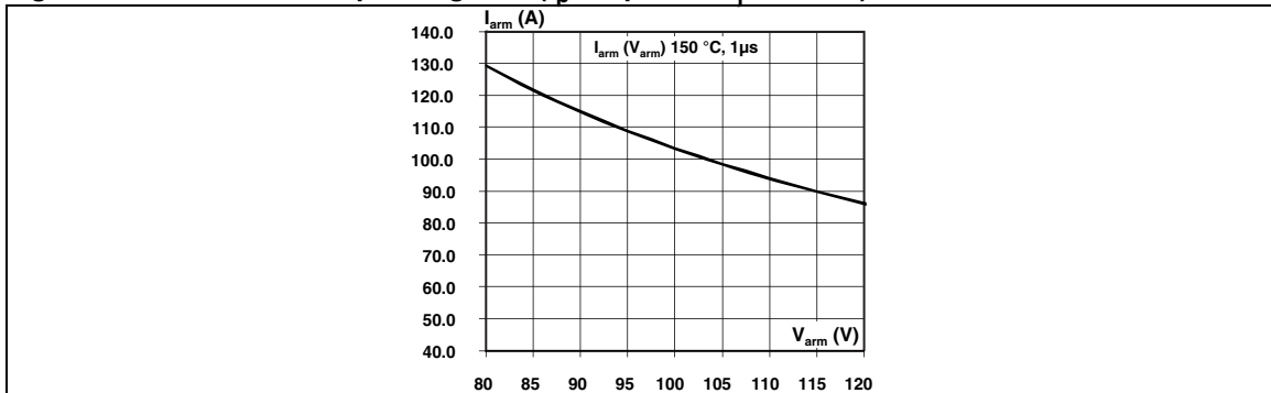
Figure 12. Reverse safe operating area ( t_p < 1 \mu\text{s} and T_j < 150 \text{ °C} )
