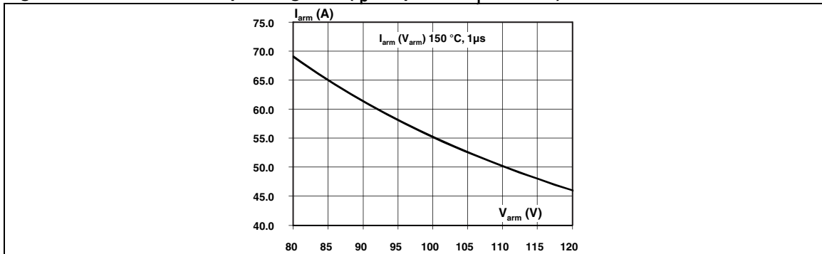
Figure 12. Reverse safe operating area ( t_p < 1 \mu s and T_j < 150 °C)
