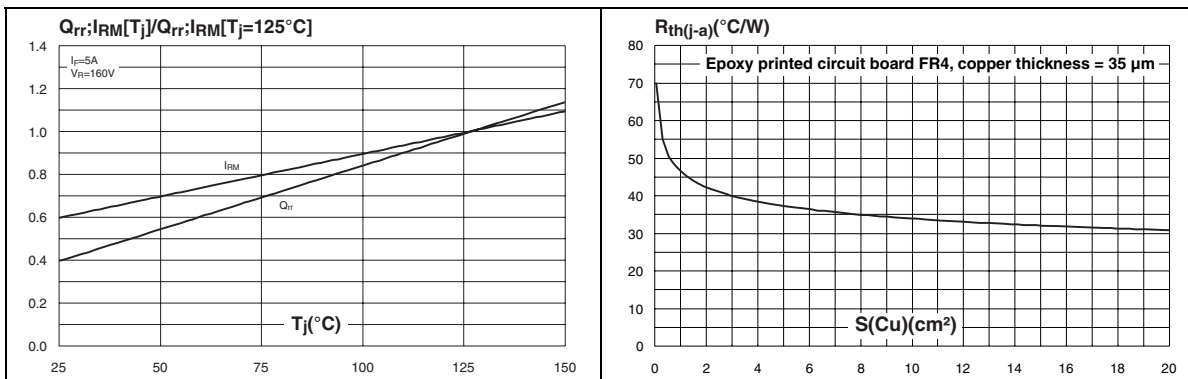
Figure 11. Thermal resistance junction to ambient versus copper surface under tab (Epoxy printed circuit board FR4, copper thickness = 35 \mu\text{m} ) for DPAK
