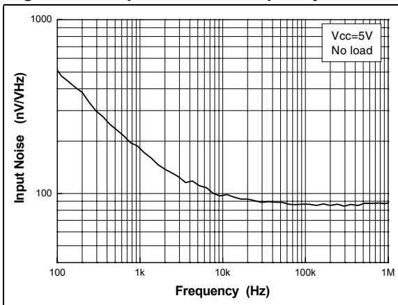
Figure 5. Input noise vs. frequency
