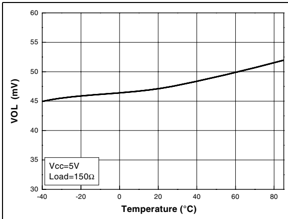
Figure 19. VOL vs. temperature
