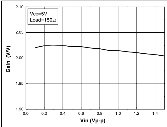
Figure 7. Gain vs. input amplitude
