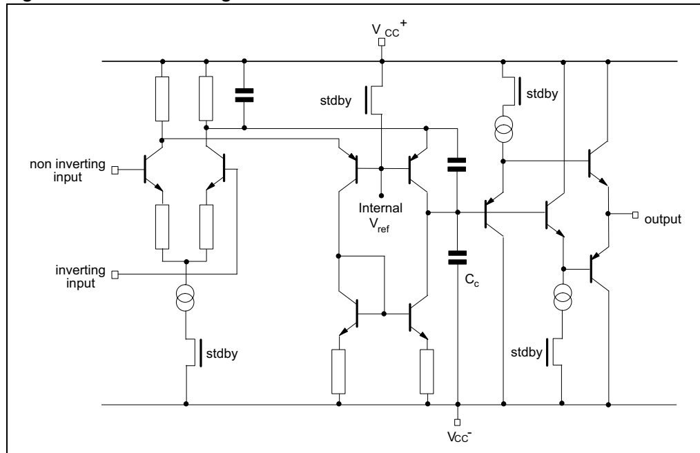
Figure 1. Schematic diagram
