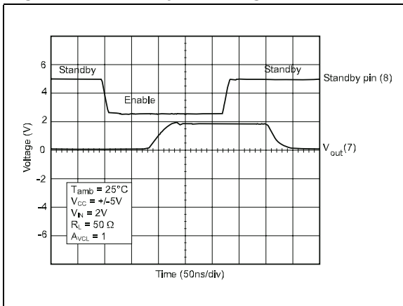
Figure 13. Standby switching
