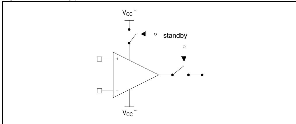
Figure 2. Standby position
