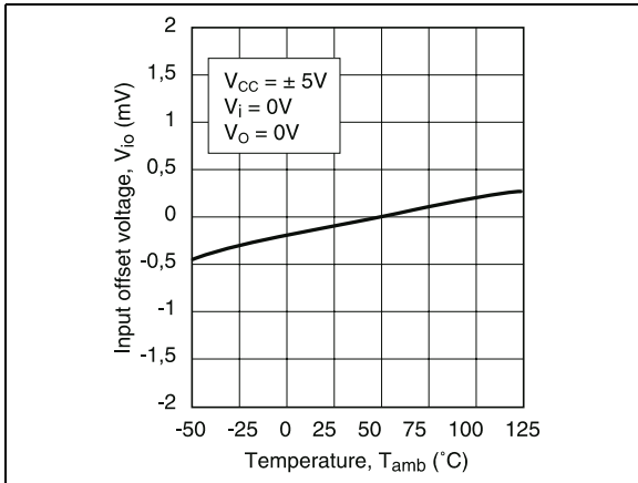
Figure 17. Input offset voltage drift versus temperature
