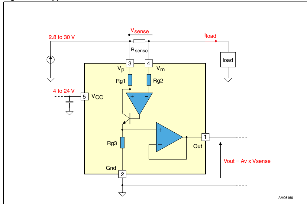
Figure 1. Application schematics
