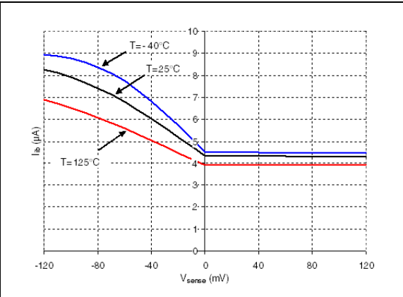
Figure 5. V_m pin input bias current vs. V_{sense}
