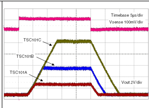
Figure 19. Step response
