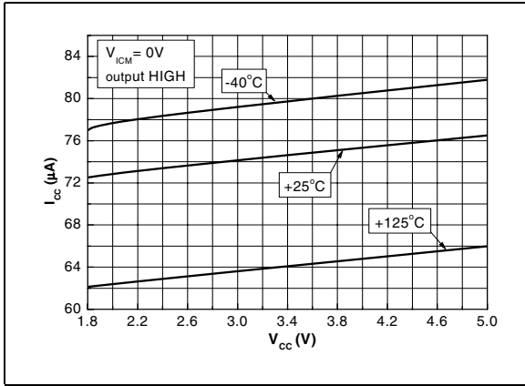
Figure 3. Current consumption /comp. vs. power supply voltage
