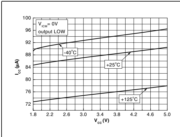
Figure 3. Current consumption /comp. vs. power supply voltage
