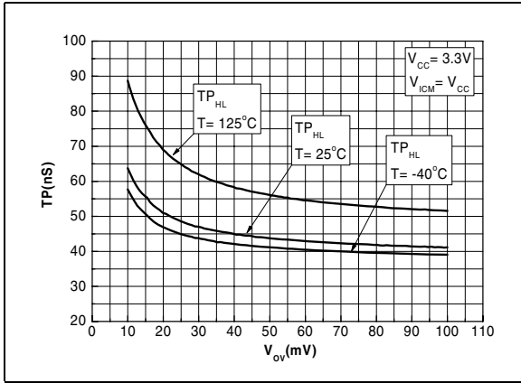
Figure 21. Propagation delay vs. overdrive V_{CC} = 3.3\text{ V}
